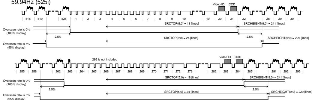
Figure 30.5 Example of Vertical Active Image Period (59.94 Hz (525i))
