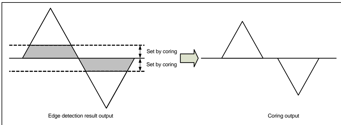
Figure 34.5 LTI Coring
