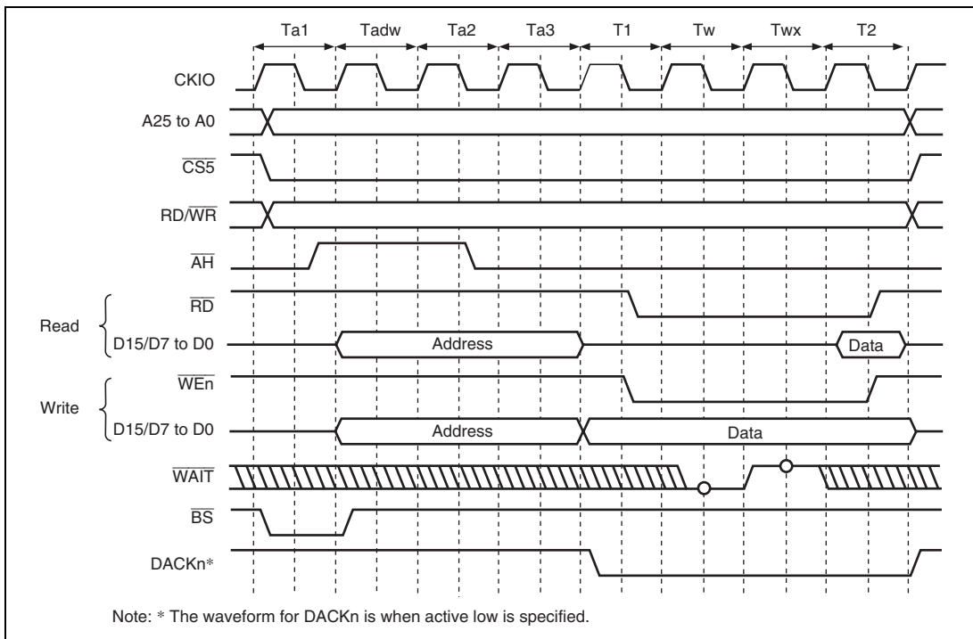
Figure 10.13 Access Timing for MPX Space (Address Cycle Access Wait 1, Data Cycle Wait 1, External Wait 1)
