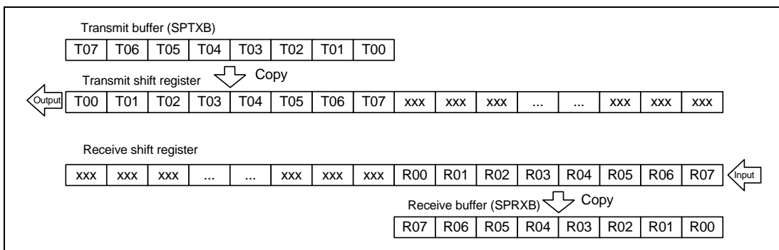
Figure 18.10 LSB First Transfer (8-Bit Data)
