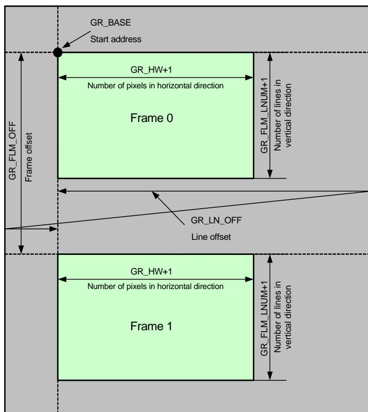
Figure 35.2 Data Arrangement in Frame Buffer
