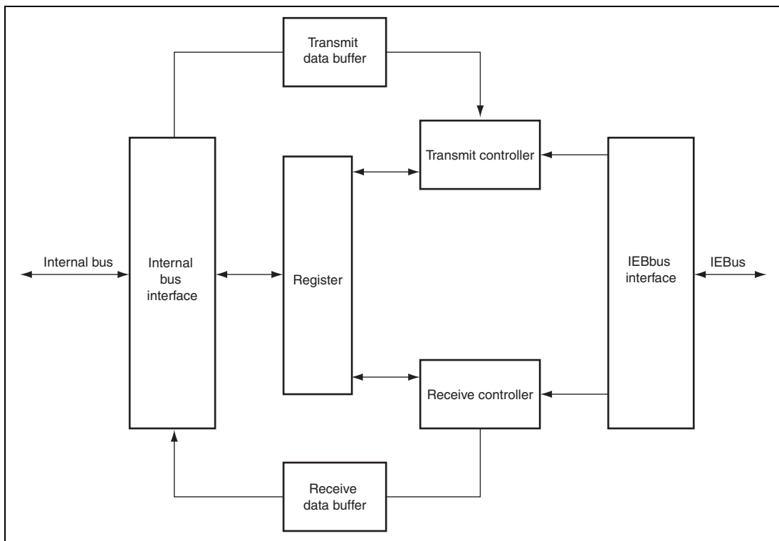
Figure 24.5 Block Diagram
