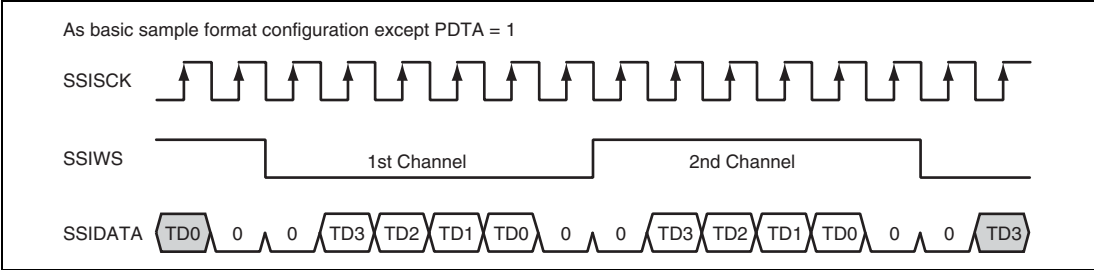
Figure 21.16 Parallel Right-Aligned with Delay
