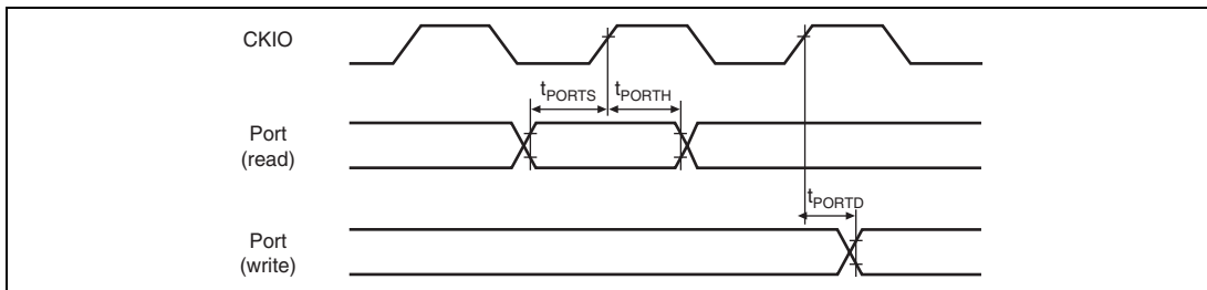
Figure 52.83 General I/O Ports Timing
