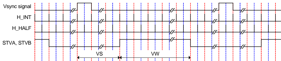
Figure 36.17 Vertical Panel Driver Signal (H_INT Reference Operation)
