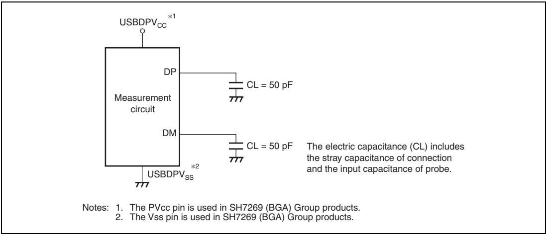
Figure 52.74 Measurement Circuit (Full-Speed)
