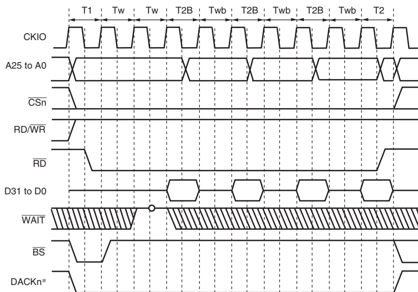
Figure 10.33 Burst ROM Access Timing (Clocked Asynchronous) (Bus Width = 32 Bits, 16-Byte Transfer (Number of Burst 4), Wait Cycles Inserted in First Access = 2, Wait Cycles Inserted in Second and Subsequent Access Cycles = 1)
