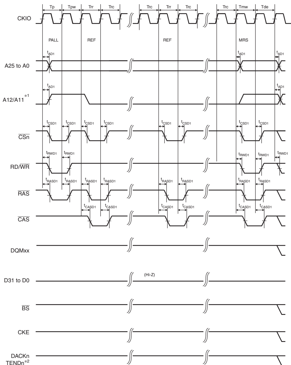
Figure 52.33 Synchronous DRAM Mode Register Write Timing (WTRP = 1 Cycle)
