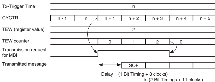
Figure 23.23 Timing Diagram of Timer
