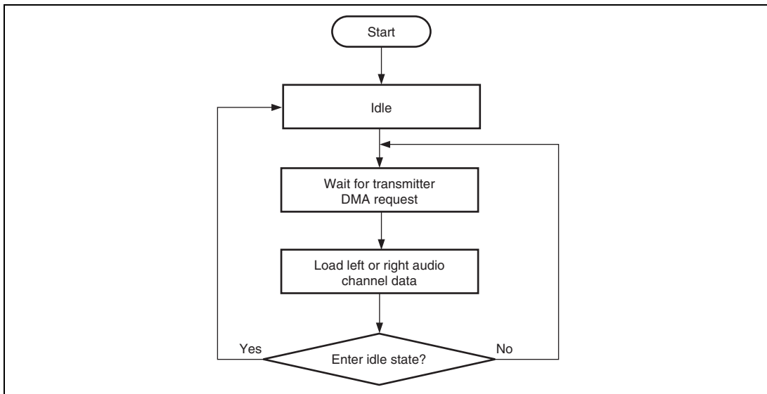
Figure 25.6 Transmitter Data Transfer Flow Diagram—DMA Request Driven
