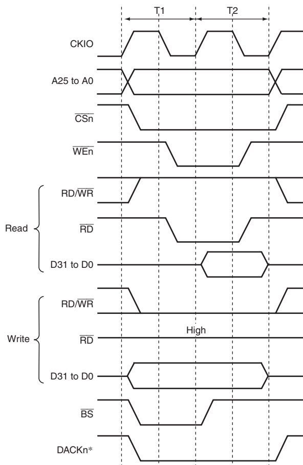
Figure 10.34 Basic Access Timing for SRAM with Byte Selection (BAS = 0)
