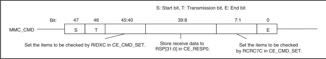
Figure 45.3 Format of 6-Byte Response
