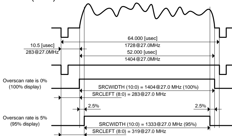
Figure 30.4 Example of Horizontal Active Image Period (50.00 Hz (625i))
