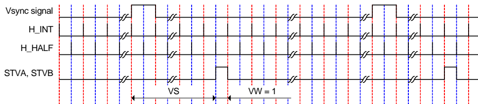
Figure 36.19 Vertical Panel Driver Signal (H_INT and H_HALF Reference Operation)
