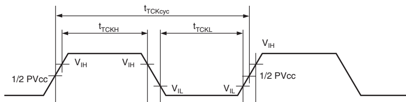
Figure 52.84 TCK Input Timing
