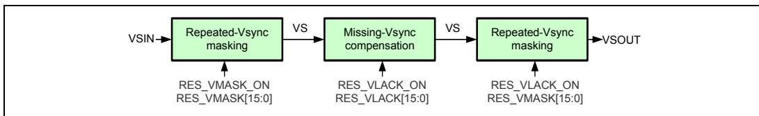
Figure 33.4 Repeated-Vsync Masking and Missing-Vsync Compensation
