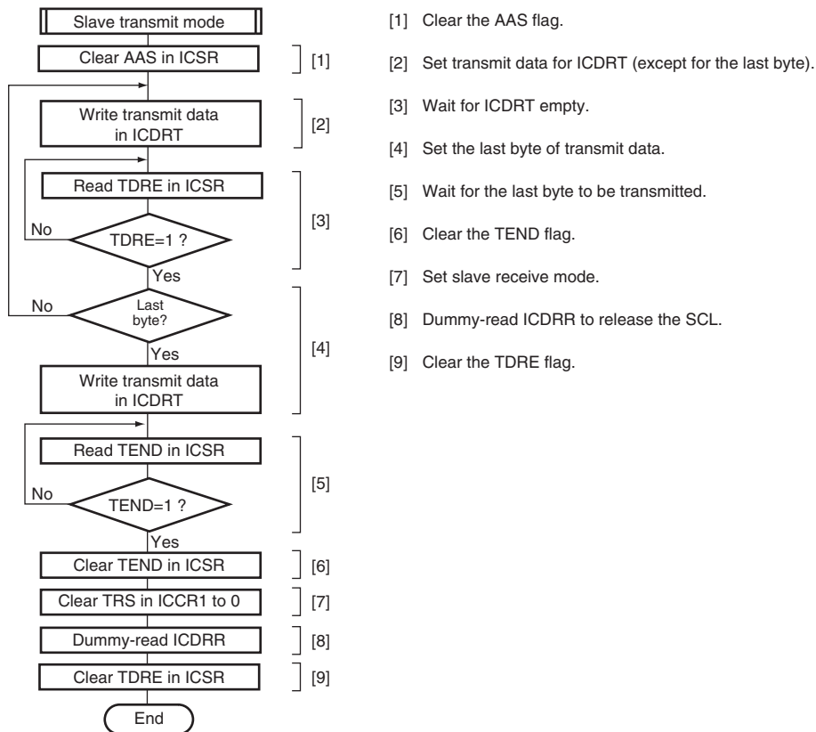
Figure 20.20 Sample Flowchart for Slave Transmit Mode
