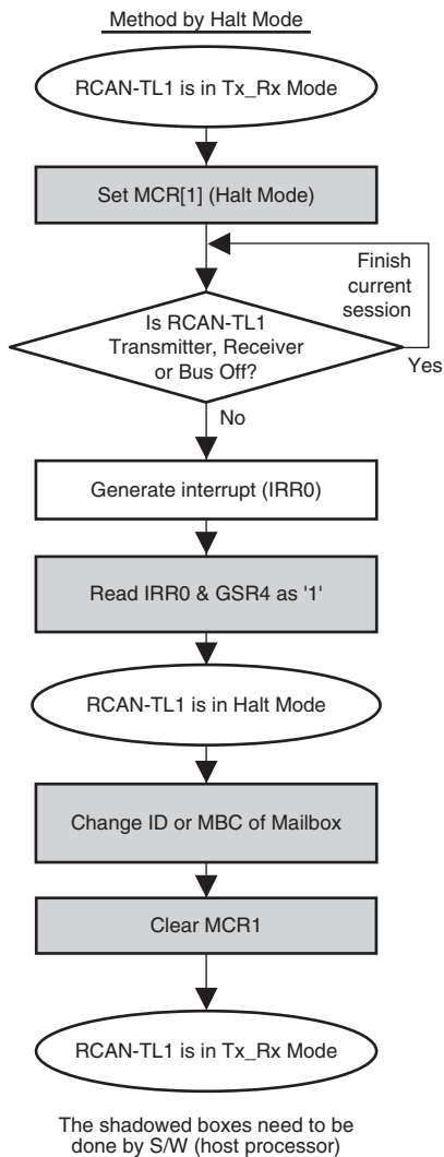
Figure 23.25 Change ID of receive box or Change receive box to transmit box
