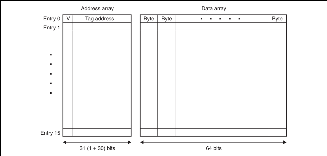
Figure 19.11 Read Cache Configuration
