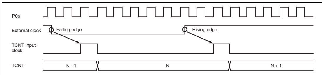
Figure 12.79 Count Timing in External Clock Operation
