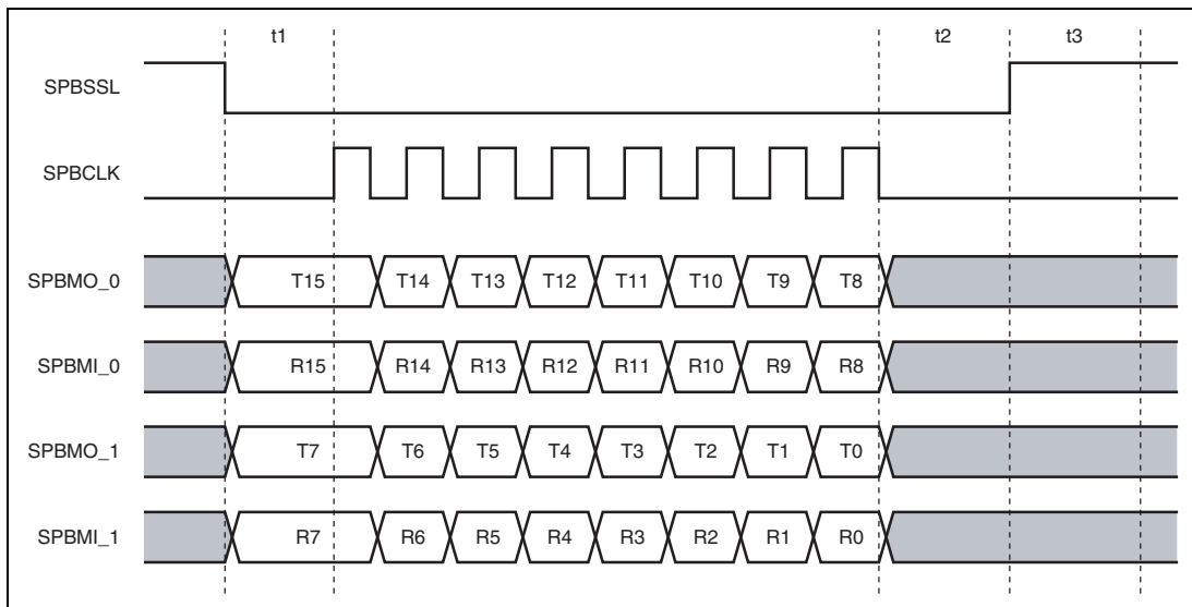
Figure 19.19 Transfer Format Example with 1-Bit Data Size and Two Serial Flash Memories Connected
