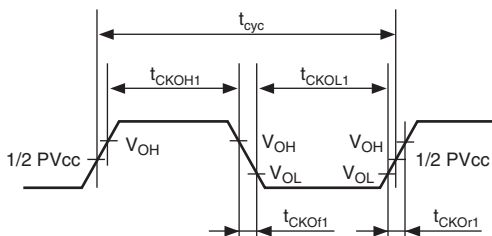
Figure 52.2 (1) CKIO Clock Output Timing 1
