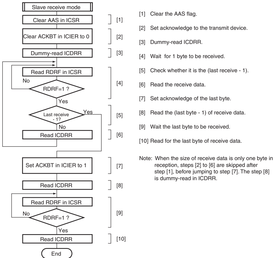
Figure 20.21 Sample Flowchart for Slave Receive Mode
