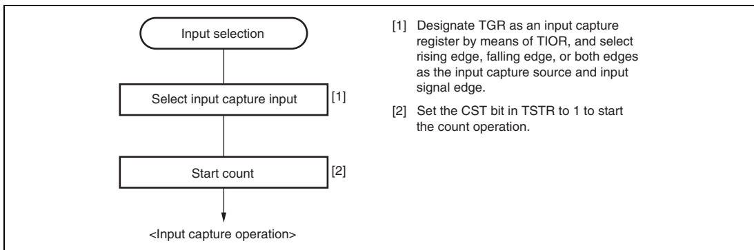
Figure 12.10 Example of Input Capture Operation Setting Procedure
