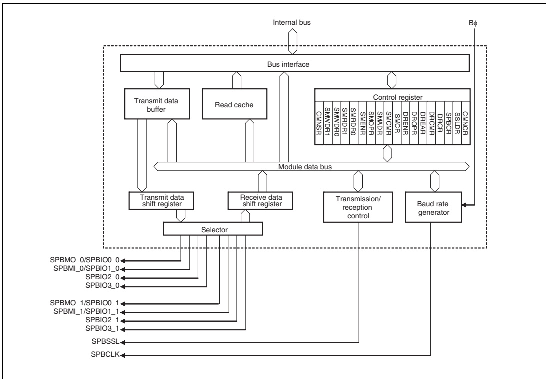
Figure 19.1 Block Diagram
