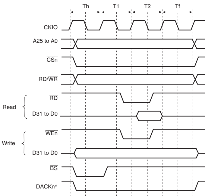
Figure 10.10 \overline{\text{CSn}} Assert Period Expansion
