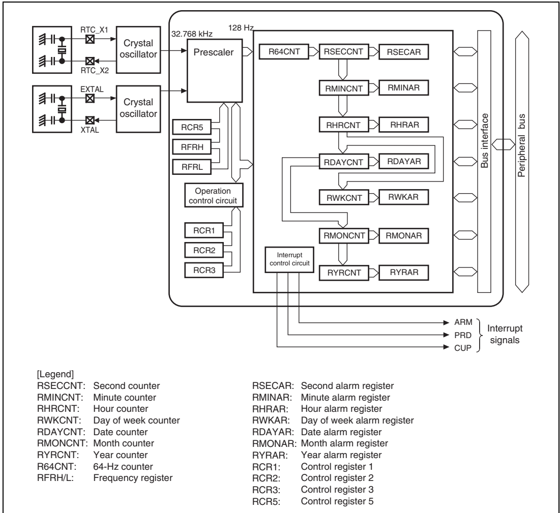
Figure 15.1 Block Diagram
