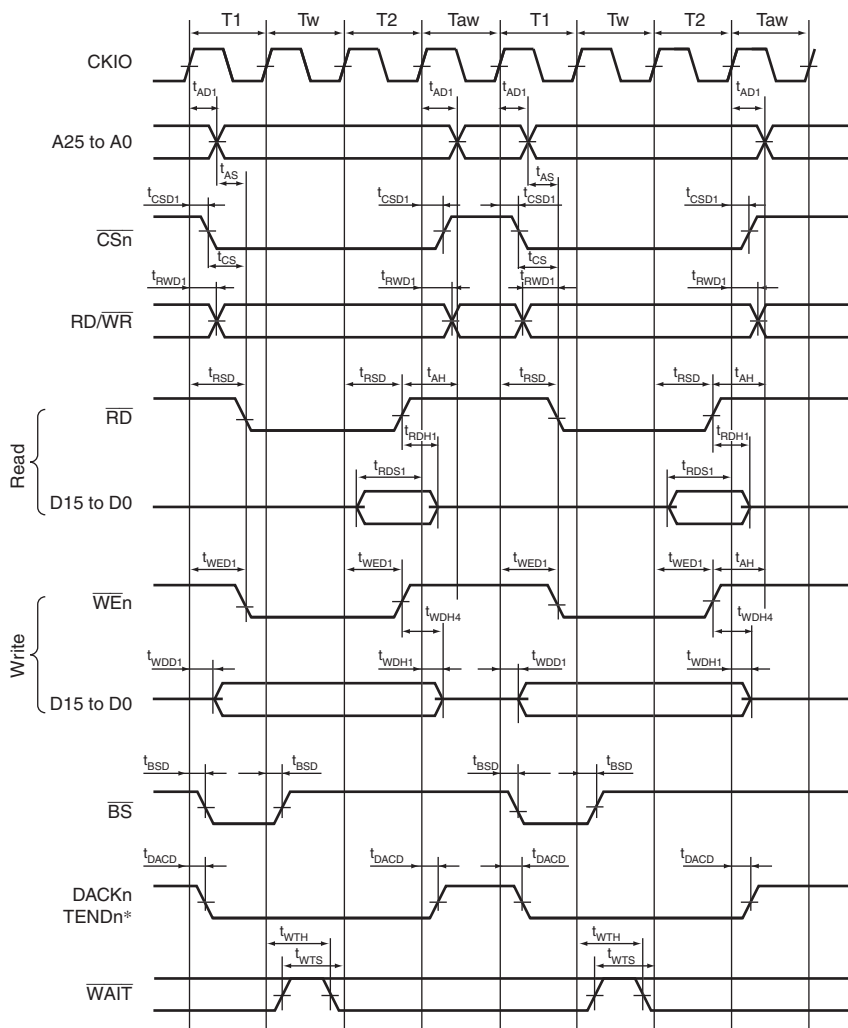
Figure 52.12 Basic Bus Timing for Normal Space (One Software Wait Cycle, External Wait Cycle Valid (WM Bit = 0), No Idle Cycle)
