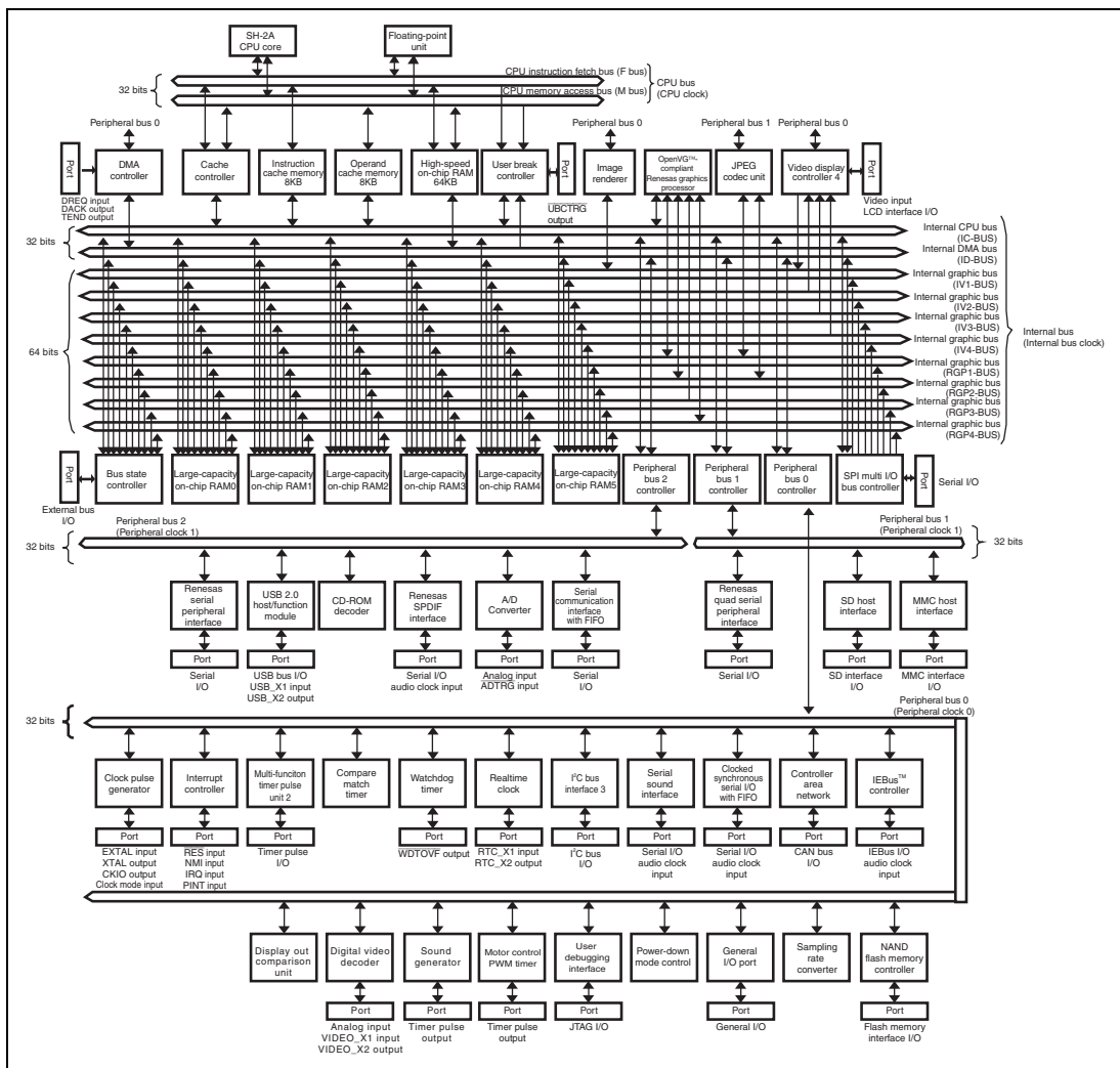
Figure 1.1 Block Diagram
