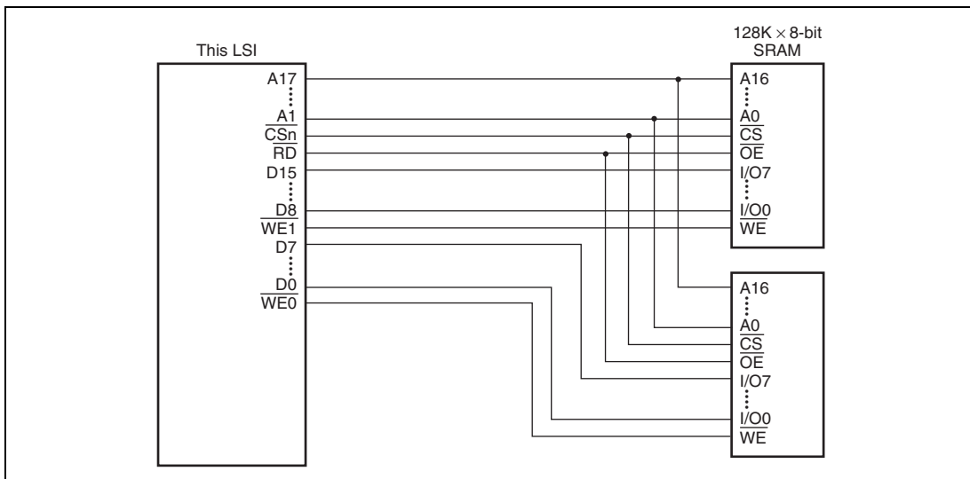
Figure 10.6 Example of 16-Bit Data-Width SRAM Connection
