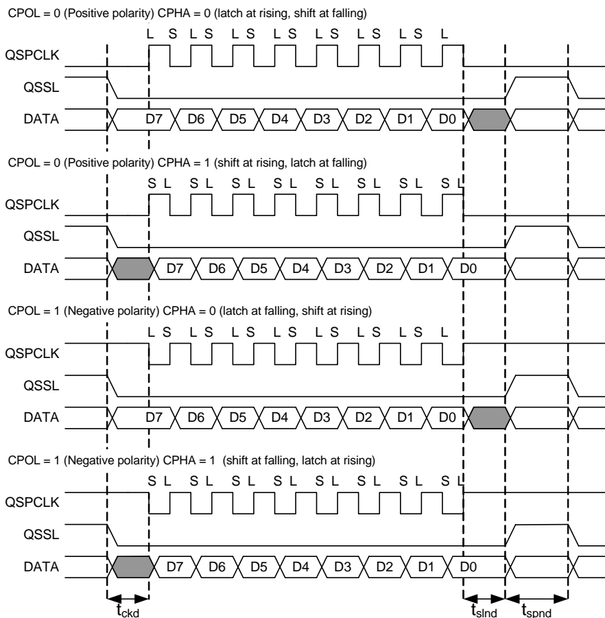
Figure 18.1 SPI Clock Setting and Transfer Timing
