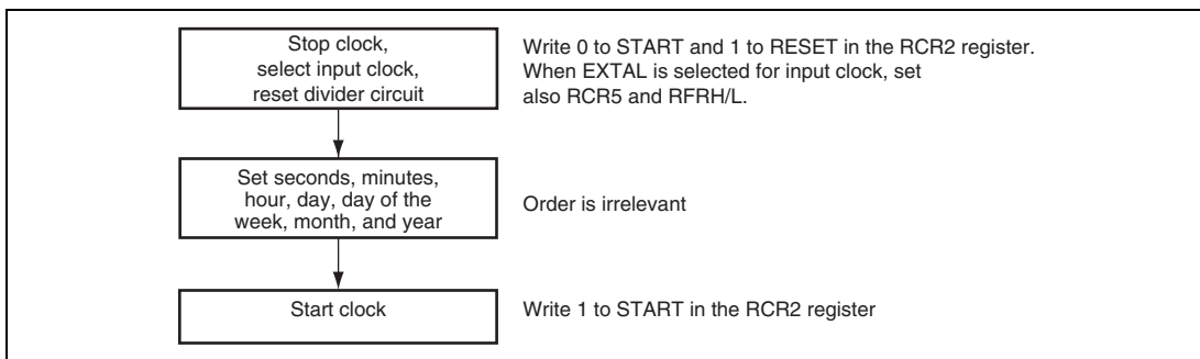
Figure 15.2 Setting Time
