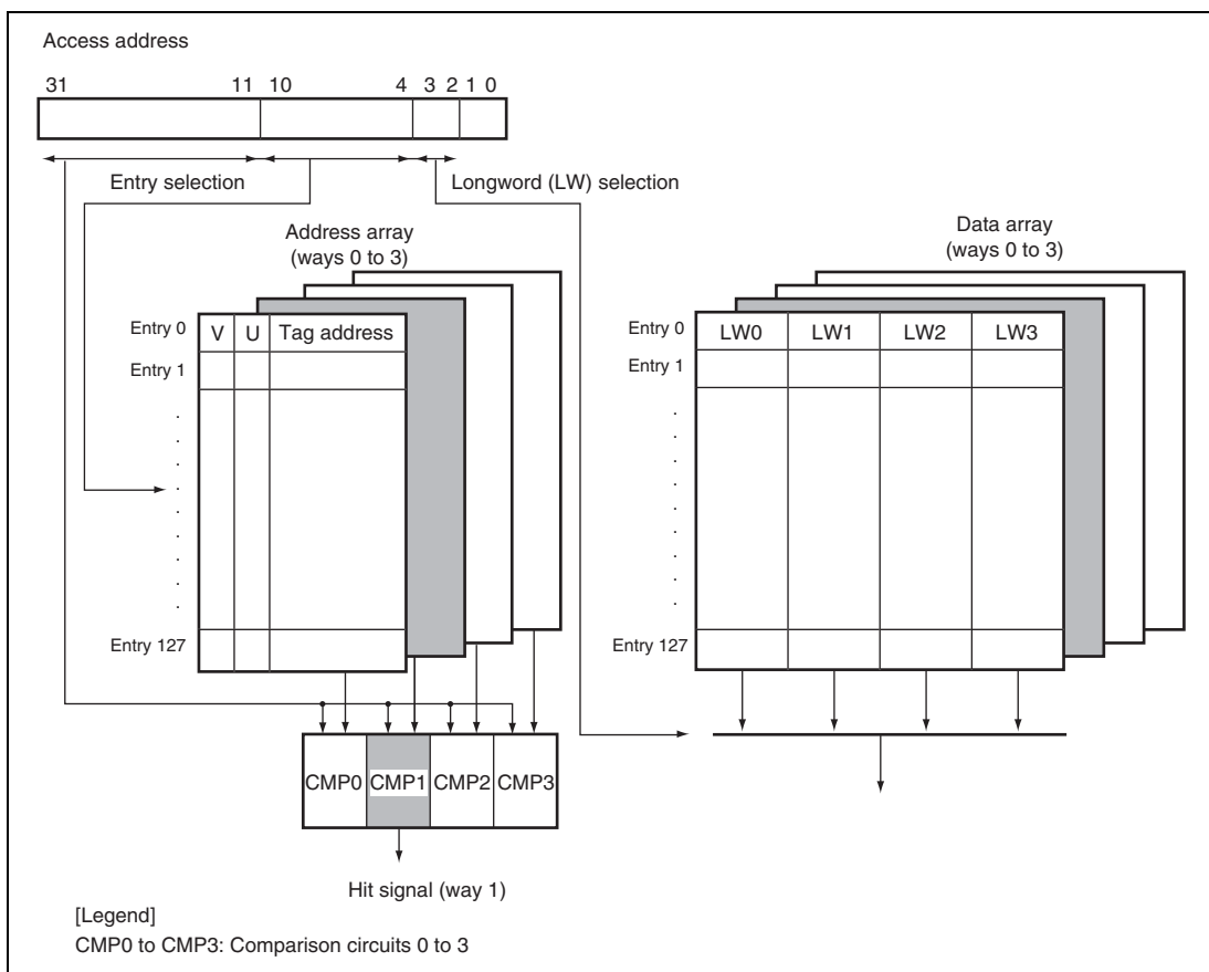
Figure 9.2 Cache Search Scheme
