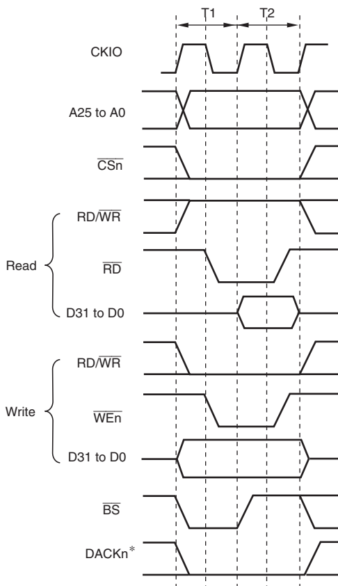
Figure 10.2 Normal Space Basic Access Timing (Access Wait 0)
