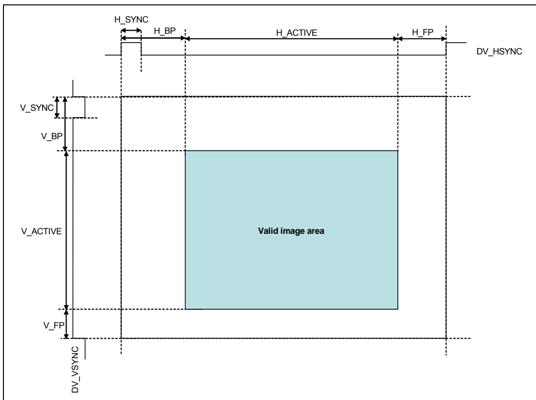
Figure 32.12 YCbCr/RGB Signal Reception Timing
