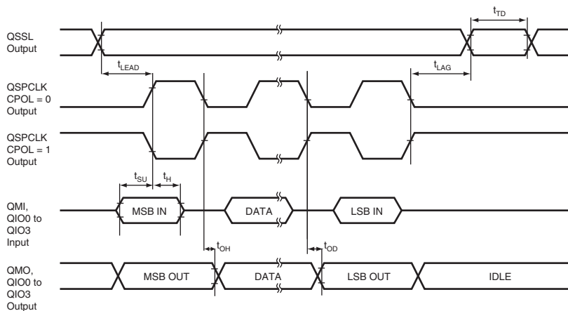
Figure 52.51 Transmission and Reception Timing (CPHA = 0)
