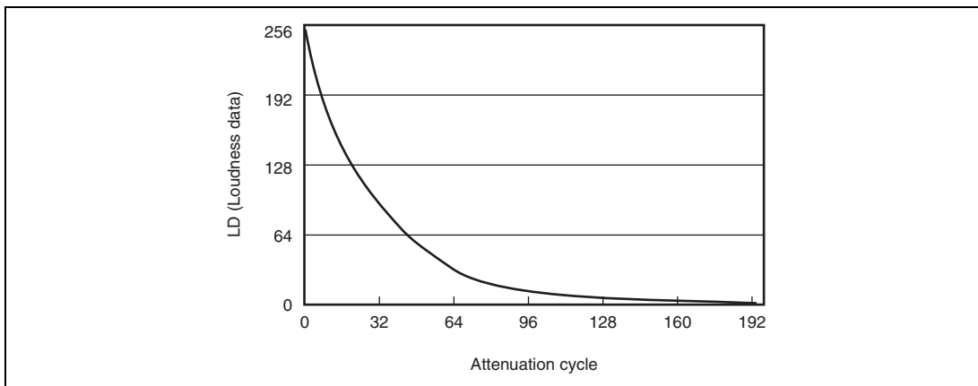
Figure 43.4 Attenuation Characteristics
