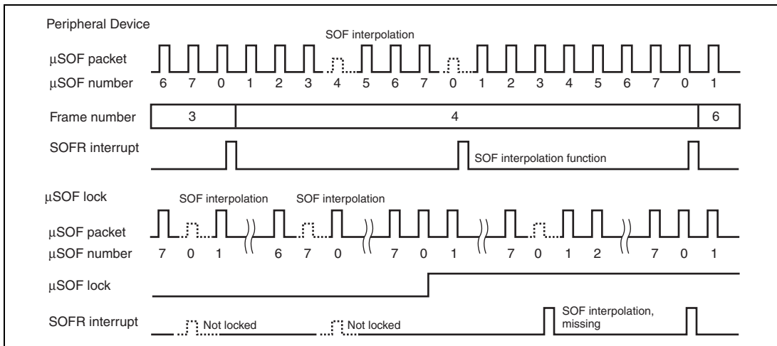
Figure 29.8 Example of SOFR Interrupt Output Timing
