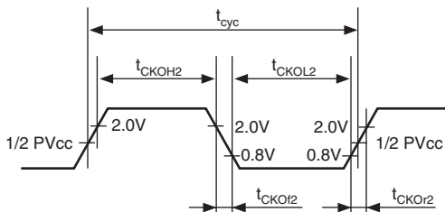
Figure 52.2 (2) CKIO Clock Output Timing 2
