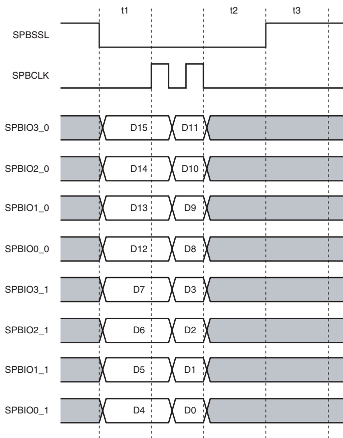
Figure 19.23 Transfer Format Example with 4-Bit Data Size and Two Serial Flash Memories Connected
