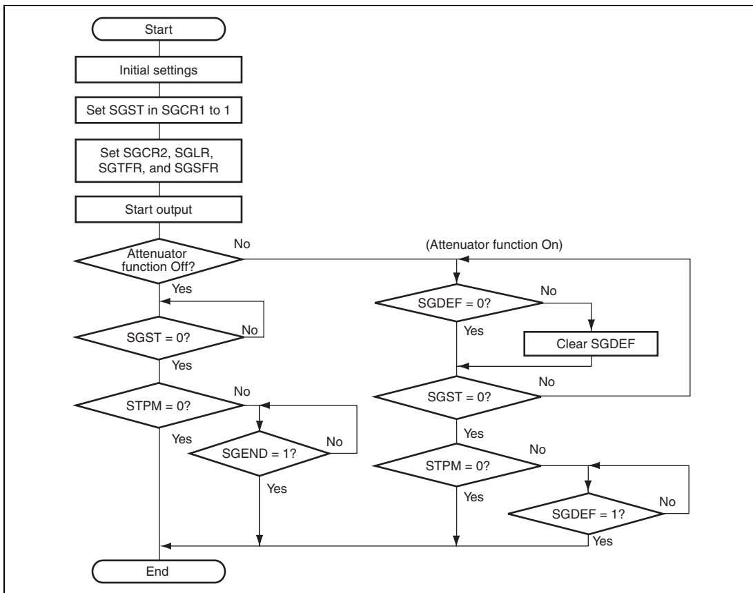
Figure 43.3 Operation Flow
