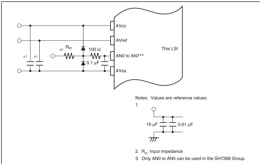
Figure 27.8 Example of Analog Input Protection Circuit
