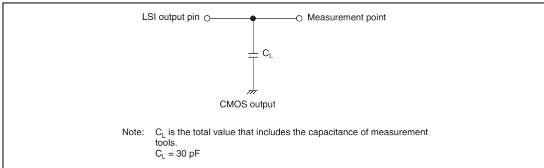
Figure 52.87 Output Load Circuit
