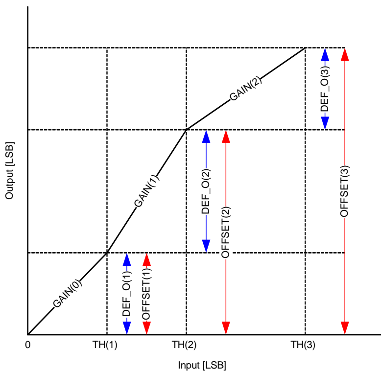
Figure 36.2 Corresponding Chart of Offset Calculation Formulas
