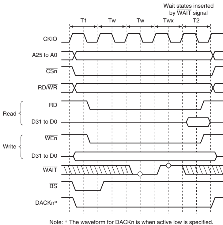
Figure 10.9 Wait Cycle Timing for Normal Space Access (Wait Cycle Insertion Using \overline{\text{WAIT}} Signal)
