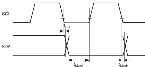
Figure 52.58(3) Transmission/Reception Timing
