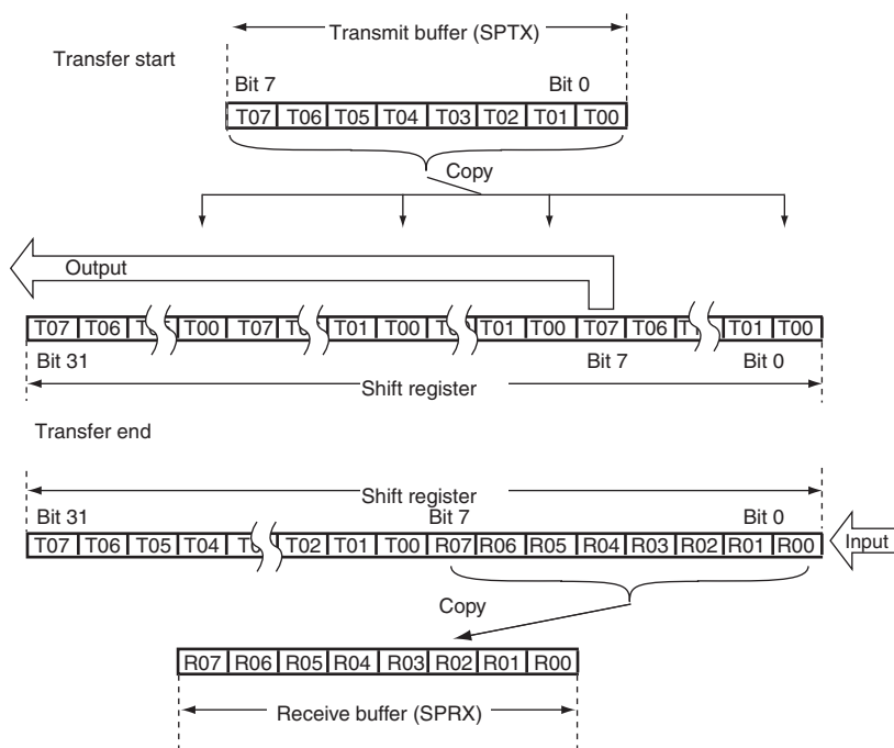
Figure 17.10 MSB First Transfer (8-Bit Data)
