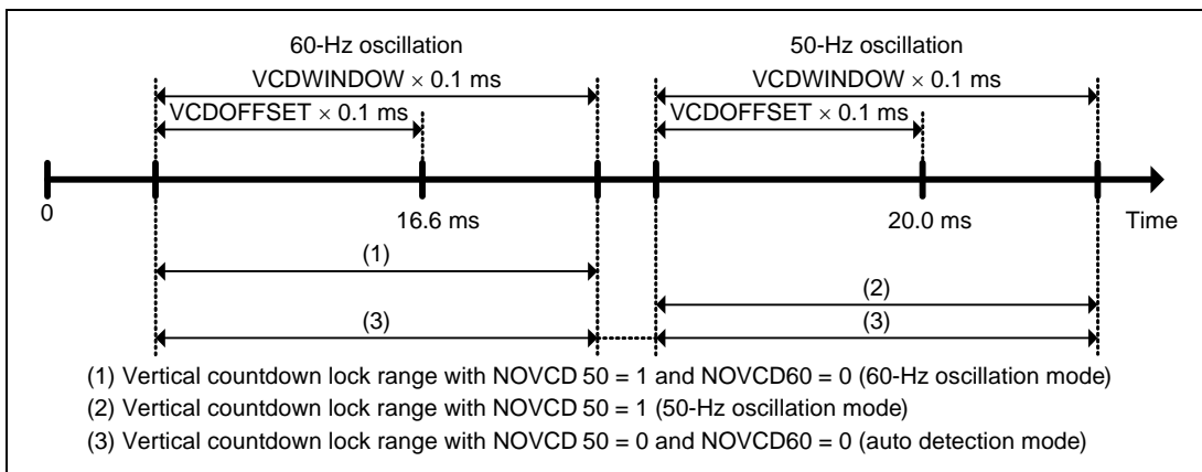
Figure 30.13 Vertical Countdown Lock Ranges
