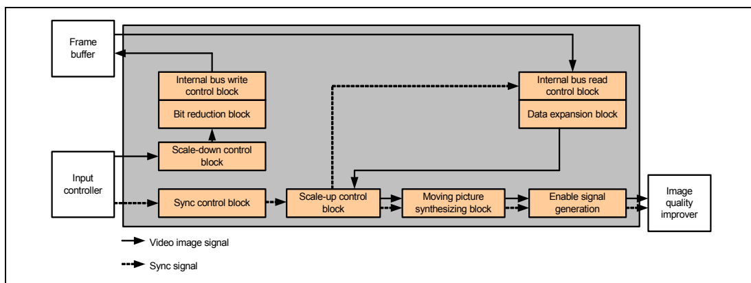
Figure 33.18 Signal Paths for Displaying Input Video Image
