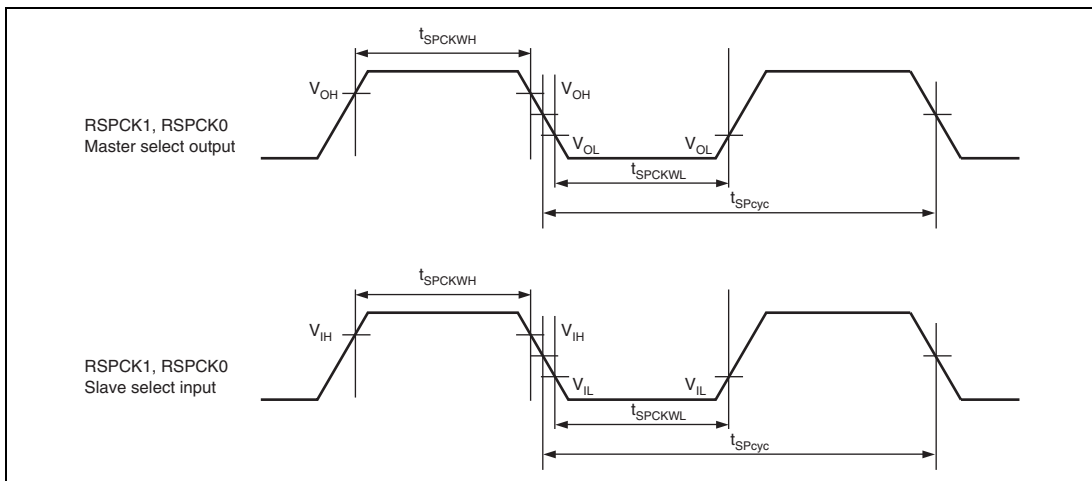
Figure 52.45 Clock Timing
