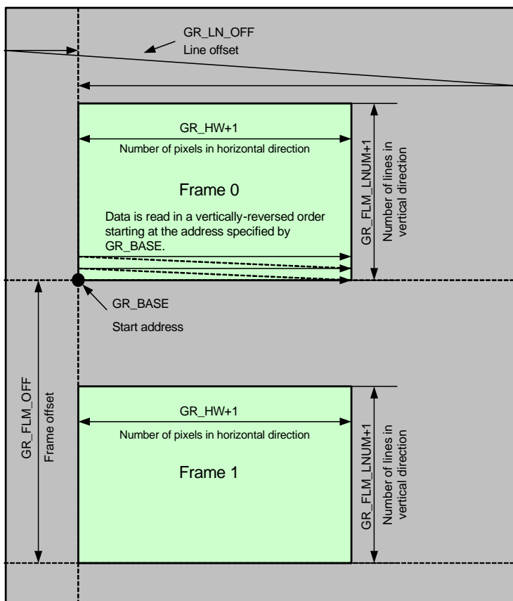
Figure 35.3 Data Arrangement with Line Offset and Decrement Control
