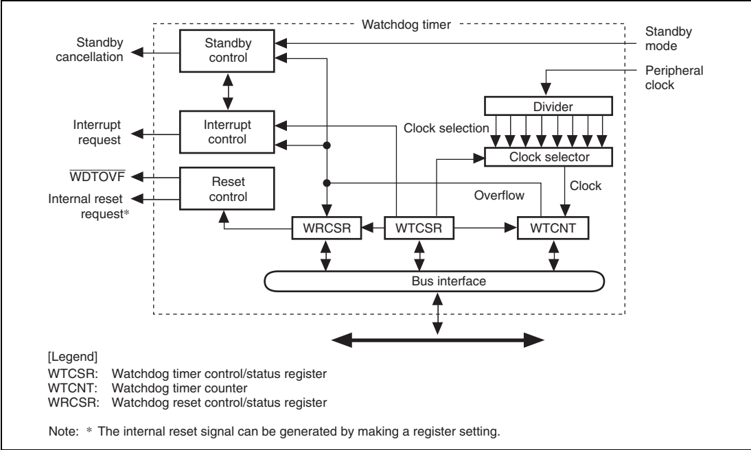
Figure 14.1 Block Diagram
