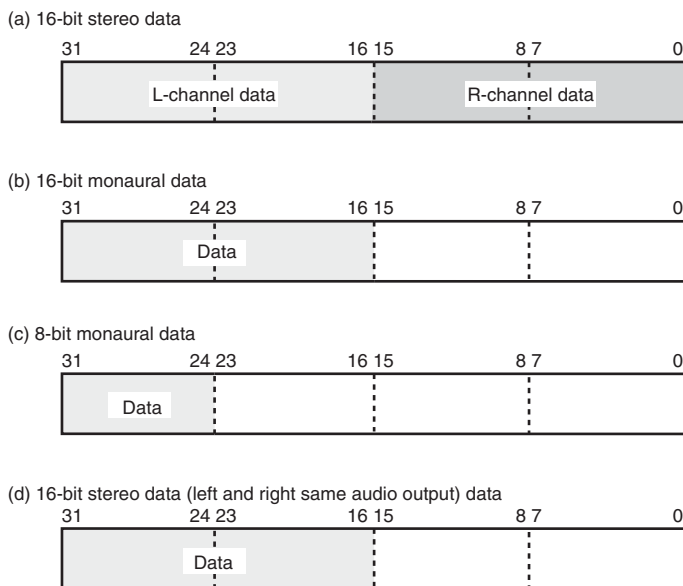
Figure 22.5 Transmit/Receive Data Bit Alignment
