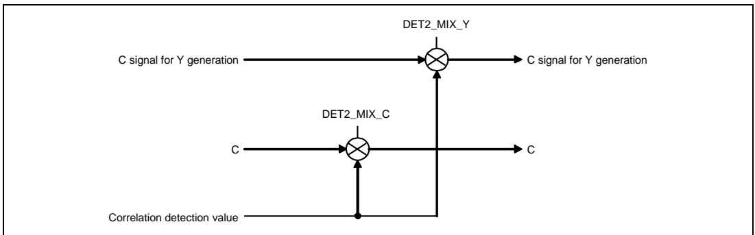
Figure 30.34 Configuration of Correlation Detection Value Mixing Block
