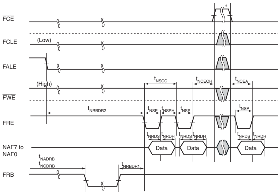
Figure 52.68 NAND Type Flash Memory Data Read Timing
