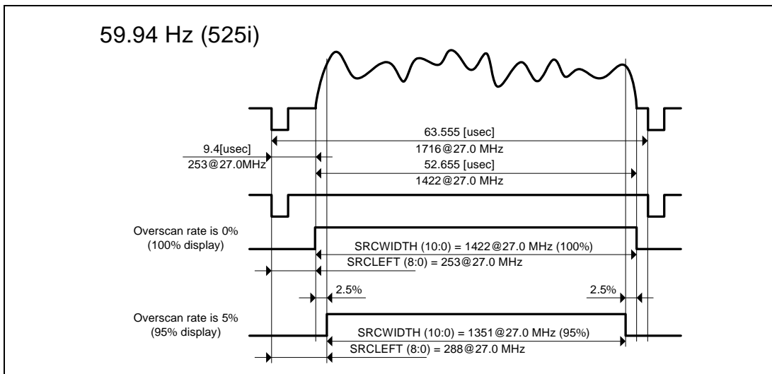
Figure 30.3 Example of Horizontal Active Image Period (59.94 Hz (525i))
