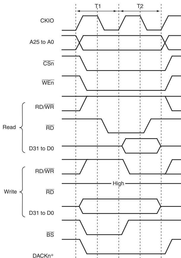
Figure 10.35 Basic Access Timing for SRAM with Byte Selection (BAS = 1)
