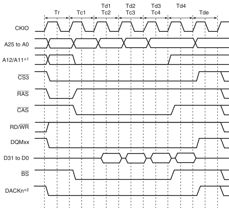
Figure 10.21 Burst Read Timing (Bank Active, Different Bank, CAS Latency 1)
