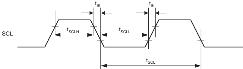
Figure 52.58(2) Clock Input/Output Timing
