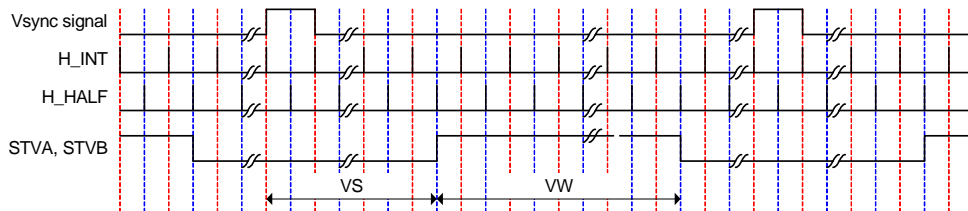
Figure 36.18 Vertical Panel Driver Signal (H_HALF Reference Operation)
