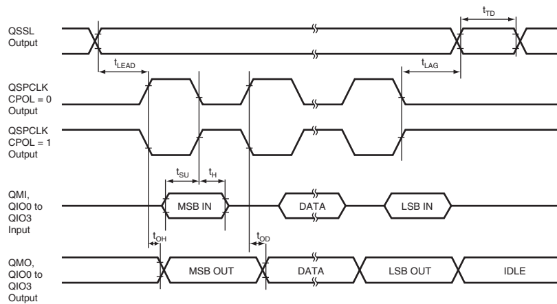
Figure 52.52 Transmission and Reception Timing (CPHA = 1)
