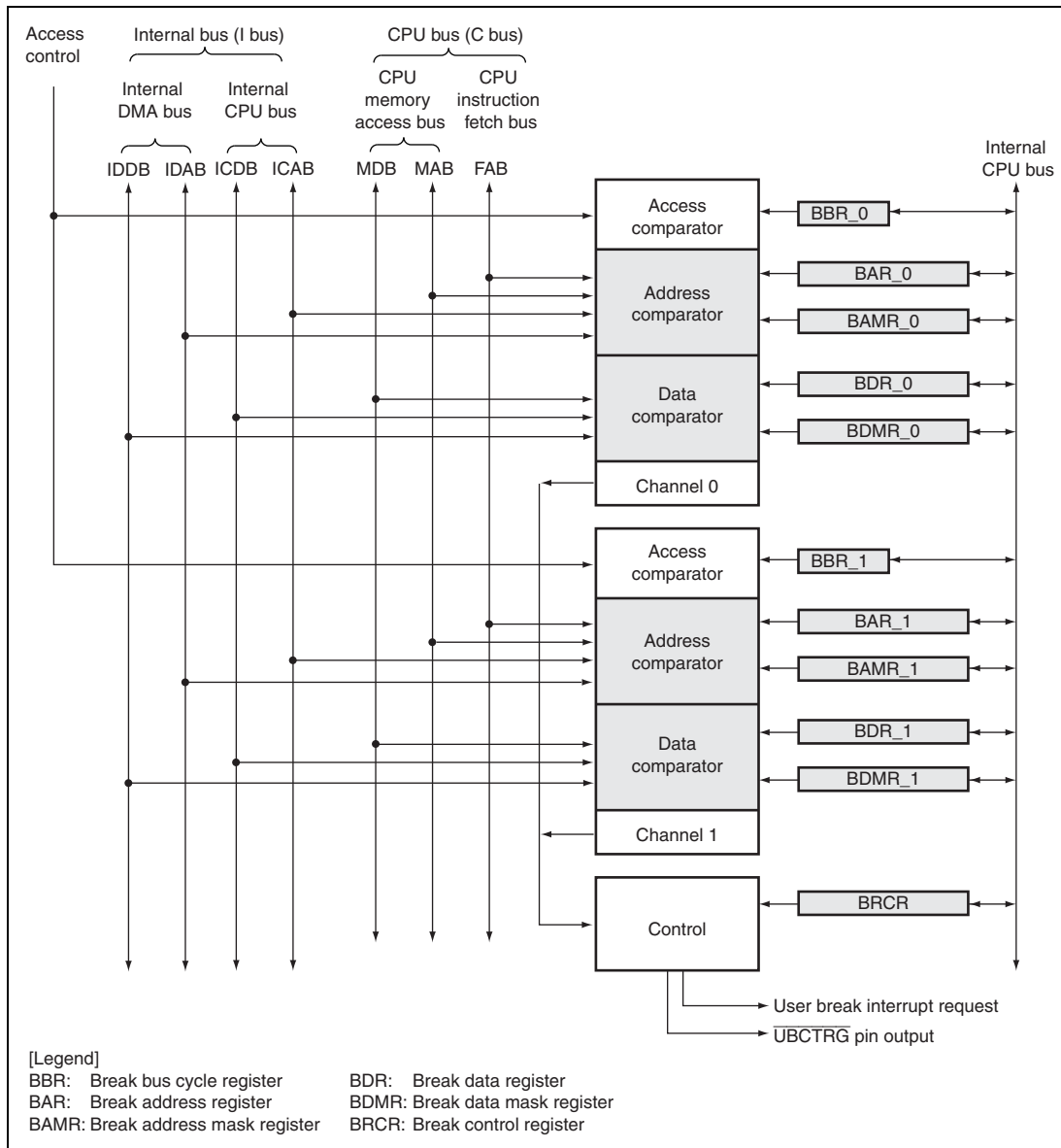
Figure 8.1 Block Diagram
