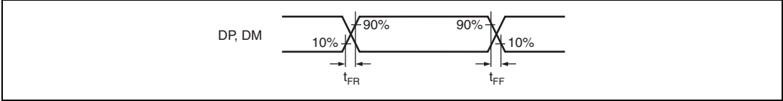
Figure 52.73 DP and DM Output Timing (Full-Speed)
