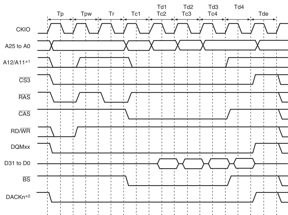
Figure 10.23 Burst Read Timing (Bank Active, Different Row Addresses in the Same Bank, CAS Latency 1)
