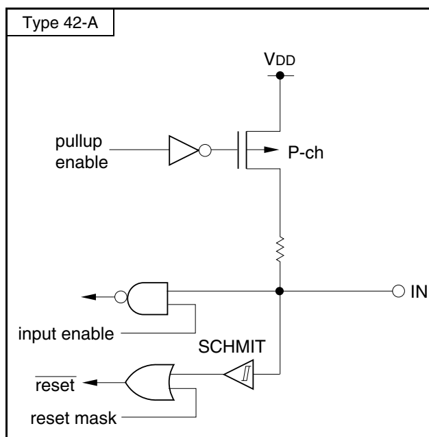
Figure 2-1. Pin I/O Circuit List (4/4)
