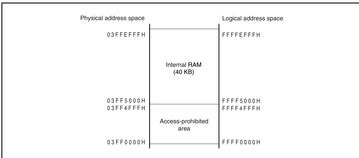
Figure 3-9. Internal RAM Area (40 KB)
