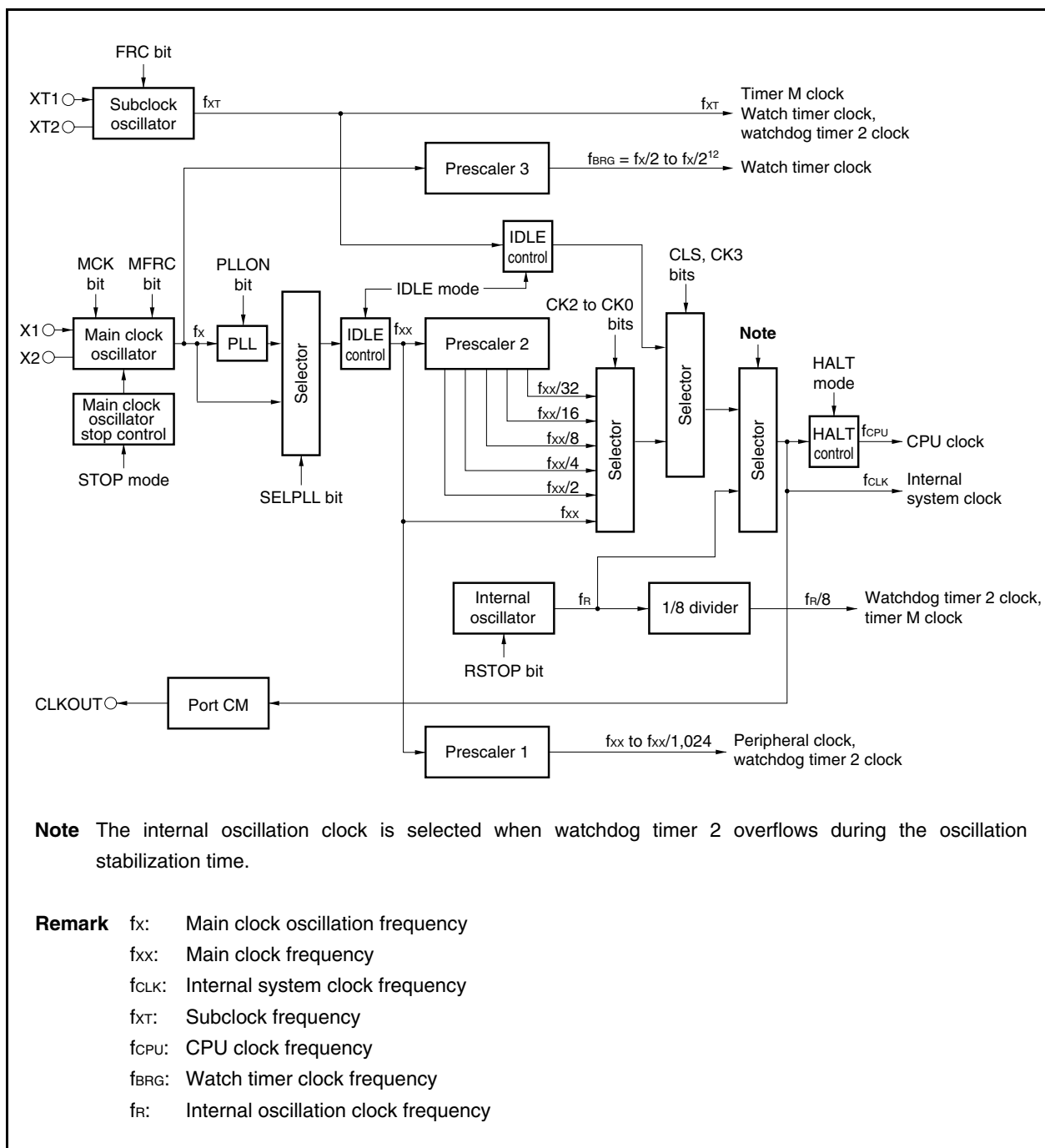
Figure 6-1. Clock Generator
