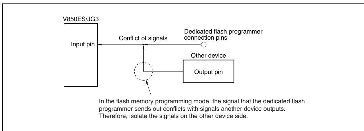
Figure 27-12. Conflict of Signals (Serial Interface Input Pin)
