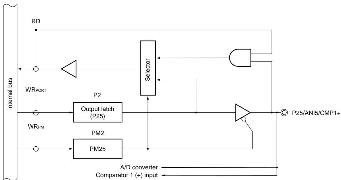
Figure 4-9. Block Diagram of P25
