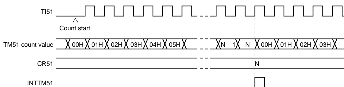
Figure 8-10. External Event Counter Operation Timing (with Rising Edge Specified)
