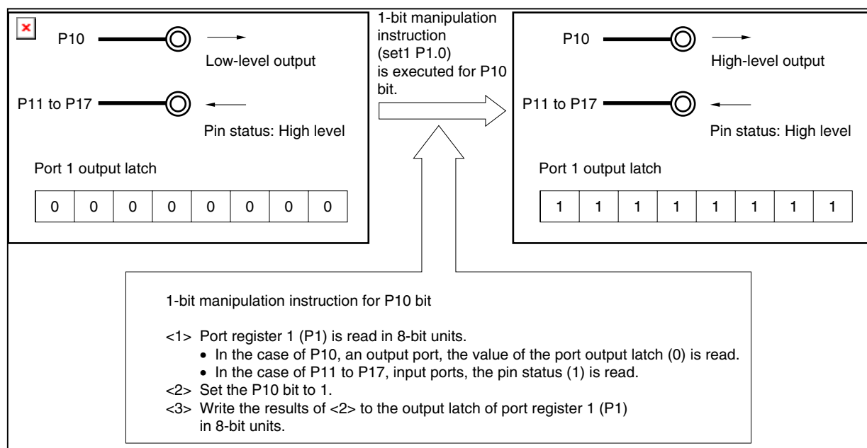
Figure 5-45. Bit Manipulation Instruction (P10)
