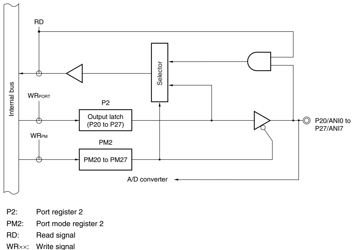
Figure 5-12. Block Diagram of P20 to P27
