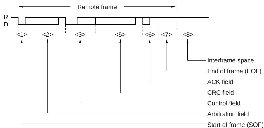
Figure 13-4. Remote Frame
