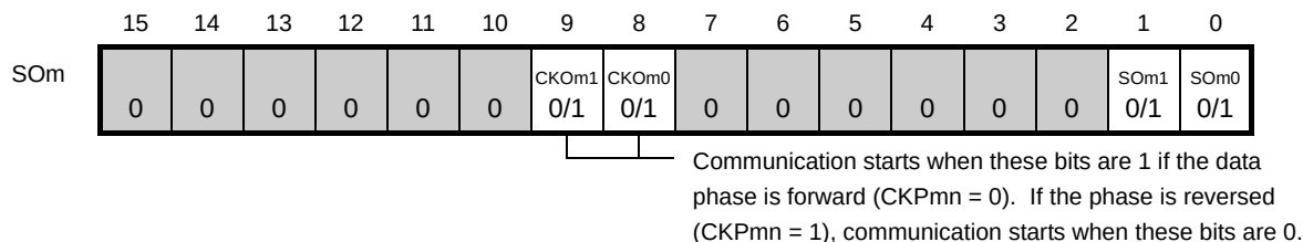
Figure 11-76. Example of Contents of Registers for Master Transmission of SPI Function (CSI00, CSI01) (1/2)
