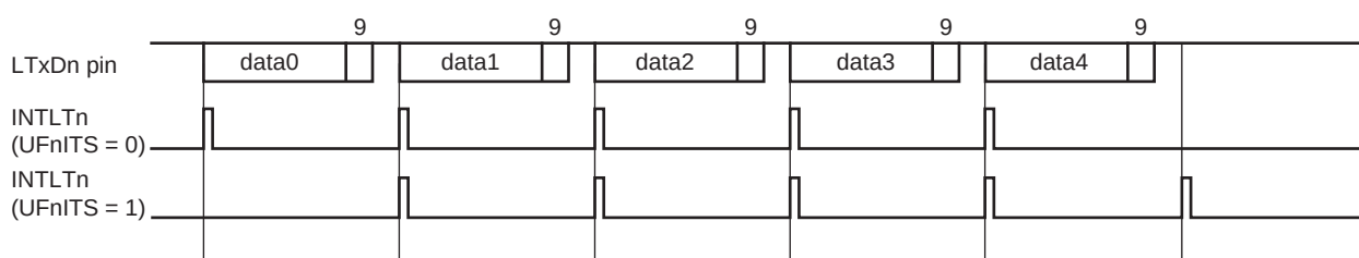
Figure 12-69. Expansion Bit Mode Transmission Example (LSB First)
