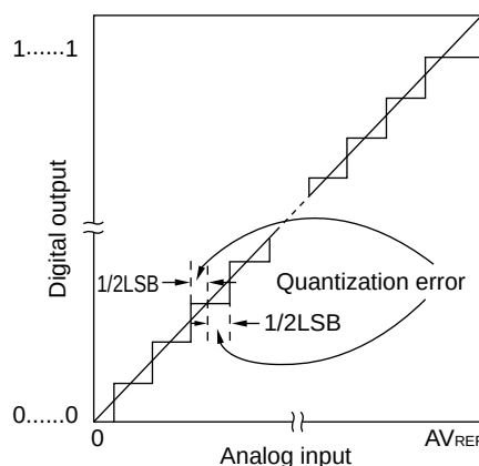
Figure 10-30. Quantization Error
