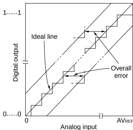
Figure 10-29. Overall Error
