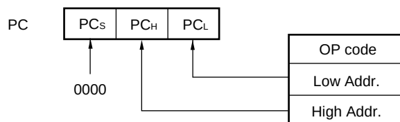
Figure 3-26. Example of CALL !addr16/BR !addr16
