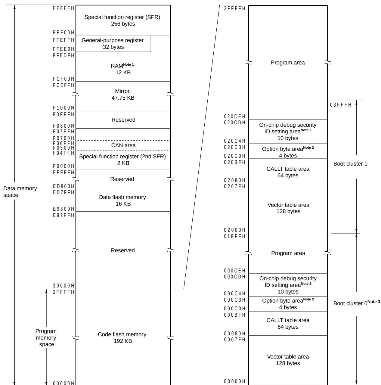
Figure 3-7. Memory Map ( \mu PD78F1829, 78F1834, 78F1839, 78F1844)
