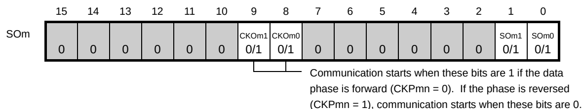
Figure 11-27. Example of Contents of Registers for Master Transmission of 3-Wire Serial I/O (CSI00, CSI01, CSI10, CSI11) (1/2)
