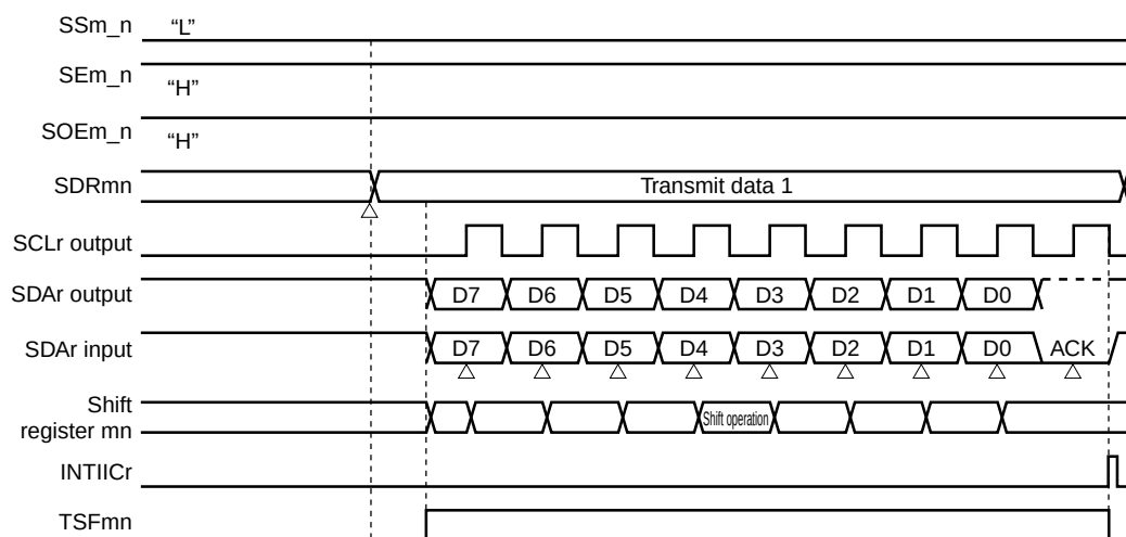
Figure 11-145. Timing Chart of Data Transmission
