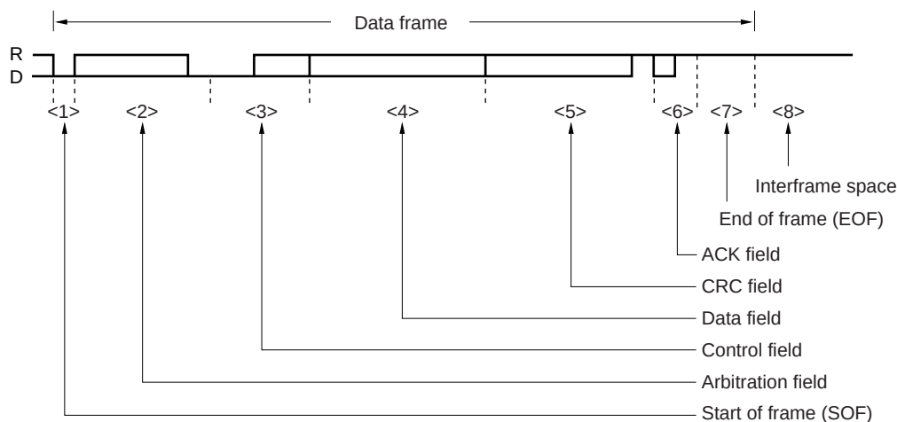
Figure 13-3. Data Frame
