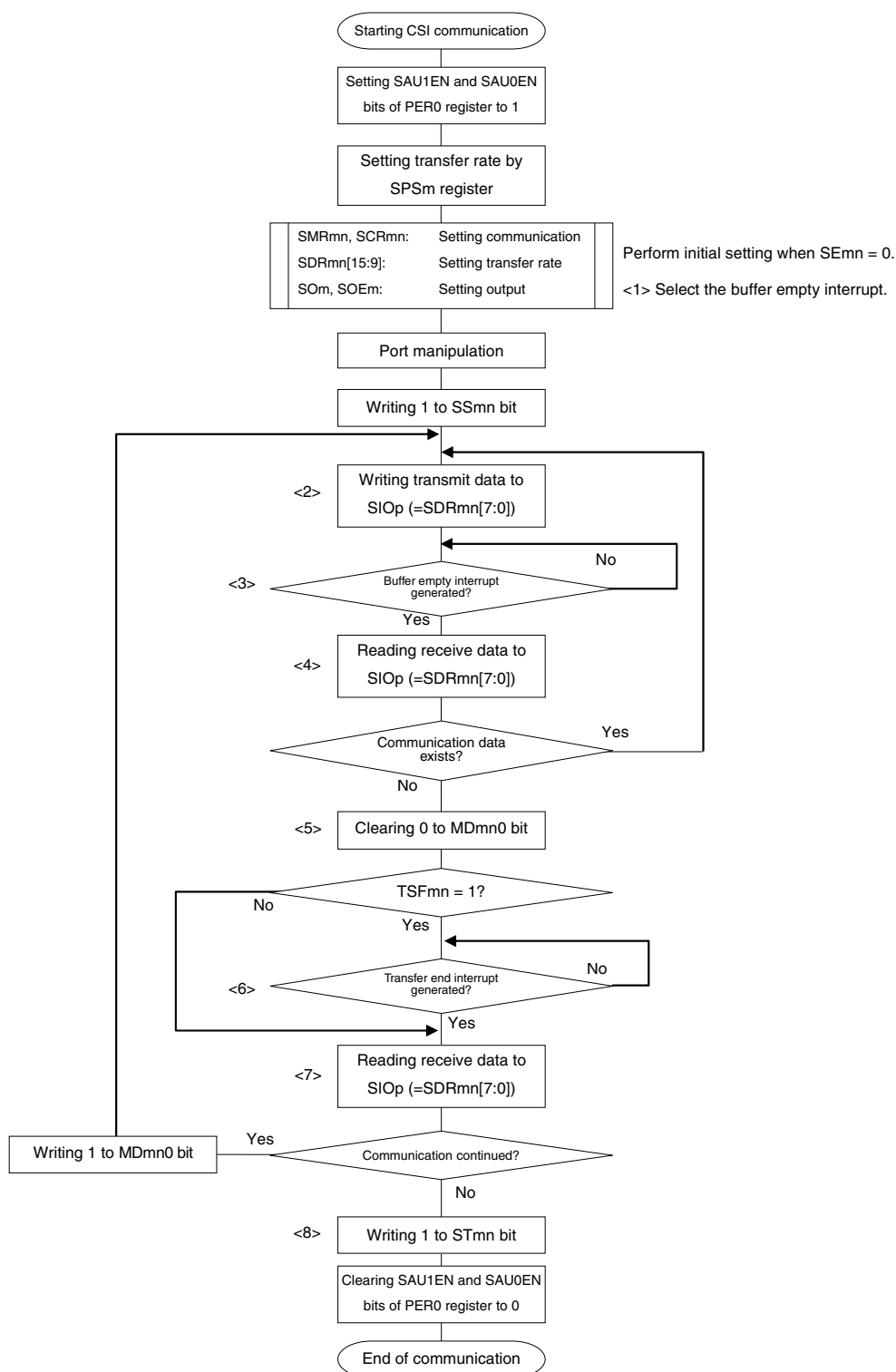
Figure 14-67. Flowchart of Slave Transmission/Reception (in Continuous Transmission/Reception Mode)
