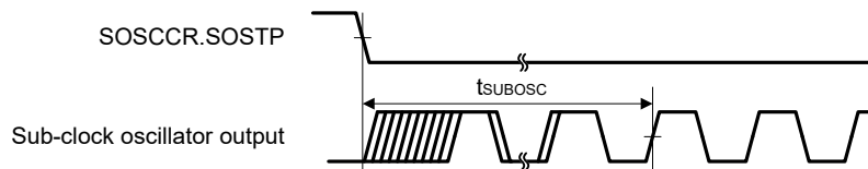
Figure 2.6 Sub-clock oscillation start timing
