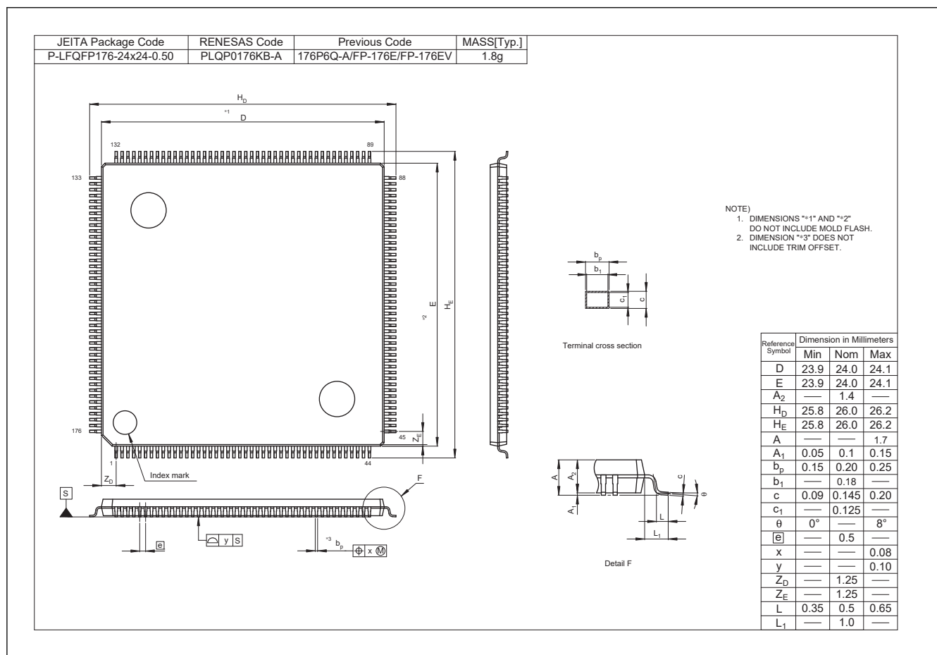
Figure 2.1 LQFP 176-pin
