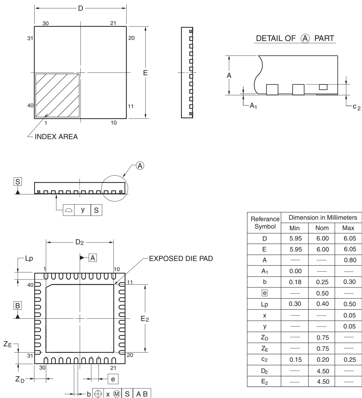
Figure 1.6 QFN 40-pin (1)
