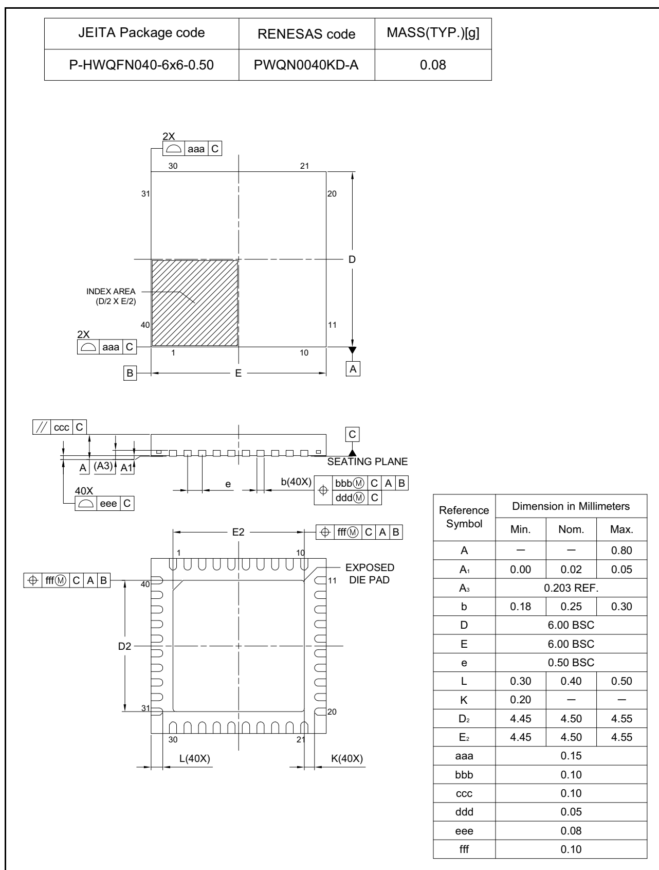
Figure 1.7 QFN 40-pin (2)
