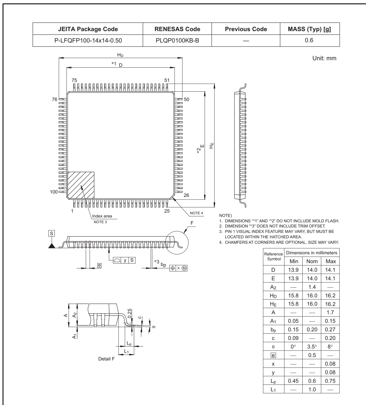
Figure 1.5 LQFP 100-pin
