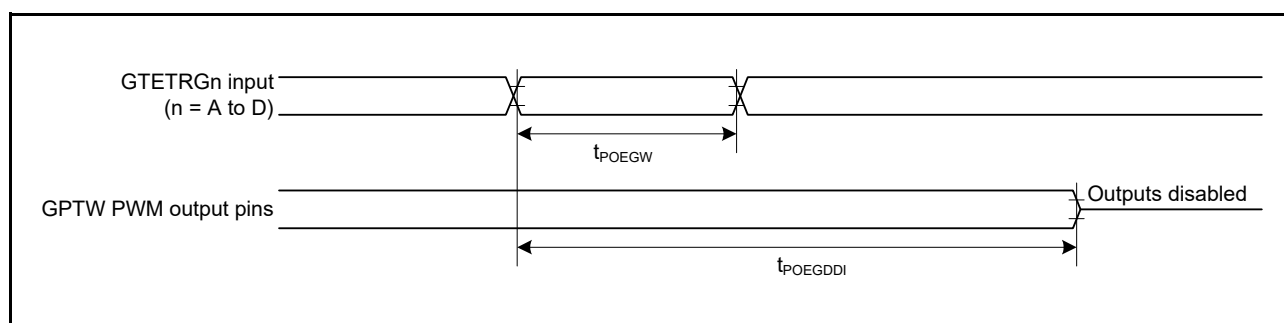
Figure 5.39 Output Disable Time for POEG in Direct Response to the Input Level Detection of the GTETR Gn pin
