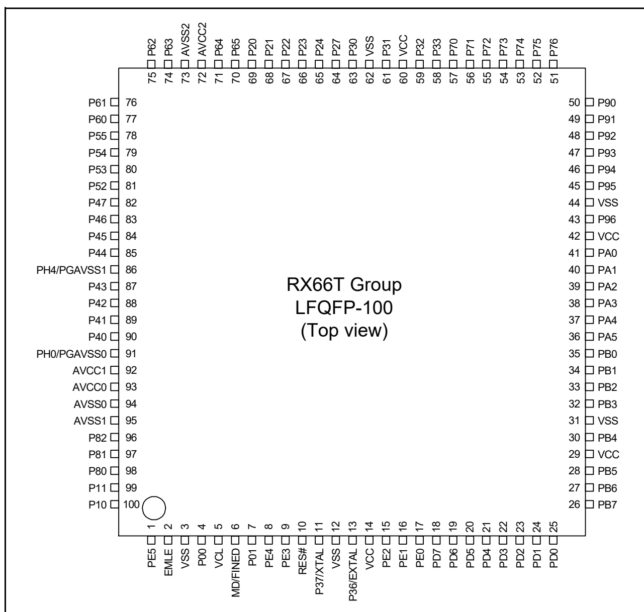
Figure 1.6 Pin Assignment (100-pin LFQFP) with PGA pseudo-differential input and without USB pin
