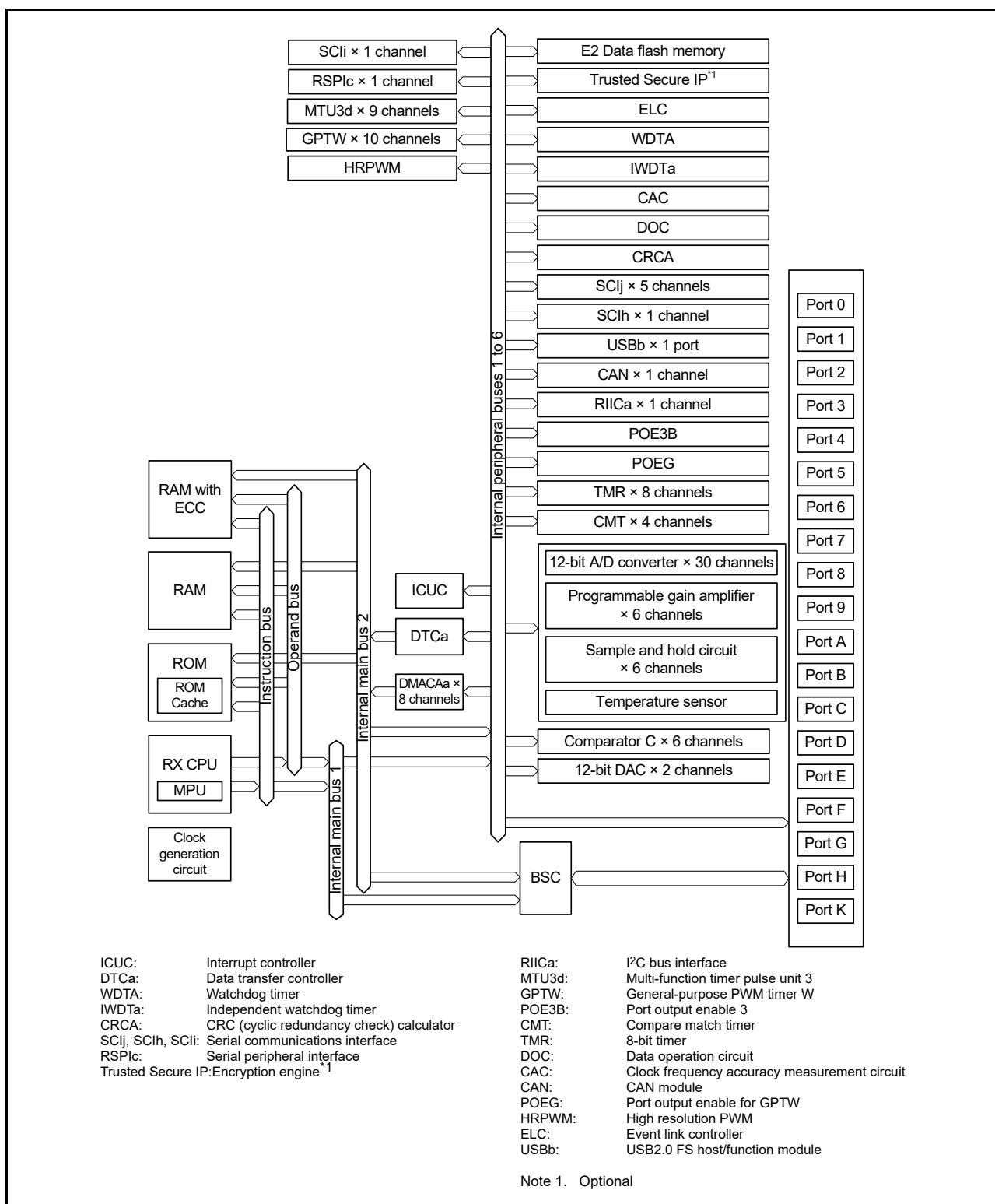
Figure 1.2 Block Diagram
