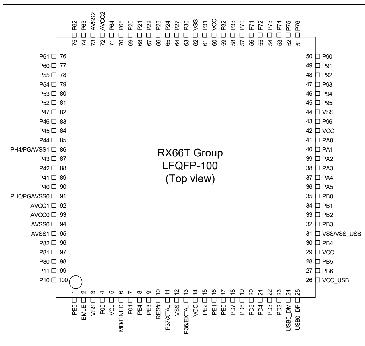
Figure 1.5 Pin Assignment (100-pin LFQFP) with PGA pseudo-differential input and with USB pin
