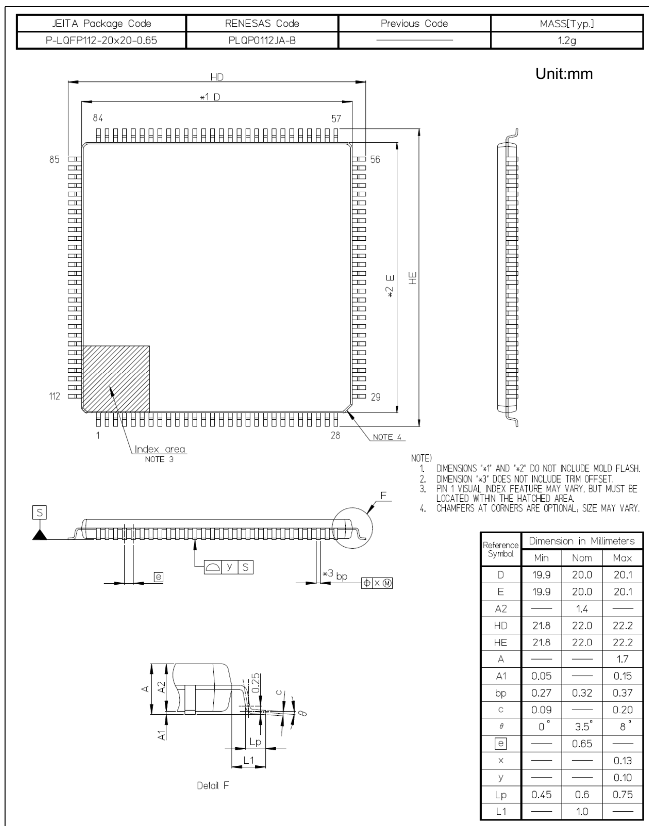
Figure B 112-Pin LQFP (PLQP0112JA-B)
