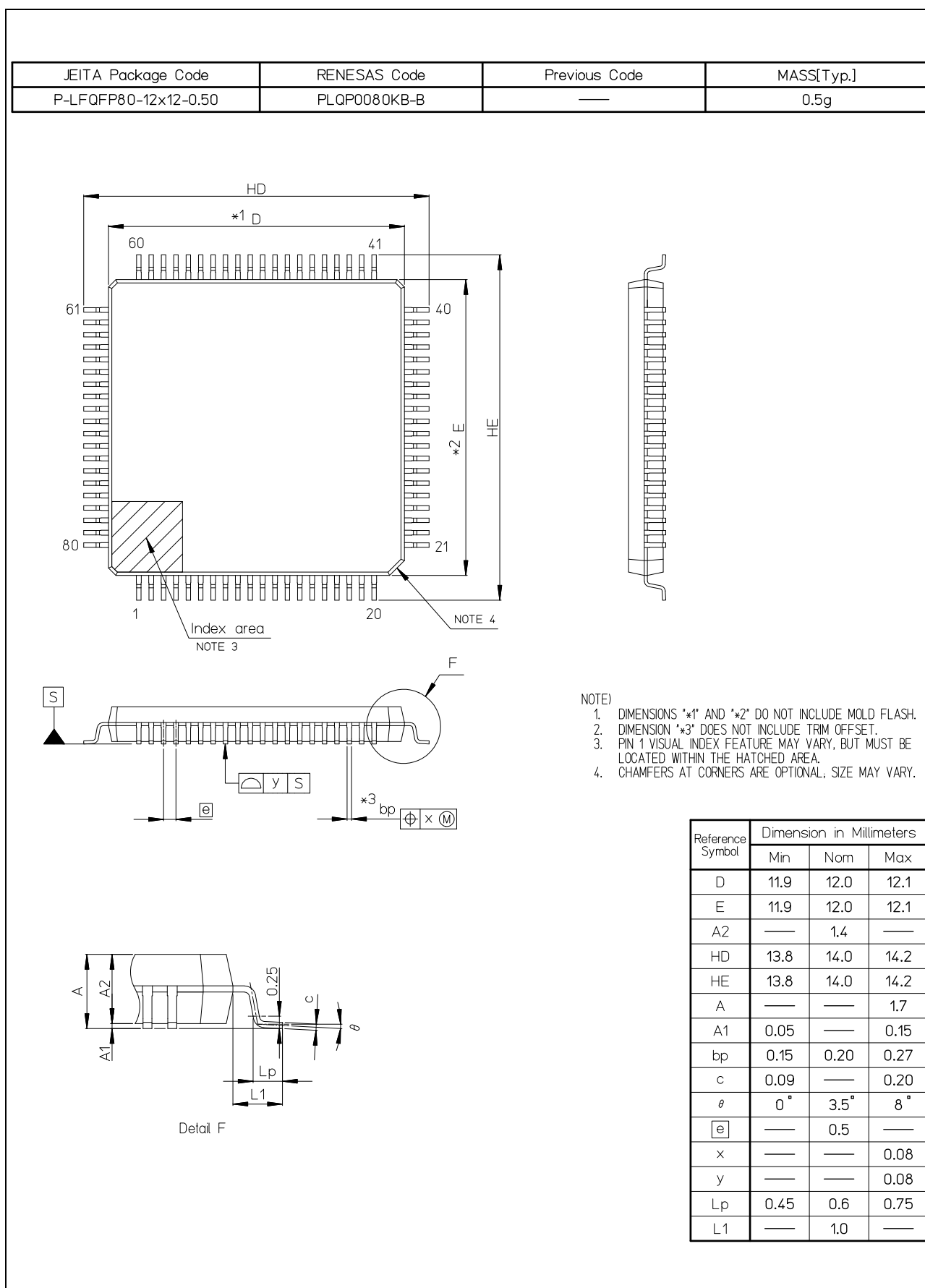
Figure E 80-Pin LFQFP (PLQP0080KB-B)
