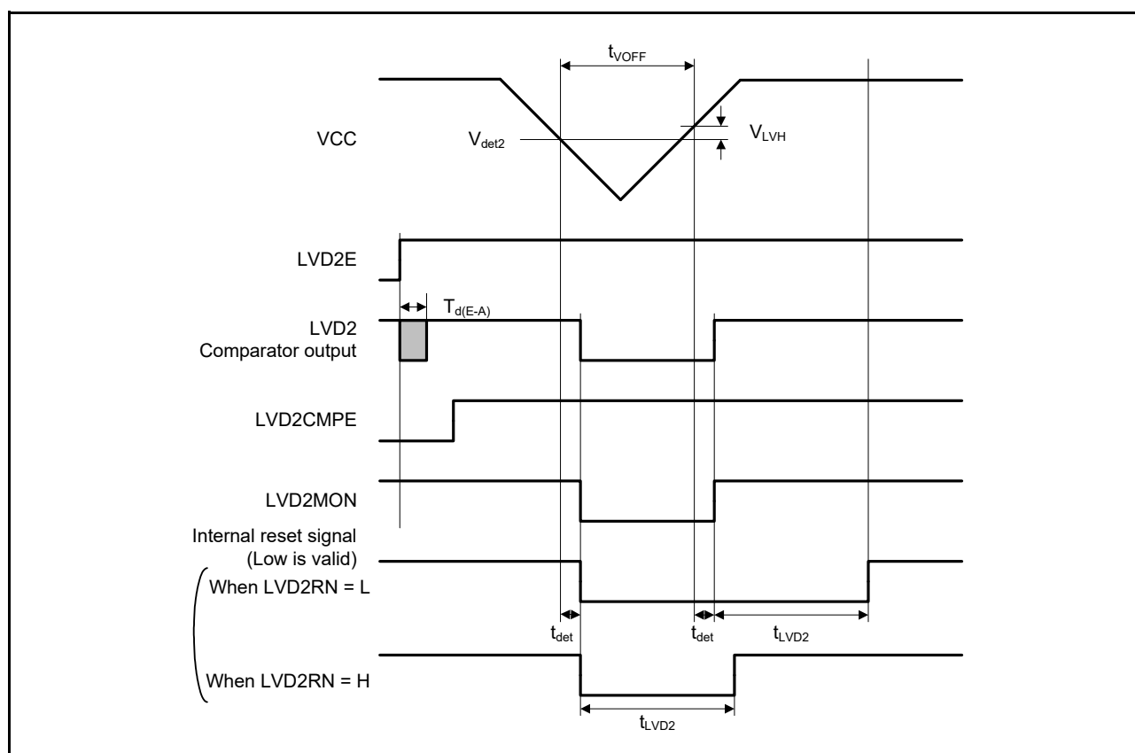
Figure 5.64 Voltage Detection Circuit Timing ( V_{\text{det2}} )
