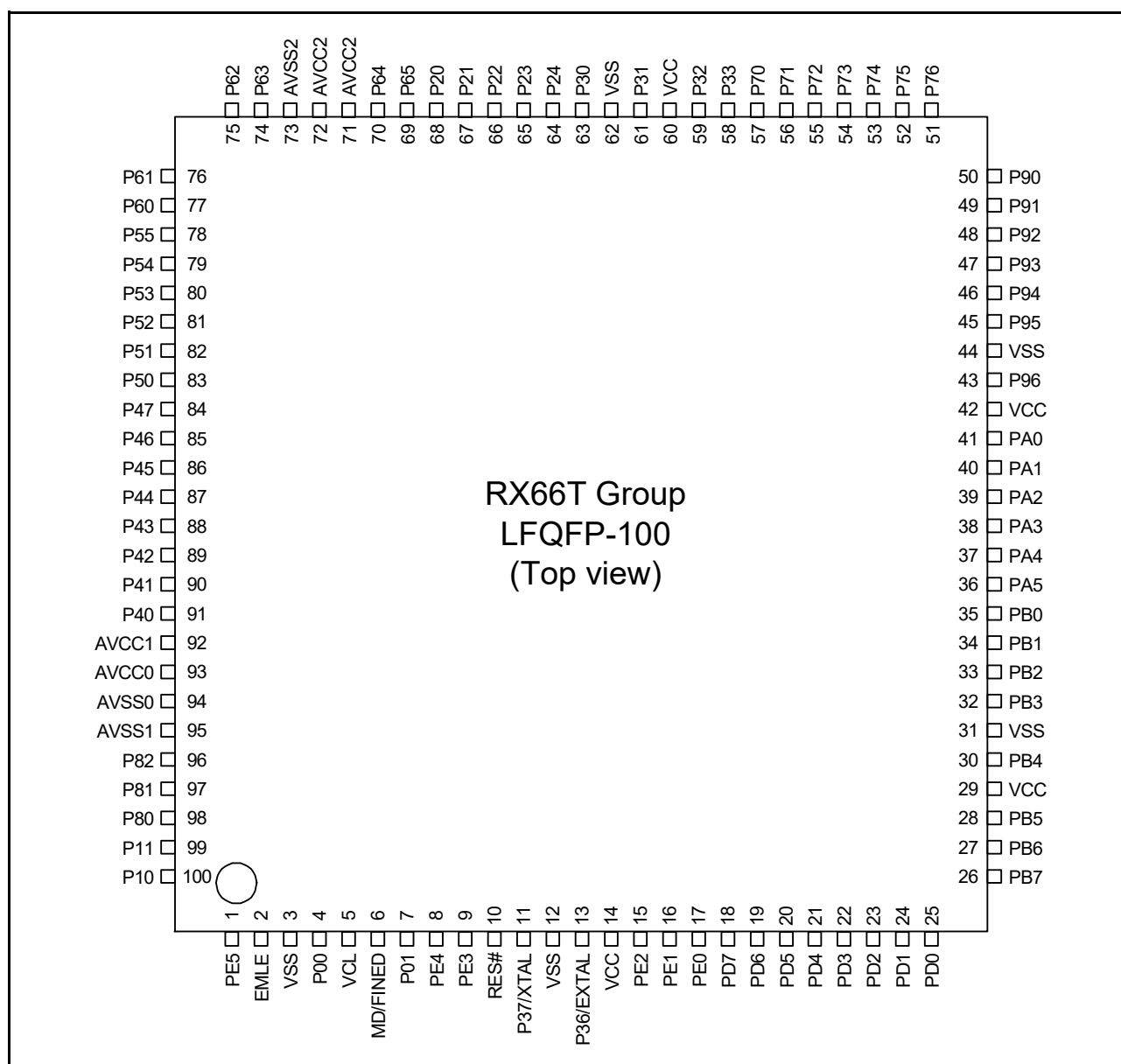
Figure 1.7 Pin Assignment (100-pin LFQFP) without PGA pseudo-differential input and without USB pin
