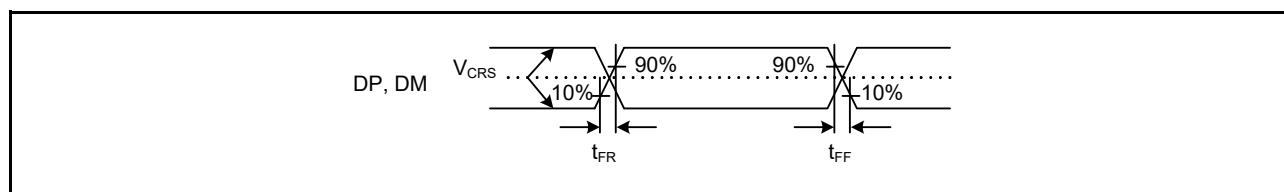
Figure 5.57 DP and DM Output Timing (Full-Speed)
