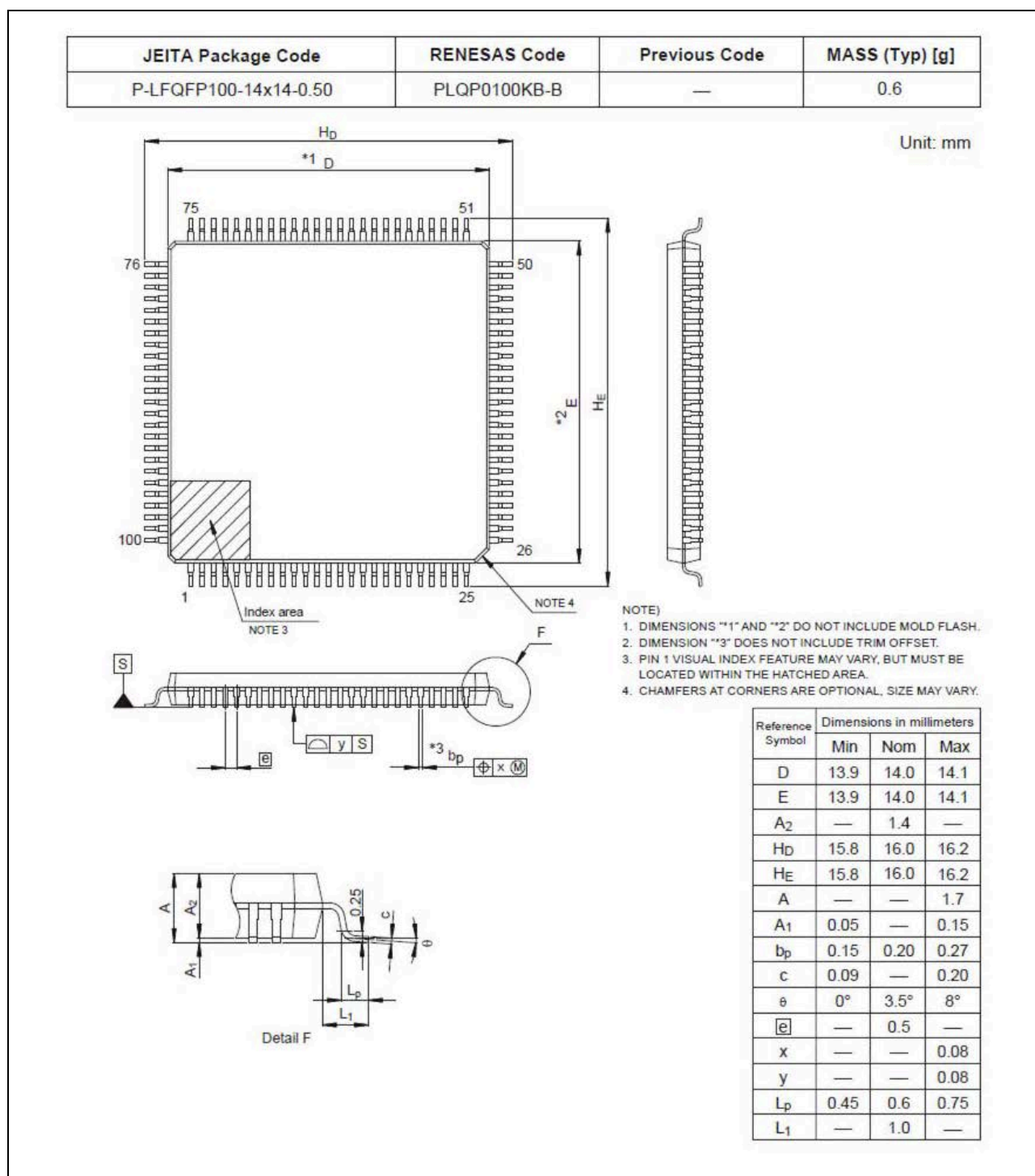
Figure C 100-Pin LFQFP (PLQP0100KB-B)
