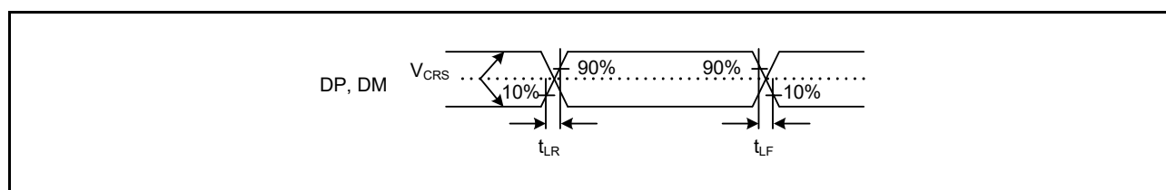
Figure 5.55 DP and DM Output Timing (Low Speed)
