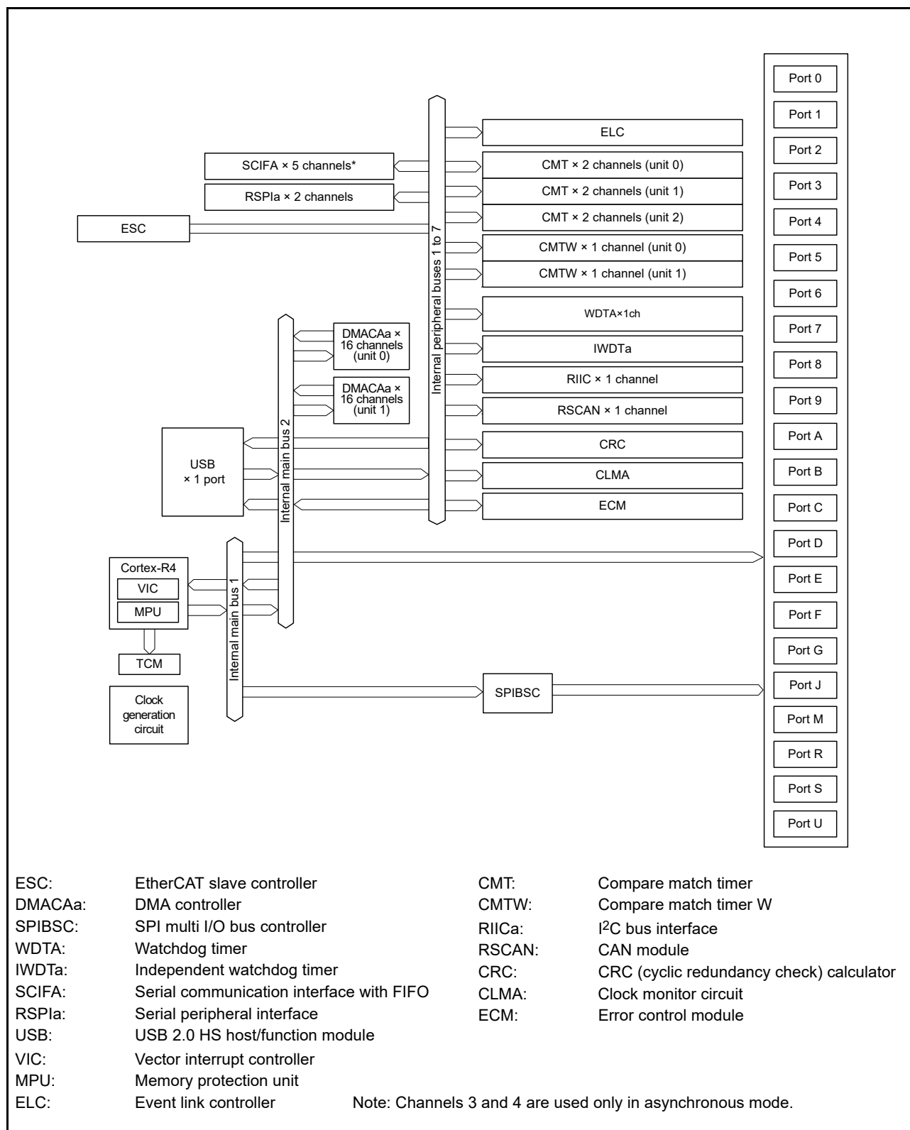
Figure 1.1 Block Diagram
