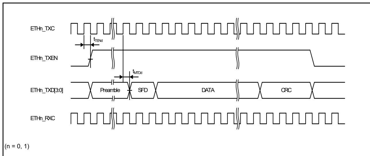
Figure 2.27 MII Transmission Timing
