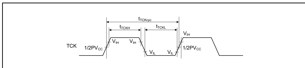
Figure 2.36 TCK Input Timing
