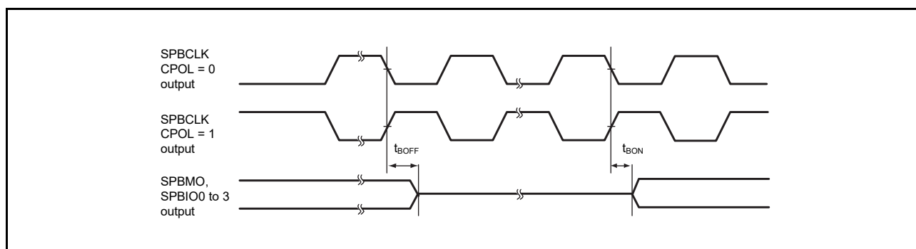
Figure 2.24 SPIBSC Buffer On/Off Timing (CPHAT = 0, CPHAR = 1)
