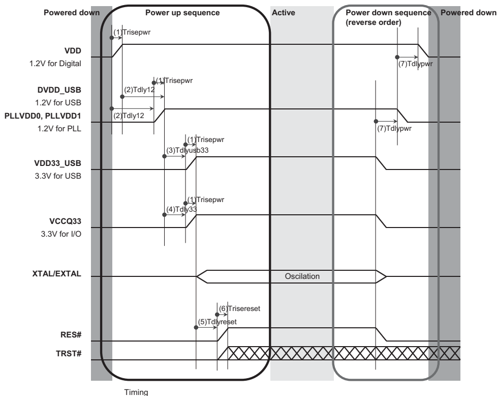
Timing
