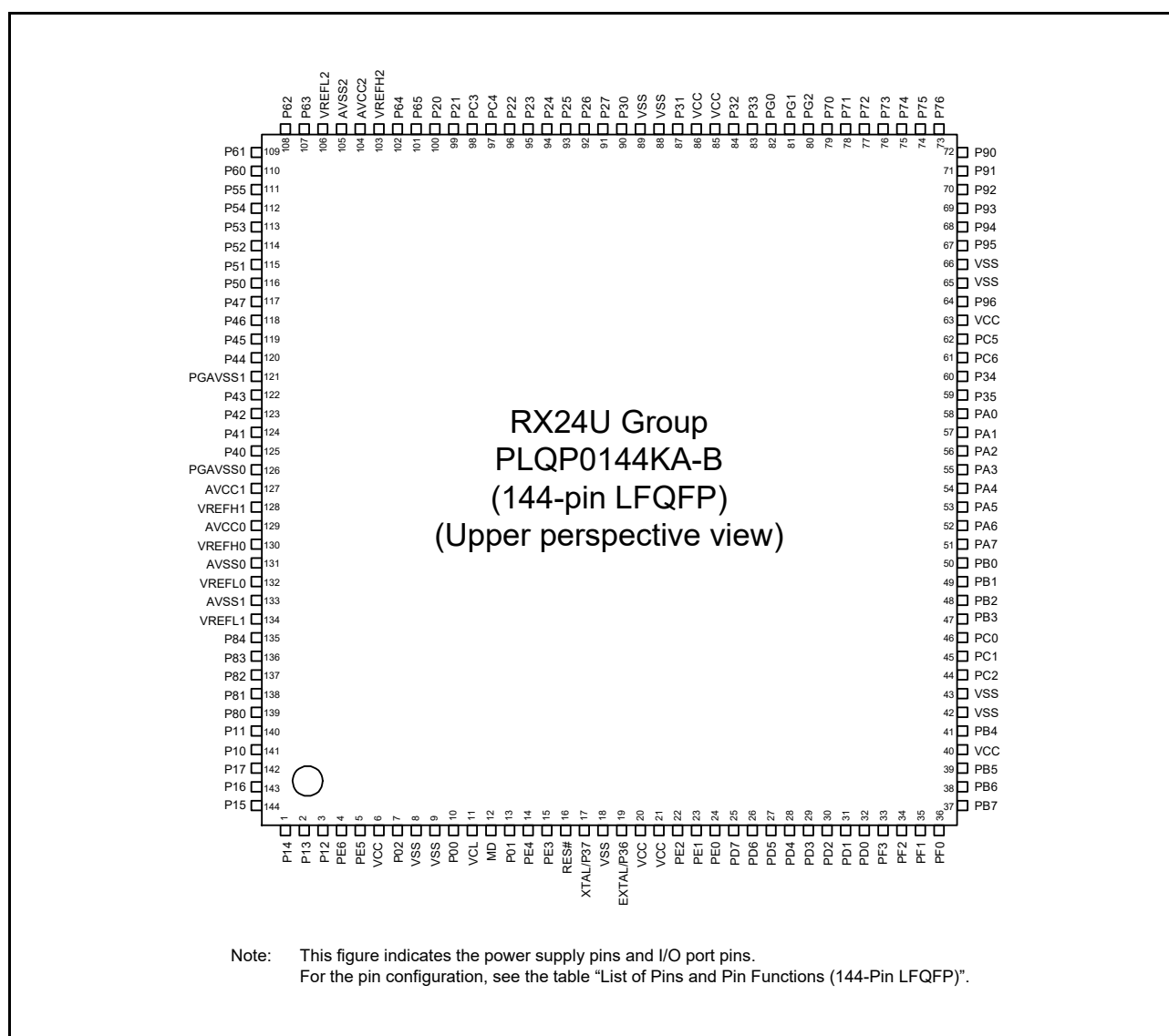
Figure 1.3 Pin Assignments of the 144-Pin LFQFP
