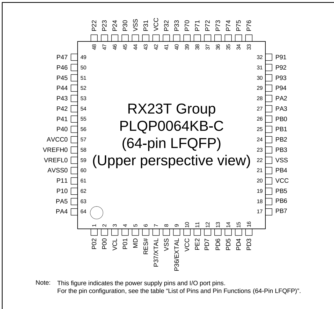
Figure 1.3 Pin Assignments of the 64-Pin LFQFP
