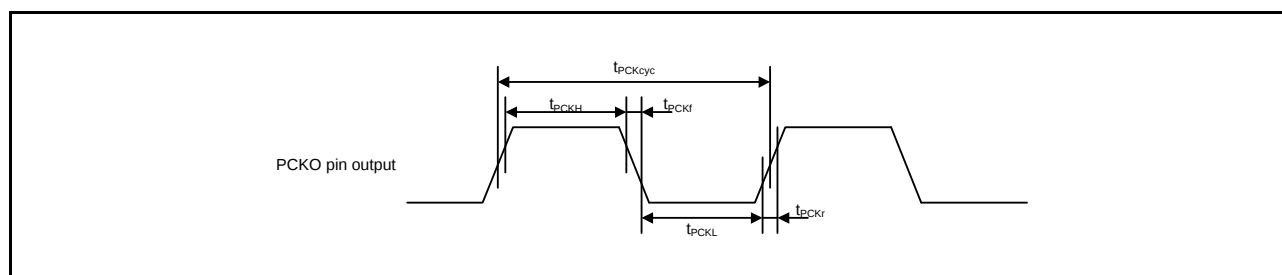
Figure 5.73 PDC Output Clock Timing
