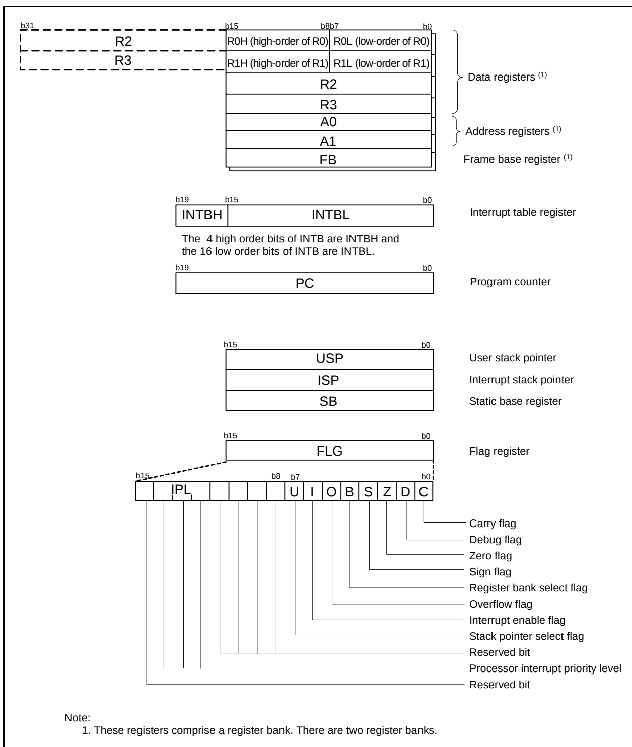
Figure 2.1 CPU Registers
