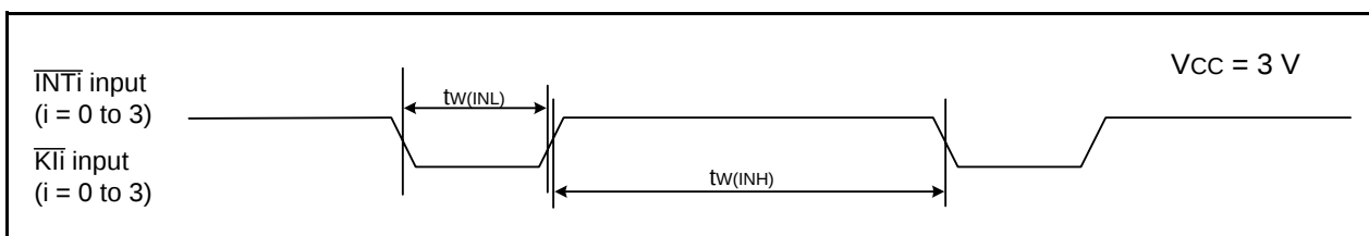
Figure 5.15 Input Timing Diagram for External Interrupt \overline{\text{INTi}} and Key Input Interrupt \overline{\text{Kli}} when V_{CC} = 3\text{ V}
