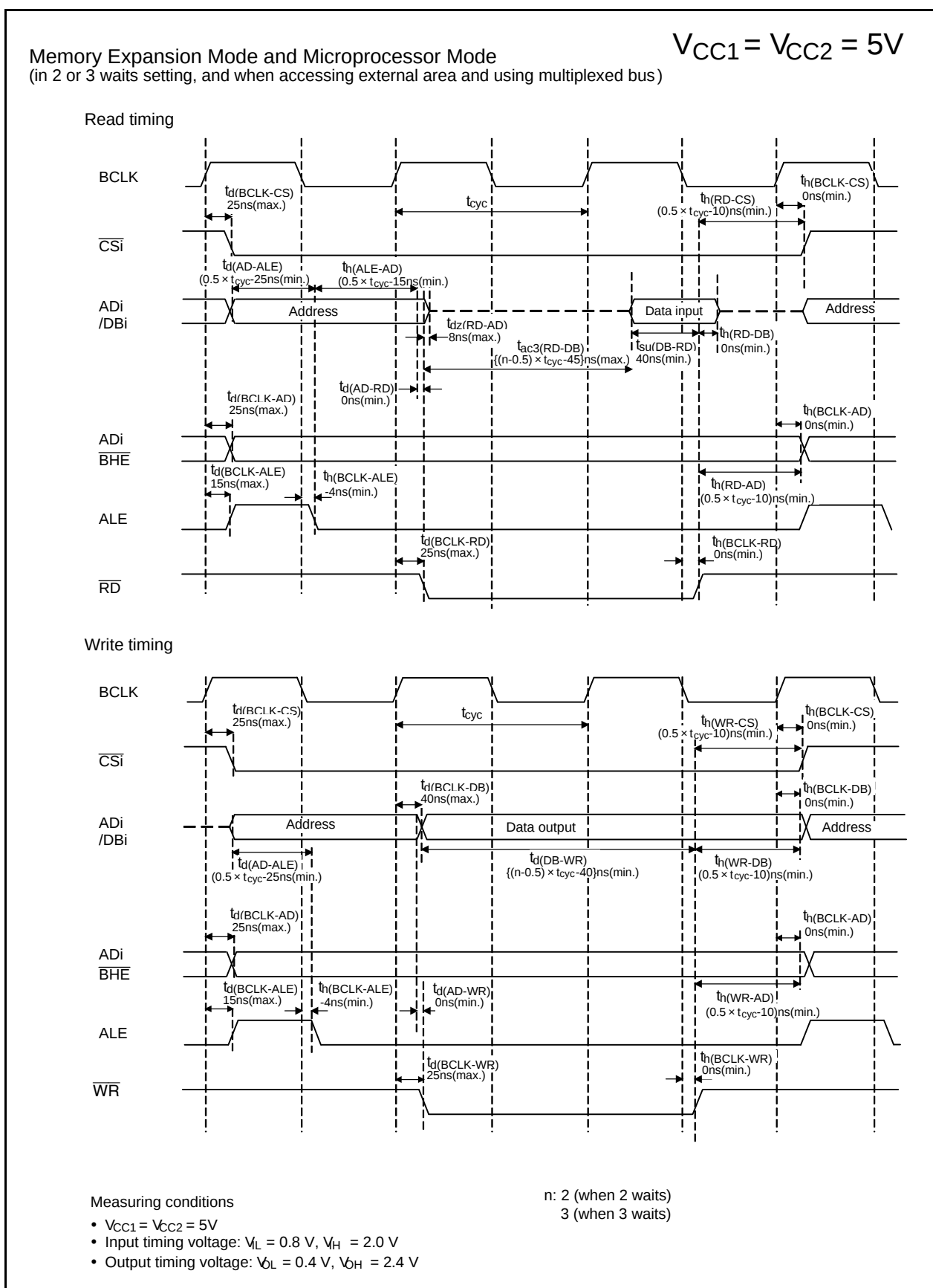
Figure 5.20 Timing Diagram
