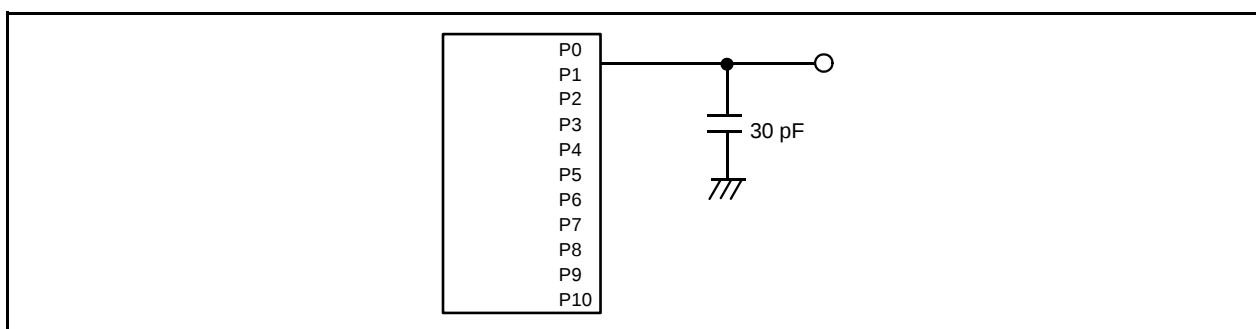
Figure 5.17 Ports P0 to P10 Measurement Circuit
