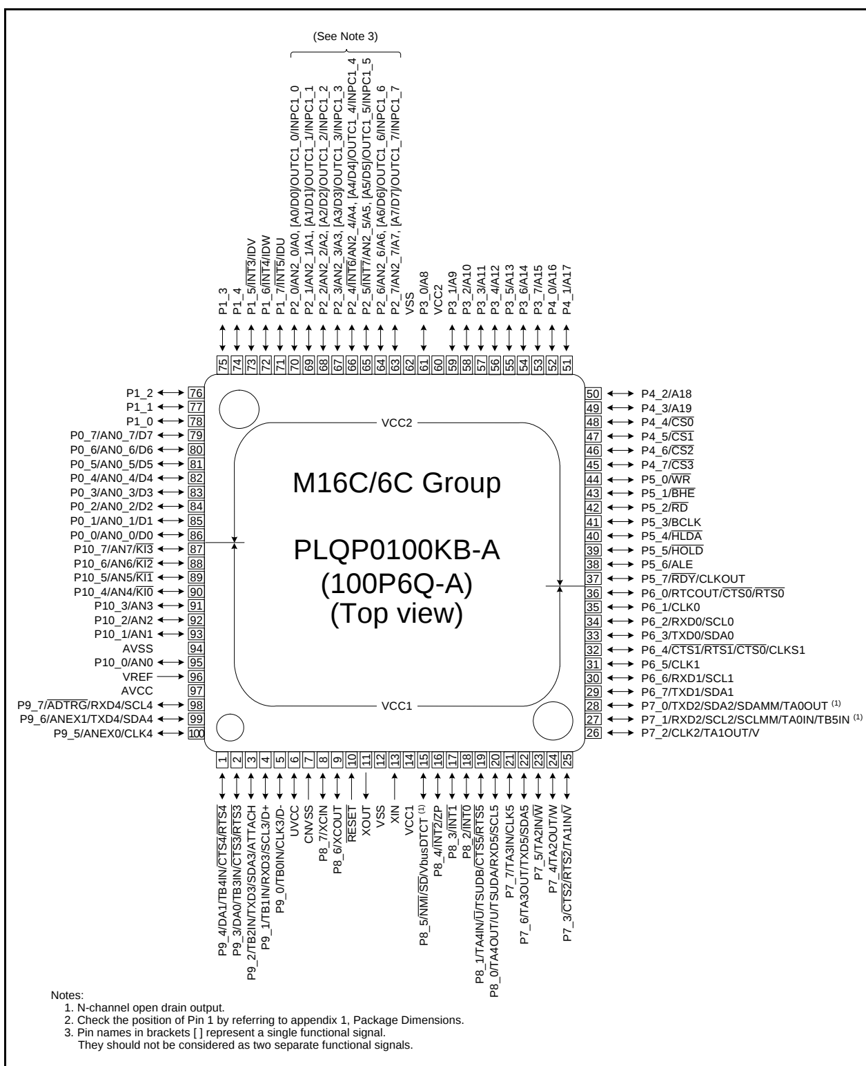
Figure 1.5 Pin Assignment
