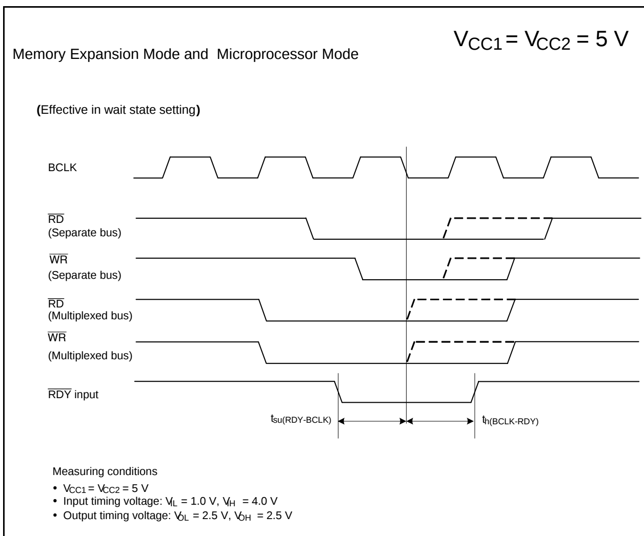
Figure 5.16 Timing Diagram
