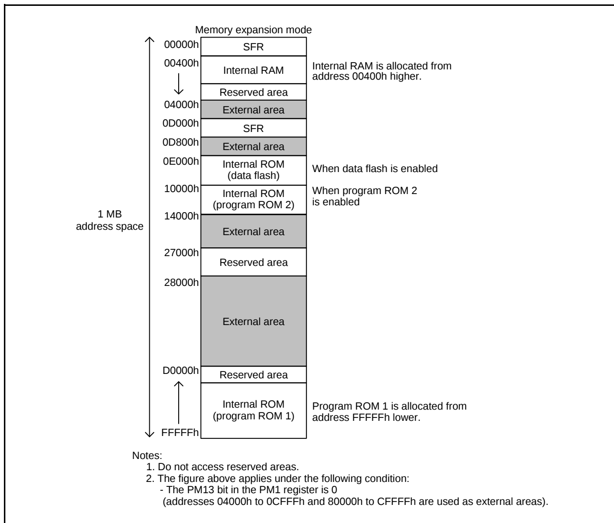
Figure 3.1 Address Space
