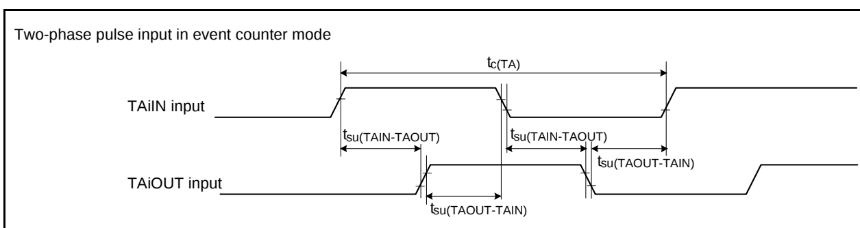
Figure 5.10 Timer A Input (Two-Phase Pulse Input in Event Counter Mode)
