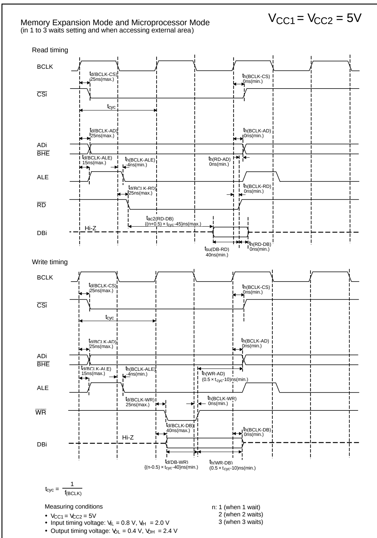
Figure 5.19 Timing Diagram
