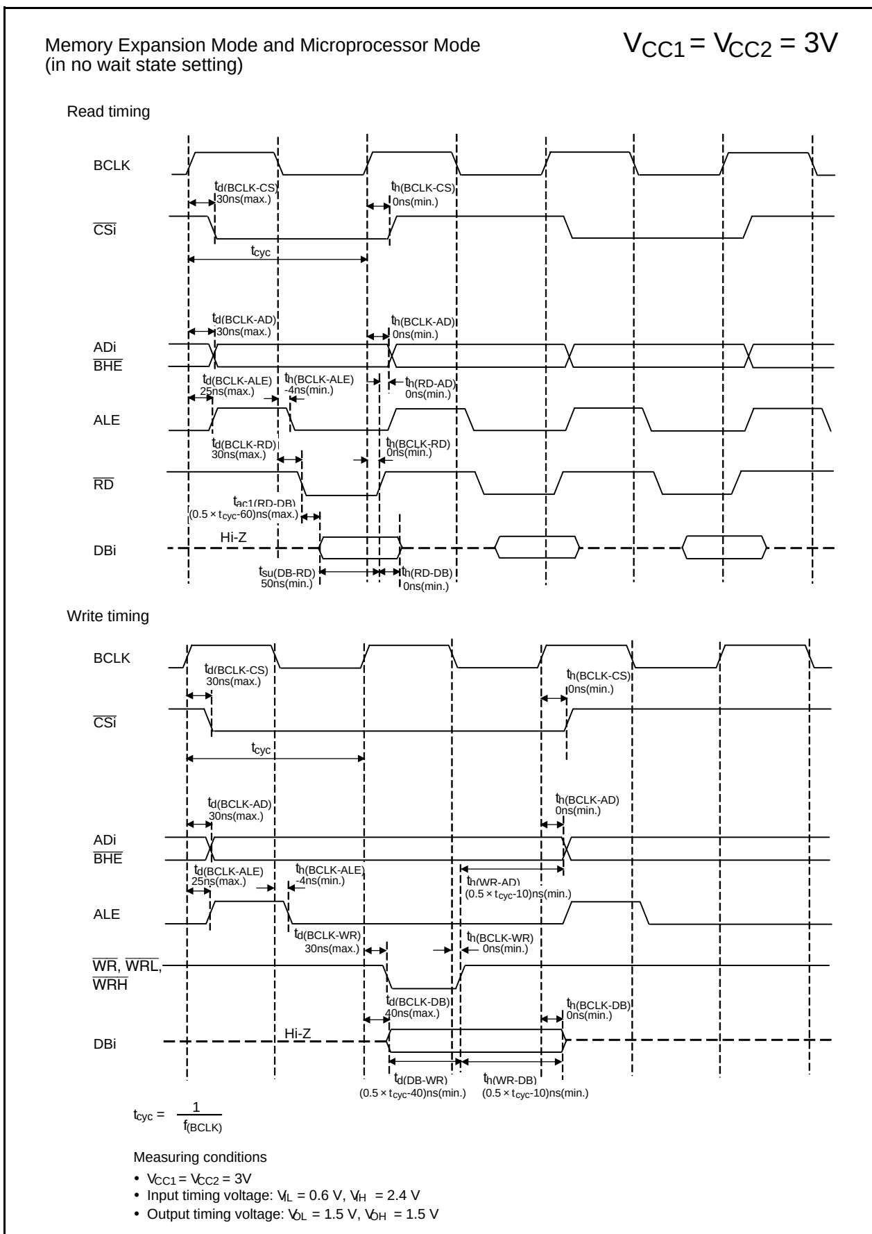
Figure 5.28 Timing Diagram
