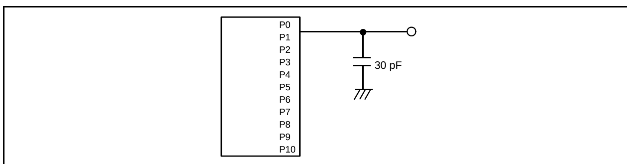
Figure 5.14 Ports P0 to P10 Measurement Circuit
