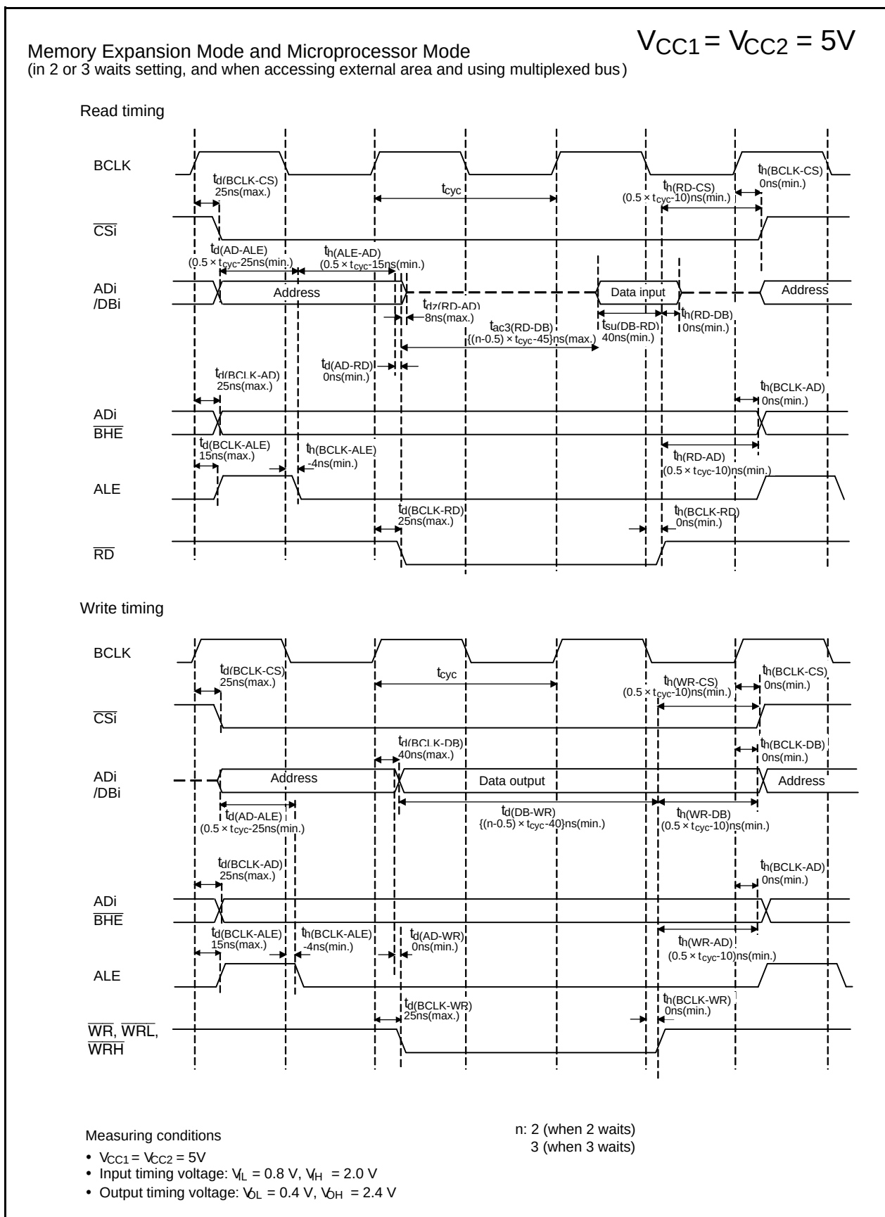
Figure 5.17 Timing Diagram
