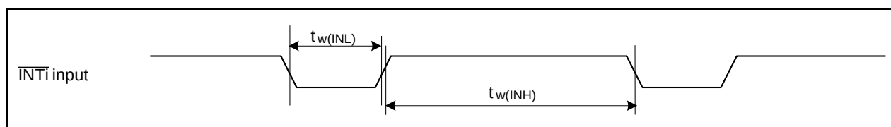
Figure 5.24 External Interrupt \overline{\text{INTi}} Input
