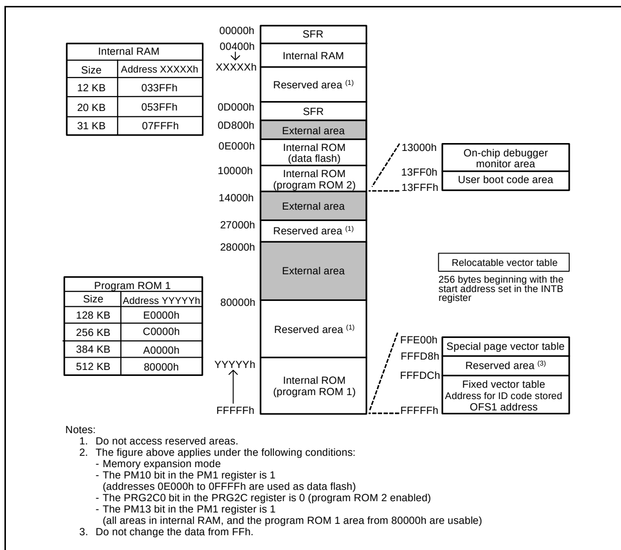
Figure 3.2 Memory Map
