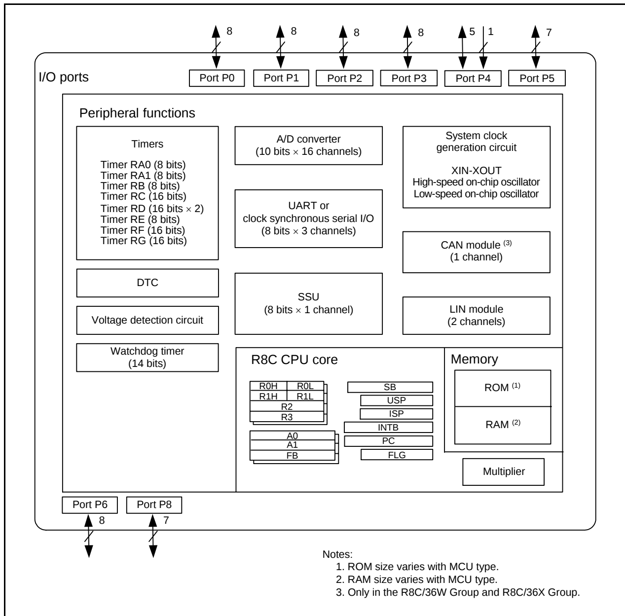
Figure 1.5 Block Diagram
