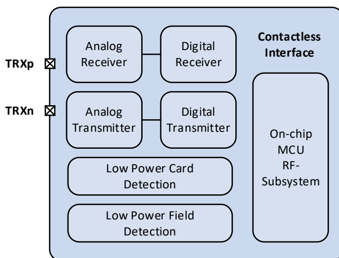
Figure 6: Contactless Interface
