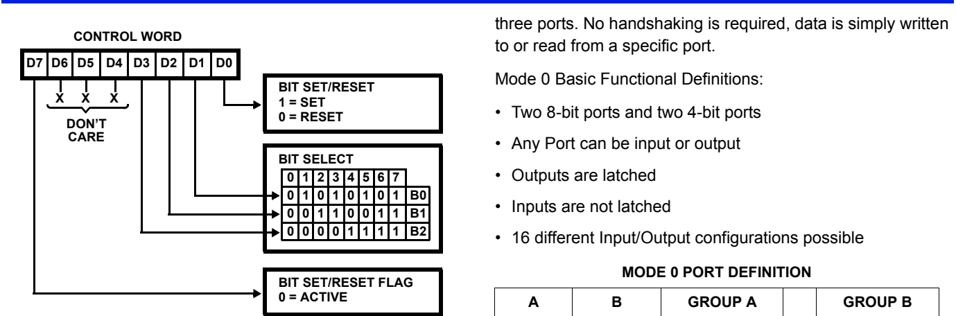
FIGURE 5. BIT SET/RESET FORMAT
