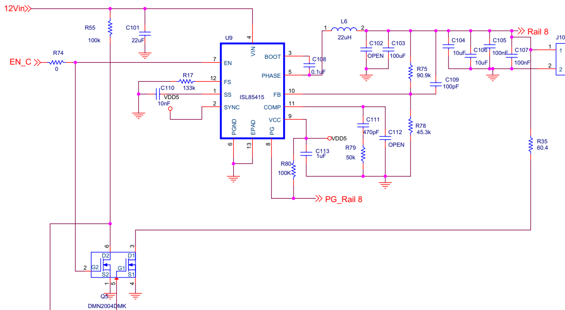
Figure 11. Schematic 8
