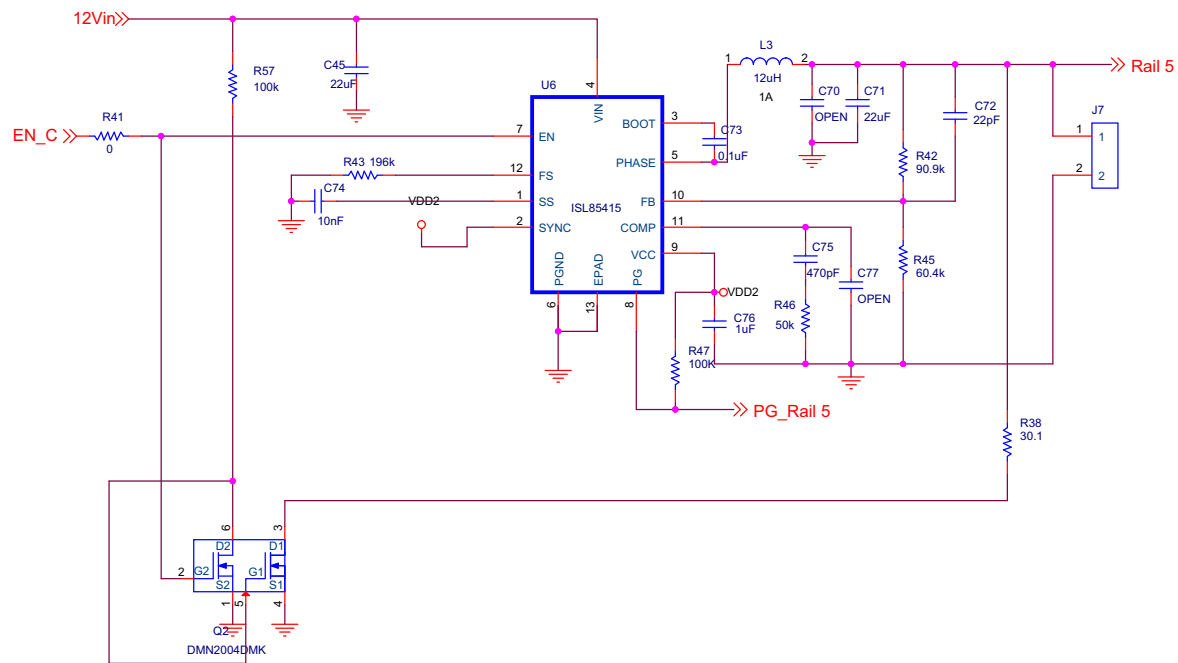
Figure 8. Schematic 5
