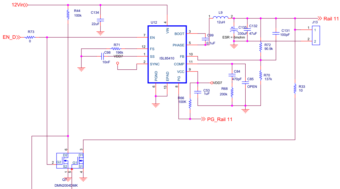
Figure 14. Schematic 11
