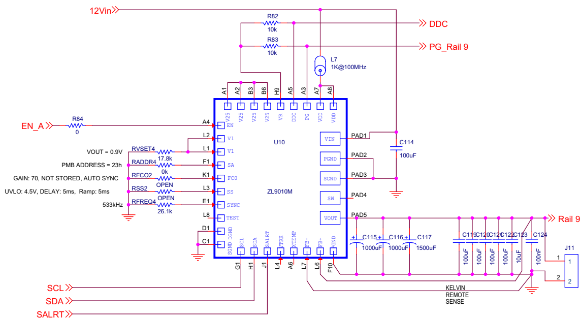
Figure 12. Schematic 9
