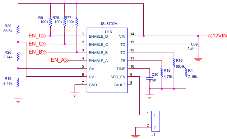
Figure 15. Schematic 12
