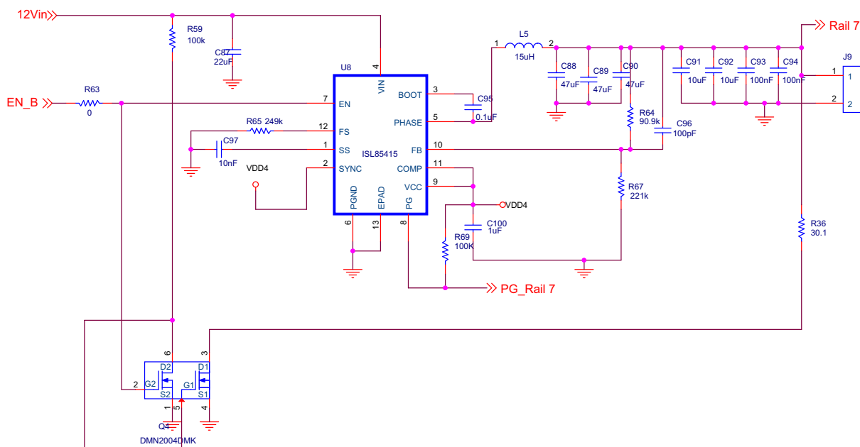
Figure 10. Schematic 7
