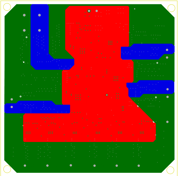
Figure 19. Layer 3
