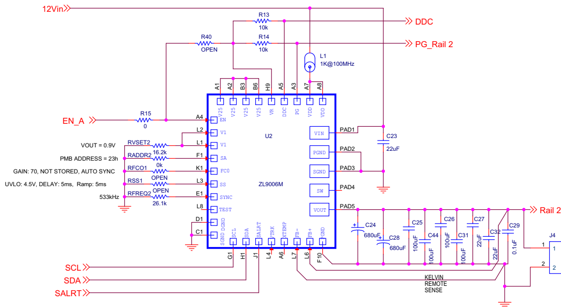
Figure 5. Schematic 2
