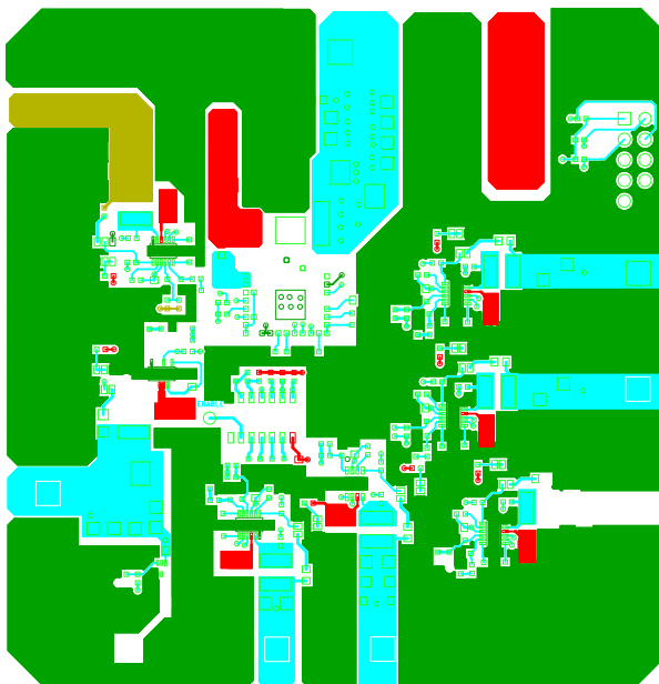
Figure 15. Top Layer
