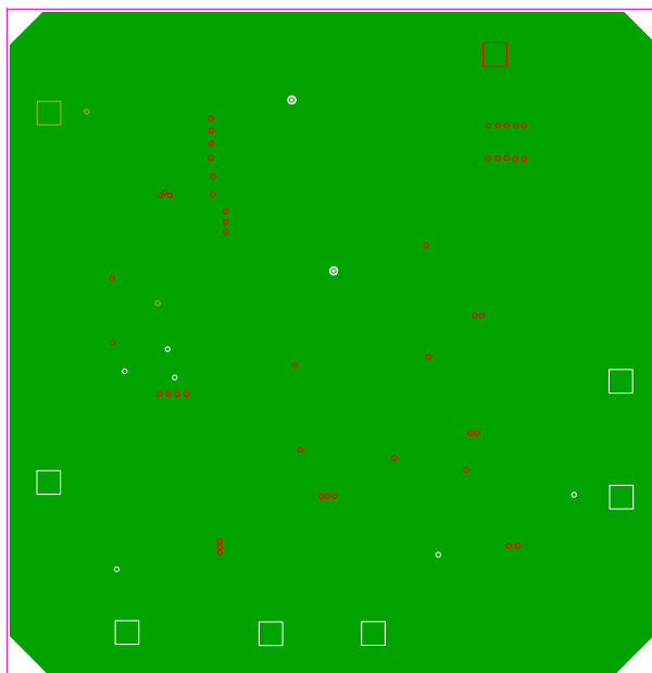
Figure 16. Layer 2
