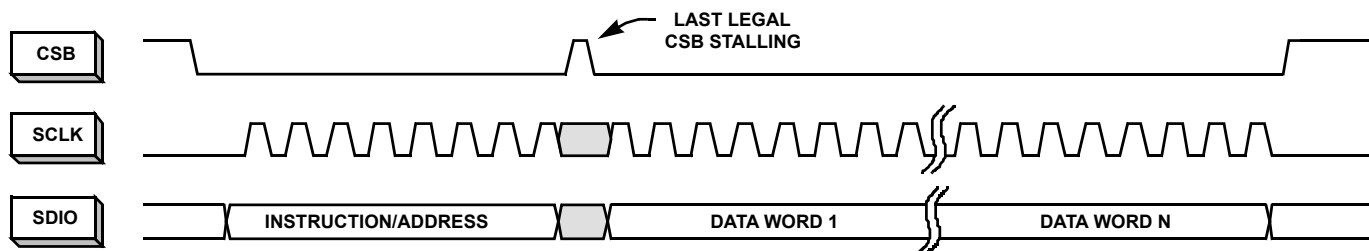
FIGURE 43. N-BYTE TRANSFER
