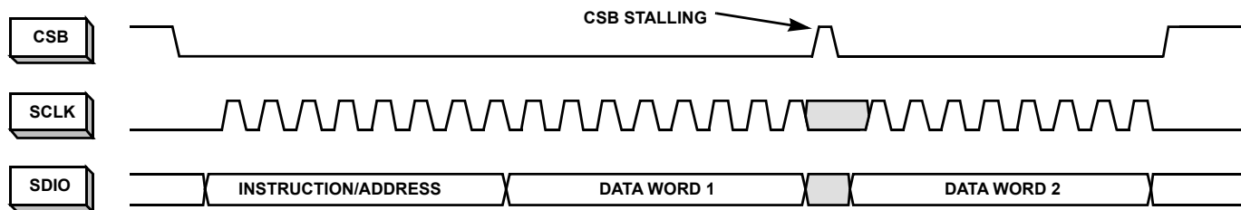
FIGURE 42. 2-BYTE TRANSFER
