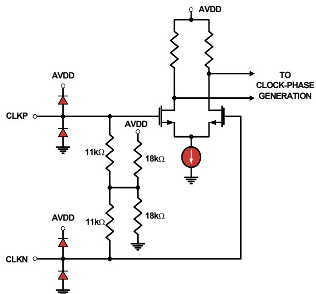
FIGURE 46. CLOCK INPUTS
