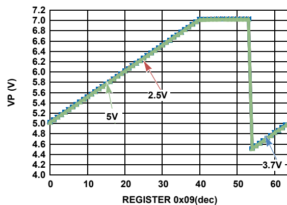
FIGURE 5. V_P OUTPUT VOLTAGE RANGE
