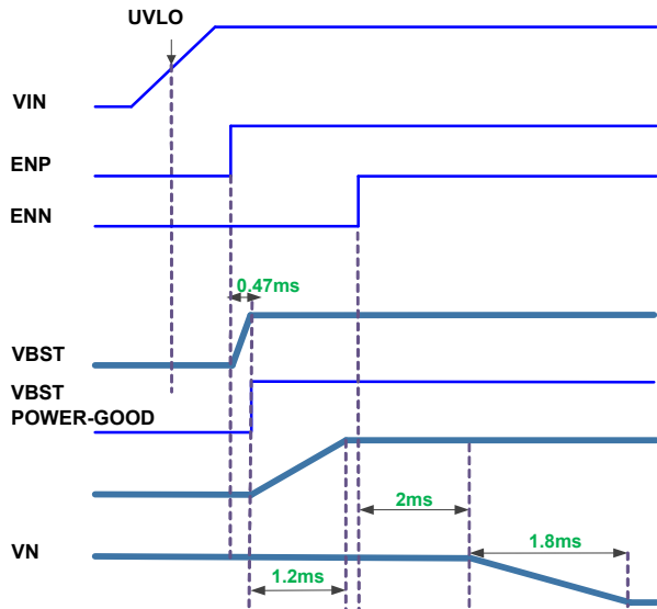
FIGURE 52. POWER-ON SEQUENCE - ACTIVATED BY TWO GPIOs FOR ENN AND ENP, REGISTER 0x04 <b 4 > = 0 AND 0x05 <b 7 > = 0
