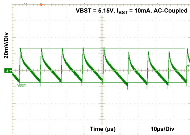
Figure 5. VBST Output Voltage Ripple with 10mA Load
