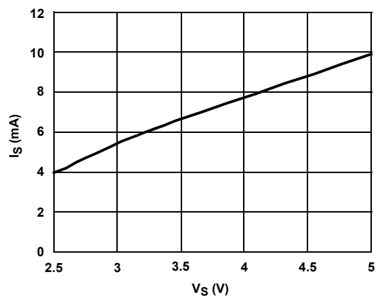
FIGURE 6. NO LOAD QUIESCENT CURRENT
