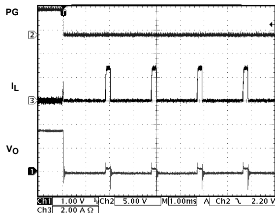
FIGURE 12. OVERCURRENT HICCUP MODE
