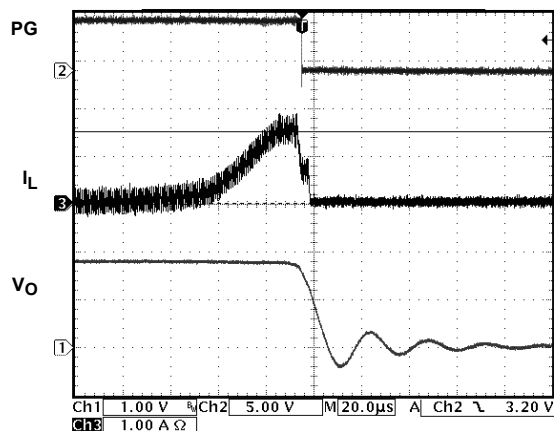
FIGURE 11. OVERCURRENT SHUTDOWN
