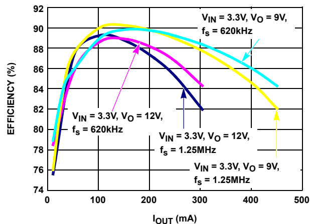
FIGURE 3. BOOST EFFICIENCY vs I_{OUT}
