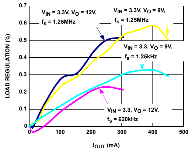
FIGURE 5. LOAD REGULATION vs I_{OUT}
