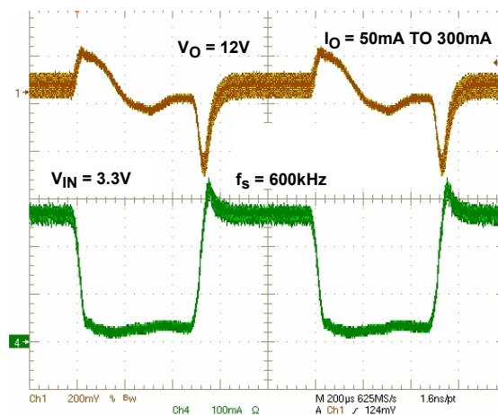
FIGURE 7. TRANSIENT RESPONSE
