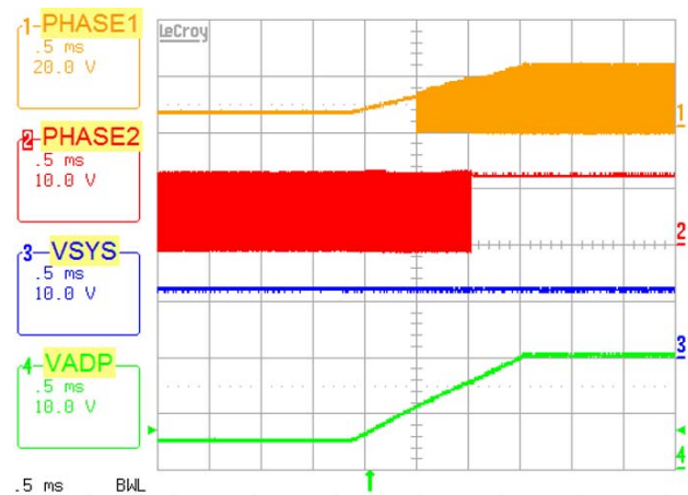
Figure 14. ADP Voltage Ramps Up in Reverse Mode, Buck -&gt; Buck-Boost -&gt; Boost Operation Mode Transition
