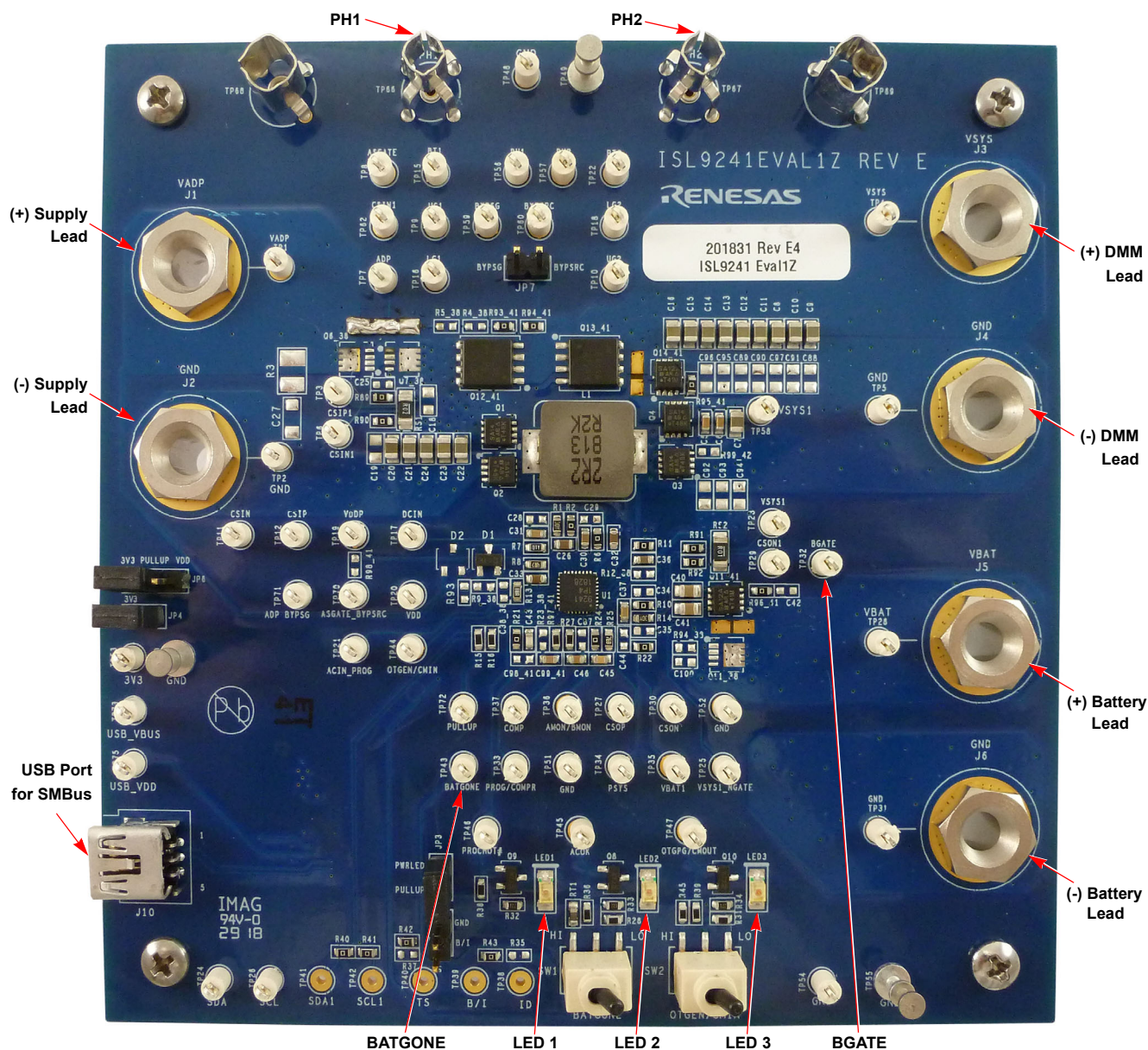
Figure 7. ISL9241EVAL1Z Connections
