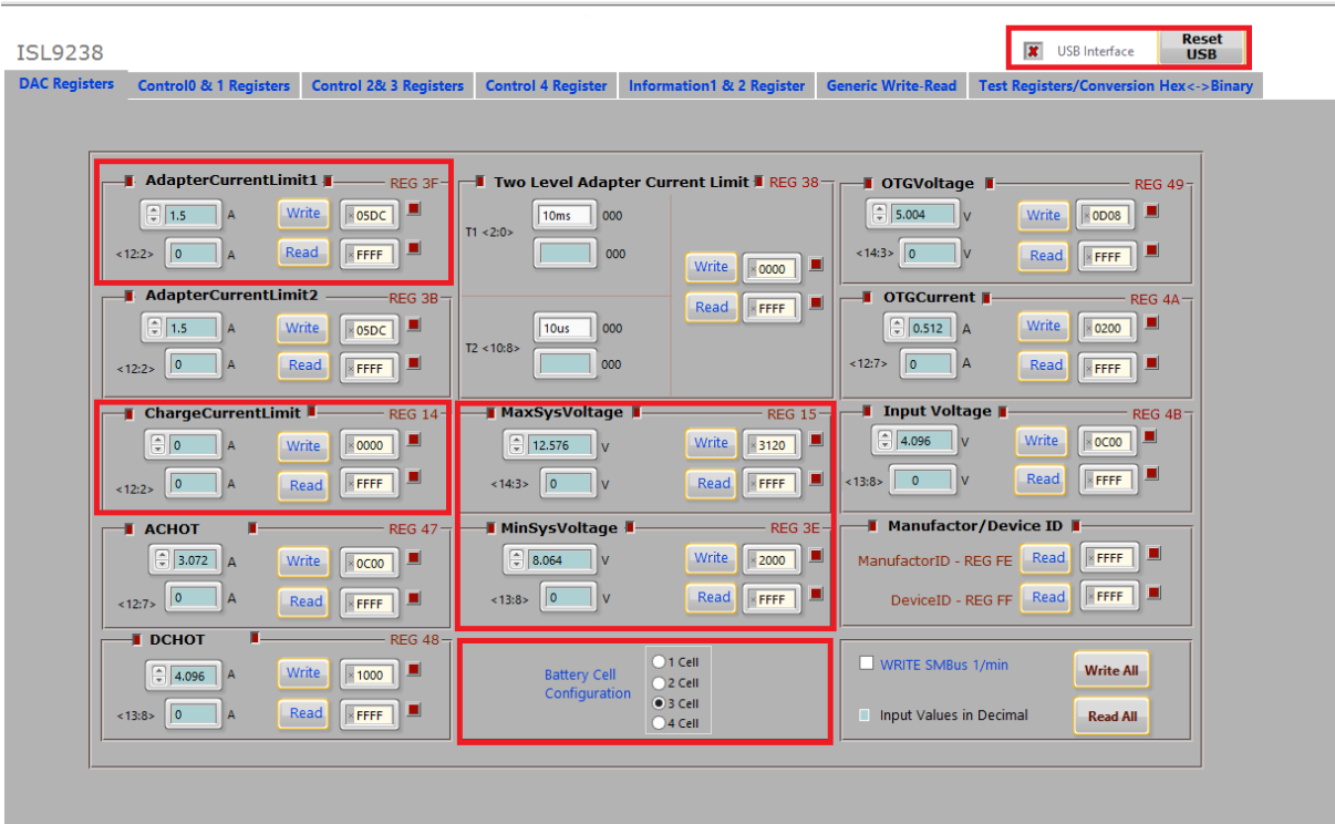
FIGURE 2. GUI SNAPSHOT
