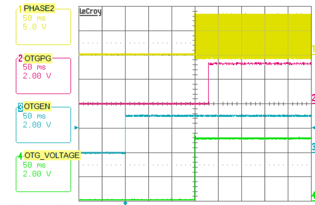
FIGURE 21. OTG MODE ENABLE, OTG ENABLE 150ms DEBOUNCE TIME
