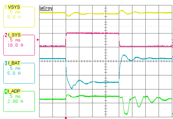
FIGURE 14. BOOST MODE, CHARGING CURRENT LOOP TO ADAPTER CURRENT LOOP TRANSITION. V_{ADP} = 5V , MAXSYSTEMVOLTAGE = 8.496V , V_{BAT} = 7V , SYSTEM LOAD 0.5A TO 10A STEP, ADAPTERCURRENTLIMIT = 3A , CHARGECURRENT = 1A
