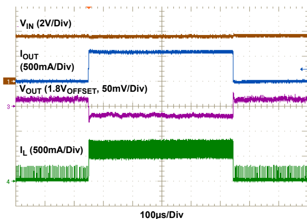
Figure 20. Load Transient: V_{IN} = 3.6V , V_{OUT} = 1.8V , Load = 0.01A to 0.60A, Slew Rate = 1A/ \mu s , Type I Error Amplifier
