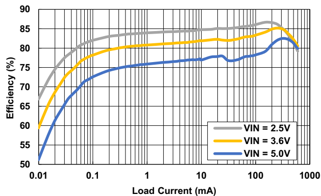
Figure 4. Efficiency vs Load Current: V_{OUT} = 0.8V
