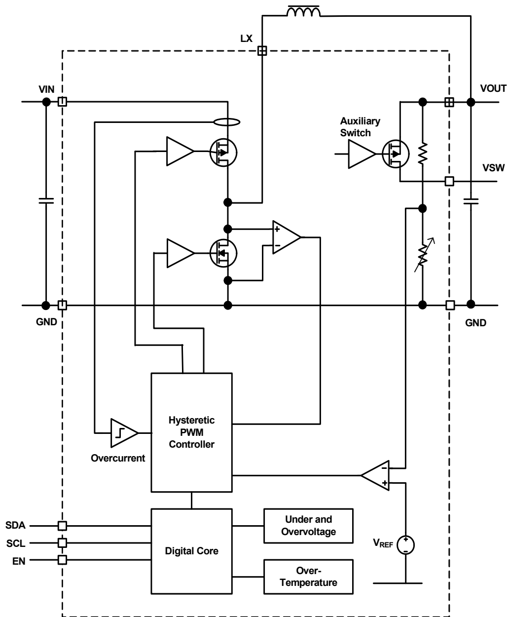
Figure 3. Block Diagram
