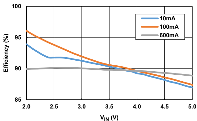
Figure 6. Efficiency vs Input Voltage: V_{OUT} = 1.8V
