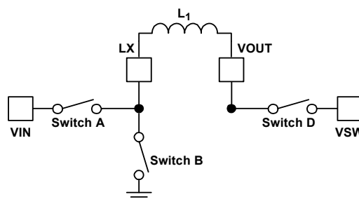
Figure 25. Buck Topology
