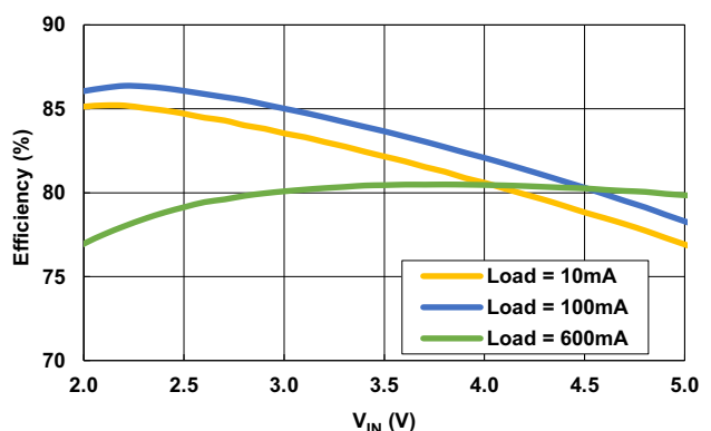
Figure 7. Efficiency vs Input Voltage: V_{OUT} = 0.8V
