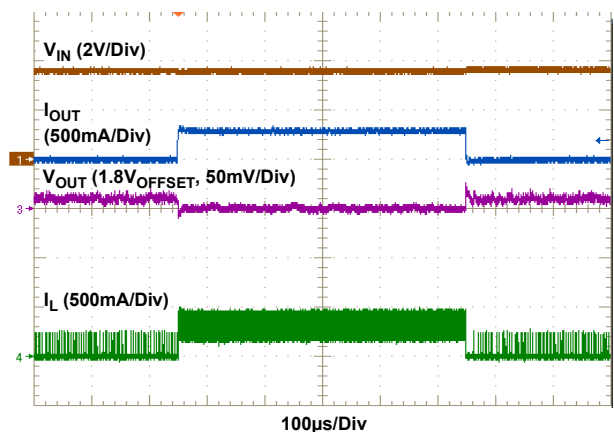
Figure 21. Load Transient: V_{IN} = 3.6V , V_{OUT} = 1.8V , Load = 0.01A to 0.30A, Slew Rate = 1A/ \mu s , Type II Error Amplifier
