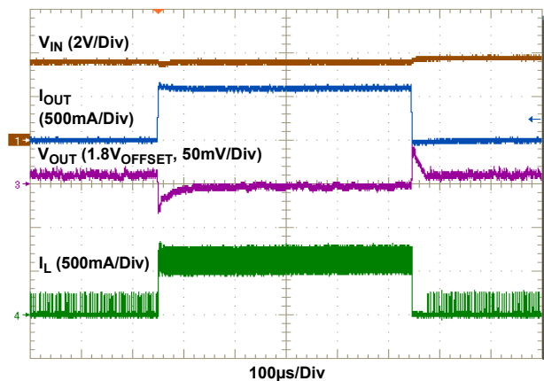
Figure 19. Load Transient: V_{IN} = 3.6V , V_{OUT} = 1.8V , Load = 0.01A to 0.60A, Slew Rate = 1A/ \mu s , Type II Error Amplifier
