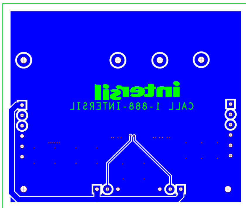
FIGURE 9. BOTTOM LAYER
