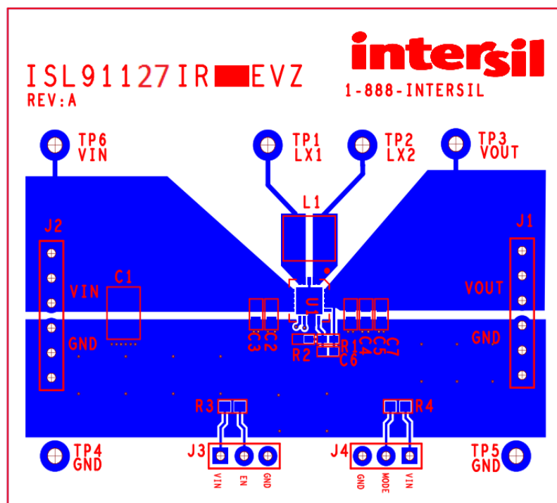
FIGURE 8. TOP LAYER
