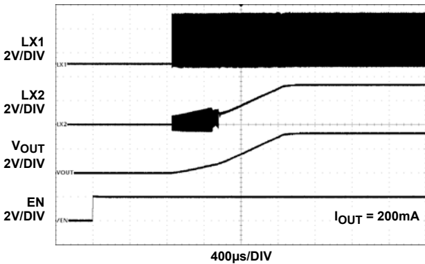
FIGURE 3. ISL91127IR START-UP WITH V_{IN} = 4V AND V_{OUT} = 3.3V
