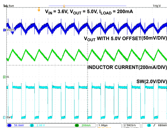
FIGURE 18. PWM WAVEFORM
