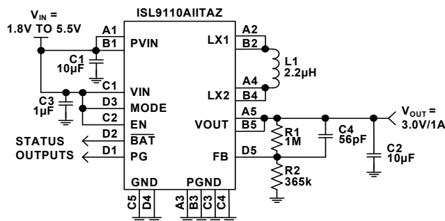
FIGURE 28. TYPICAL ISL9110AIIITAZ APPLICATION
