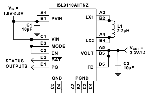
FIGURE 30. TYPICAL ISL9110AIIATNZ APPLICATION
