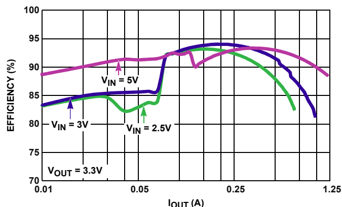
FIGURE 2. EFFICIENCY
