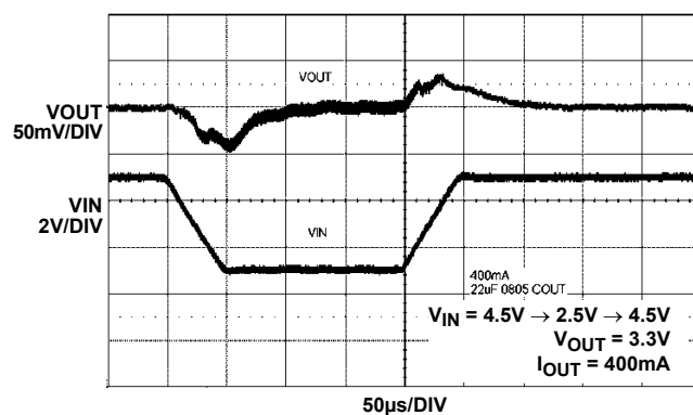
FIGURE 12. INPUT TRANSIENT
