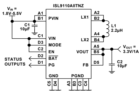
FIGURE 29. TYPICAL ISL9110AIIATAZ APPLICATION
