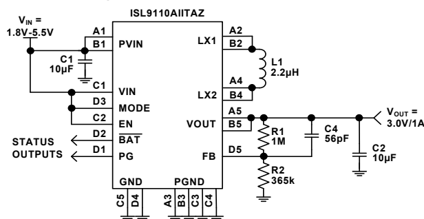
FIGURE 31. TYPICAL ISL9110AIIATAZ APPLICATION
