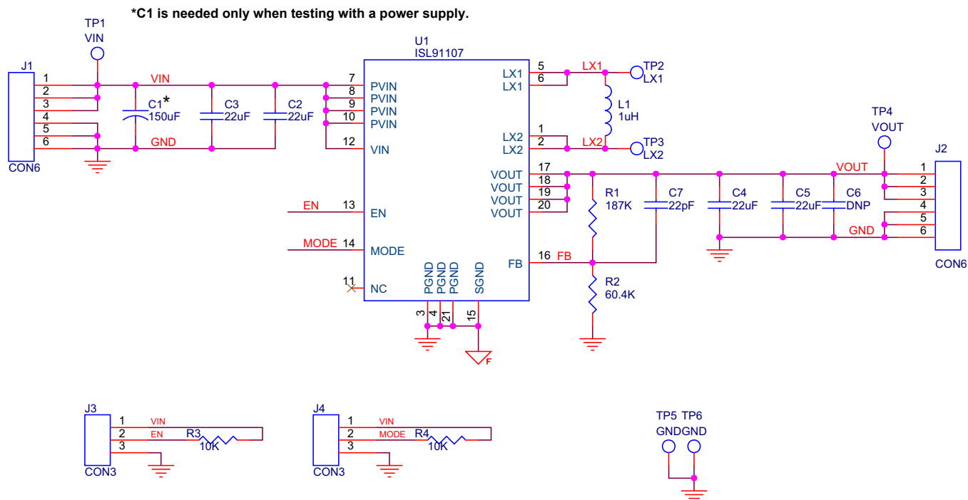
FIGURE 6. ISL91107IRA-EVZ EVALUATION BOARD SCHEMATIC
