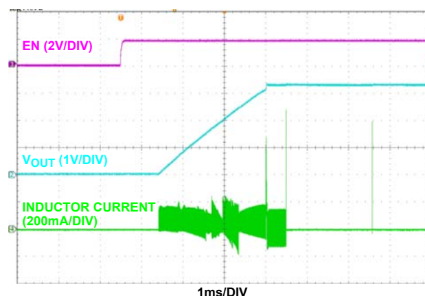
FIGURE 2. ISL91107IR START-UP WITH V_{IN} = 2V AND V_{OUT} = 3.3V
