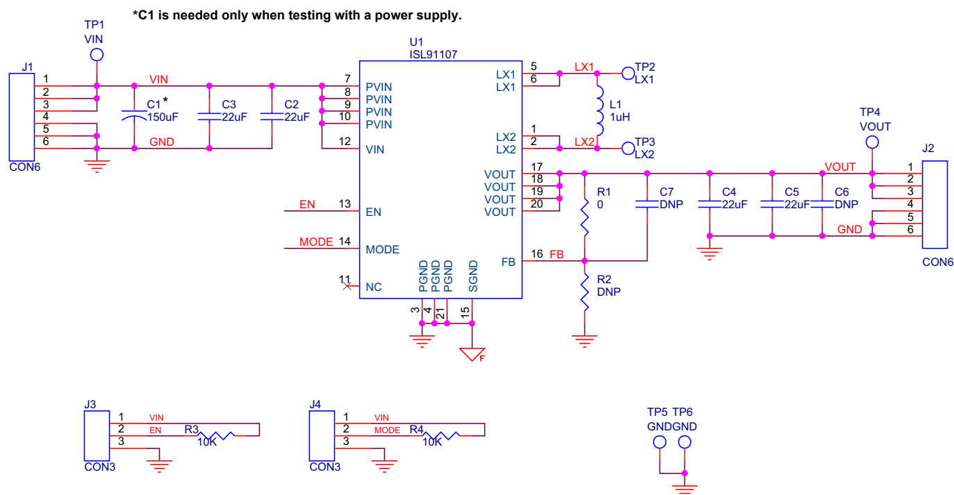
FIGURE 7. ISL91107IRN-EVZ EVALUATION BOARD SCHEMATIC
