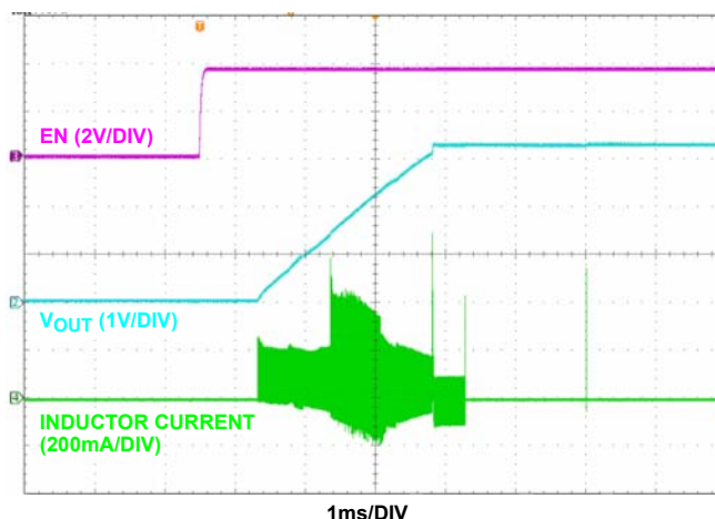
FIGURE 3. ISL91107IR START-UP WITH V_{IN} = 4V AND V_{OUT} = 3.3V
