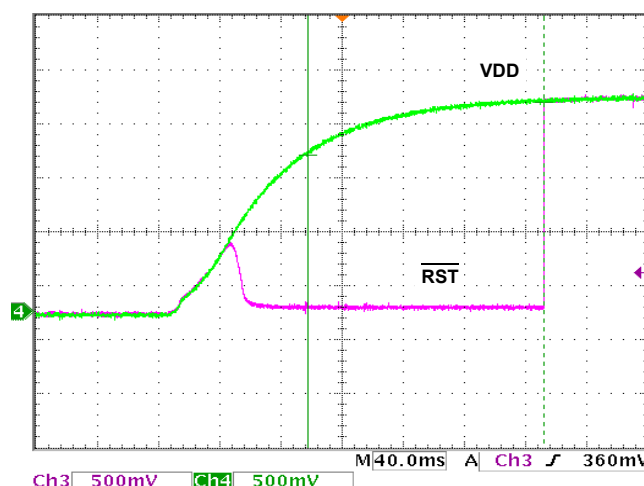
FIGURE 4. ISL88002 \overline{RST} t_{POR} ~155ms, R_{PU} = 5\text{ k}\Omega
