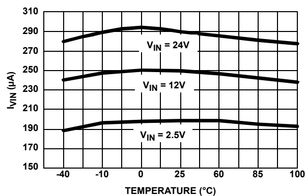
FIGURE 5. V IN CURRENT
