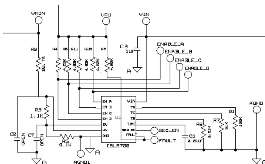
FIGURE 15. ISL870X EVAL1 PHOTOGRAPH AND SCHEMATIC OF LEFT CHANNEL
