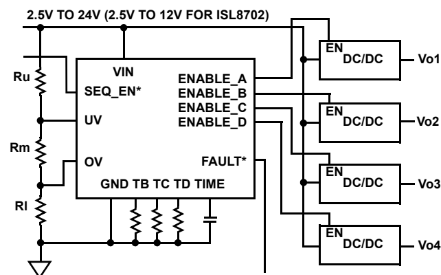
FIGURE 1. ISL870x IMPLEMENTATION
