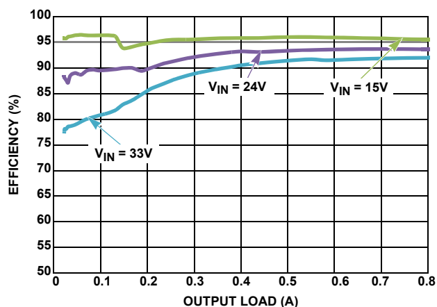
FIGURE 5. EFFICIENCY vs LOAD, PFM, V_{OUT} = 12\text{V}
