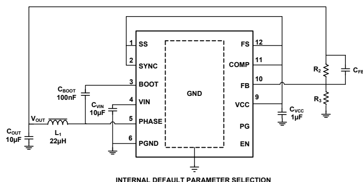
FIGURE 1. TYPICAL APPLICATION
