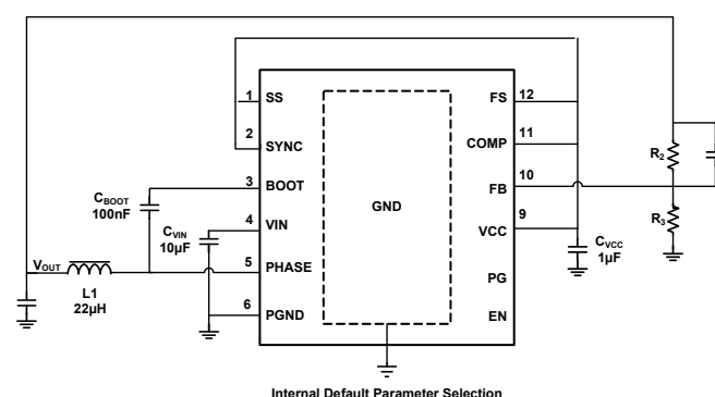
Figure 1. Typical Application
