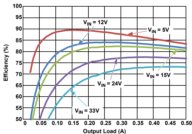
Figure 23. Efficiency vs Load, PWM, V_{OUT} = 1.8\text{V}
