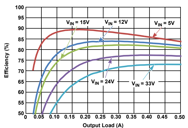
Figure 11. Efficiency vs Load, PWM, V_{OUT} = 1.8\text{V}
