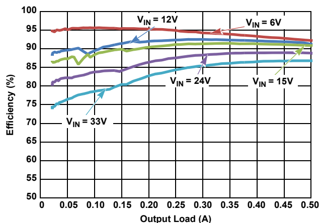
Figure 18. Efficiency vs Load, PFM, V_{OUT} = 5\text{V}
