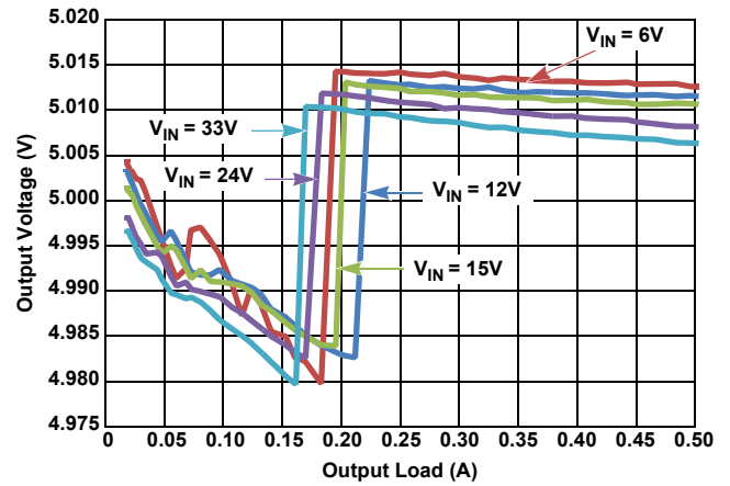
Figure 13. V_{OUT} Regulation vs Load, PFM, V_{OUT} = 5\text{V}
