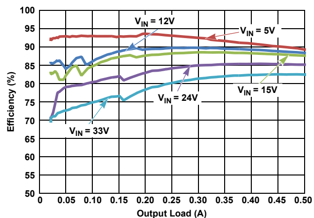
Figure 20. Efficiency vs Load, PFM, V_{OUT} = 3.3\text{V}
