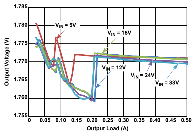
Figure 17. V_{OUT} Regulation vs Load, PFM, V_{OUT} = 1.8\text{V}
