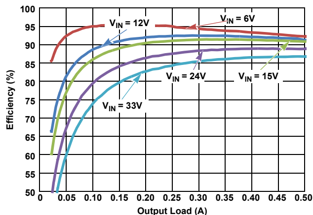
Figure 19. Efficiency vs Load, PWM, V_{OUT} = 5\text{V}
