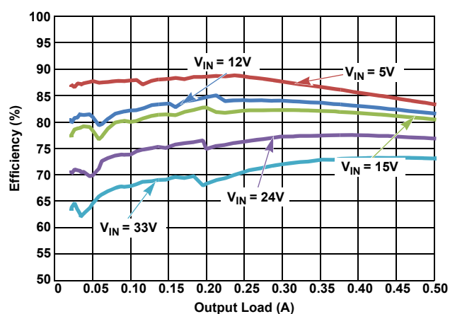
Figure 22. Efficiency vs Load, PFM, V_{OUT} = 1.8\text{V}
