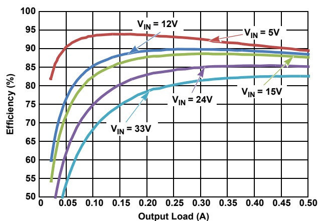
Figure 21. Efficiency vs Load, PWM, V_{OUT} = 3.3\text{V}
