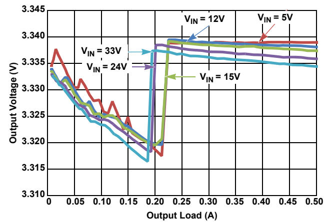
Figure 15. V_{OUT} Regulation vs Load, PFM, V_{OUT} = 3.3\text{V}
