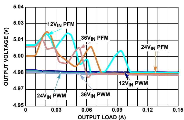
FIGURE 17. V_{OUT} REGULATION vs LOAD, V_{OUT} = 5\text{V}
