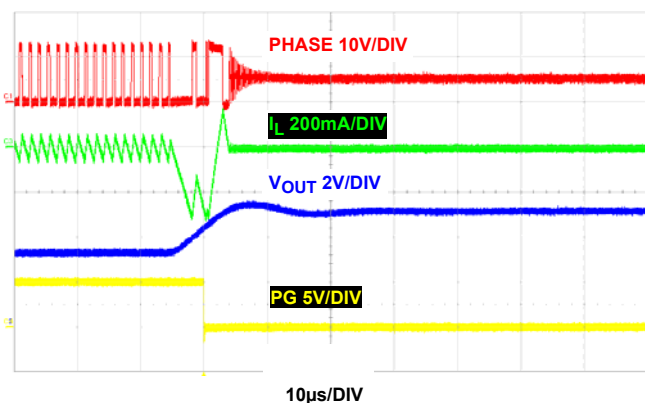
FIGURE 47. OVERVOLTAGE PROTECTION
