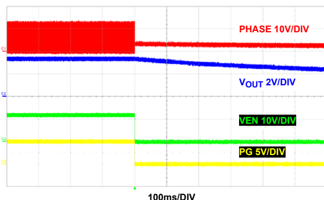
FIGURE 22. SHUTDOWN AT NO LOAD, PWM
