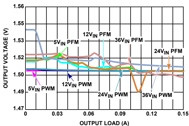
FIGURE 13. V_{OUT} REGULATION vs LOAD, PWM, V_{OUT} = 1.5\text{V}
