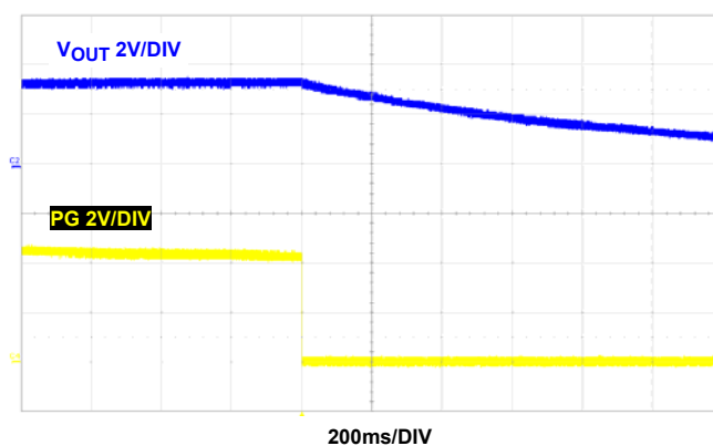
FIGURE 48. OVERTEMPERATURE PROTECTION
