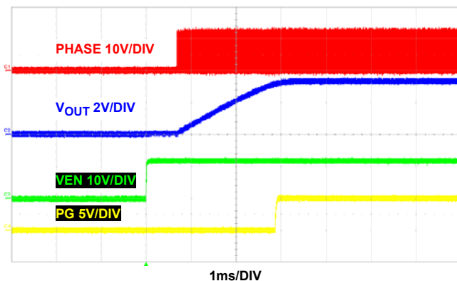
FIGURE 20. START-UP AT NO LOAD, PWM
