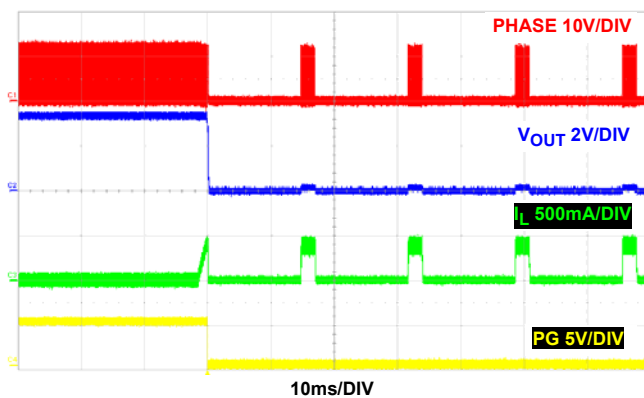
FIGURE 44. OVERCURRENT PROTECTION
