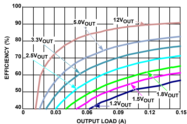
FIGURE 10. EFFICIENCY vs LOAD, PWM, V_{IN} = 36\text{V}
