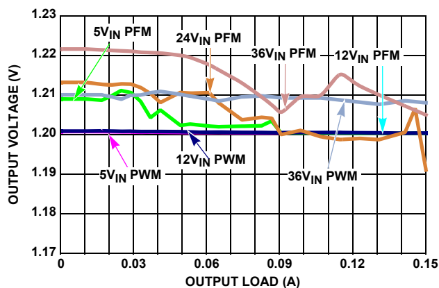
FIGURE 12. V_{OUT} REGULATION vs LOAD, V_{OUT} = 1.2\text{V}
