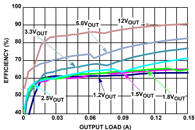
FIGURE 9. EFFICIENCY vs LOAD, PFM, V_{IN} = 36\text{V}
