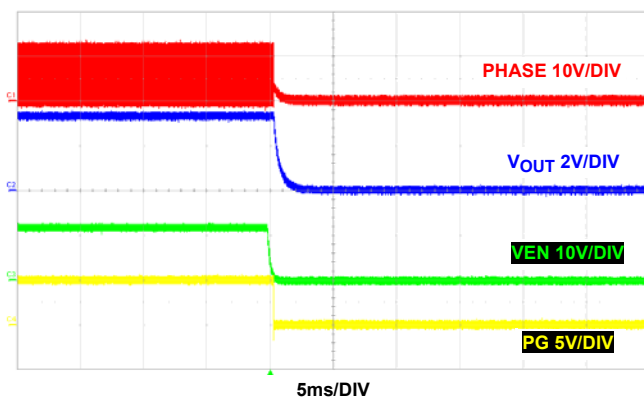
FIGURE 26. SHUTDOWN AT 150mA, PFM
