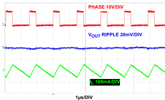
FIGURE 38. STEADY STATE AT NO LOAD, PWM
