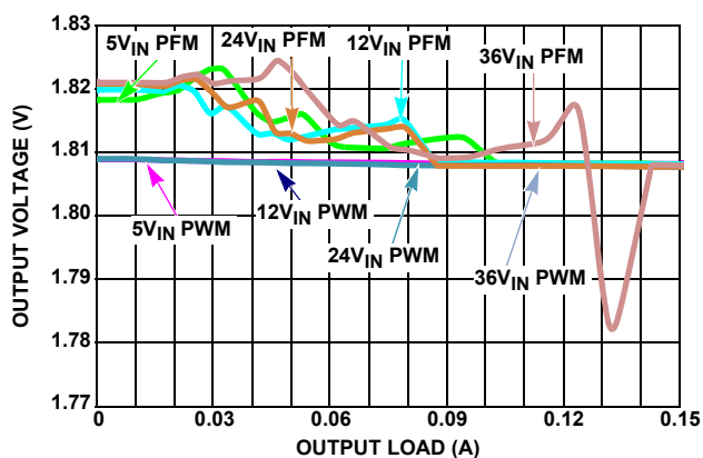
FIGURE 14. V_{OUT} REGULATION vs LOAD, V_{OUT} = 1.8\text{V}
