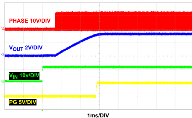
FIGURE 32. START-UP V_{IN} AT NO LOAD, PWM
