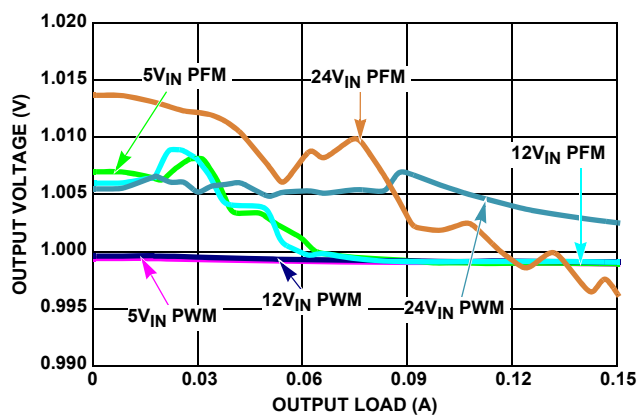
FIGURE 11. V_{OUT} REGULATION vs LOAD, V_{OUT} = 1\text{V}
