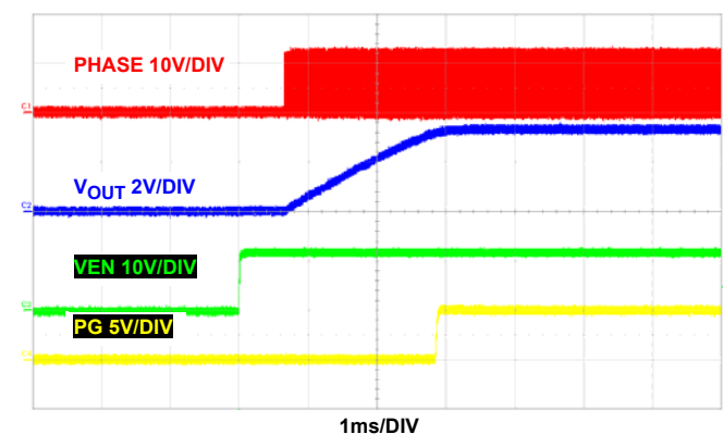
FIGURE 23. START-UP AT 150mA, PWM
