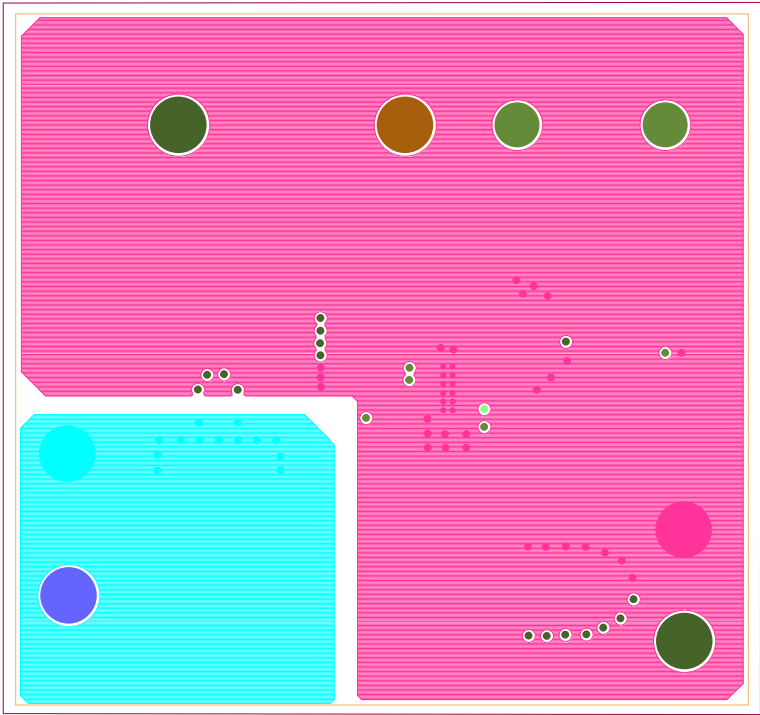
Figure 7. Layer 2
