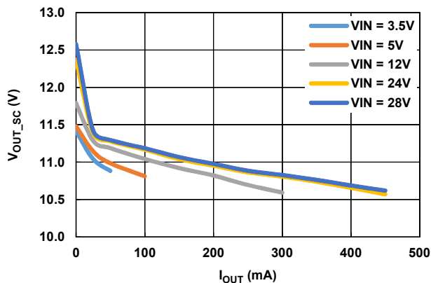
Figure 15. V_{OUT\_SC} Regulation vs I_{OUT} ( V_{OUT} = 12V )
