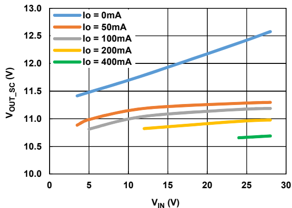
Figure 16. V_{OUT\_SC} Regulation vs V_{IN} ( V_{OUT} = 12V )
