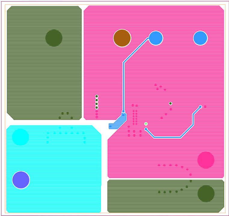
Figure 9. Layer 4
