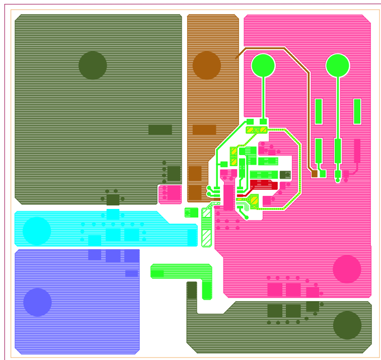
Figure 6. Layer 1
