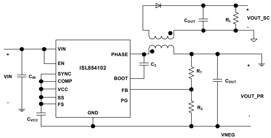
Figure 1. Block Diagram
