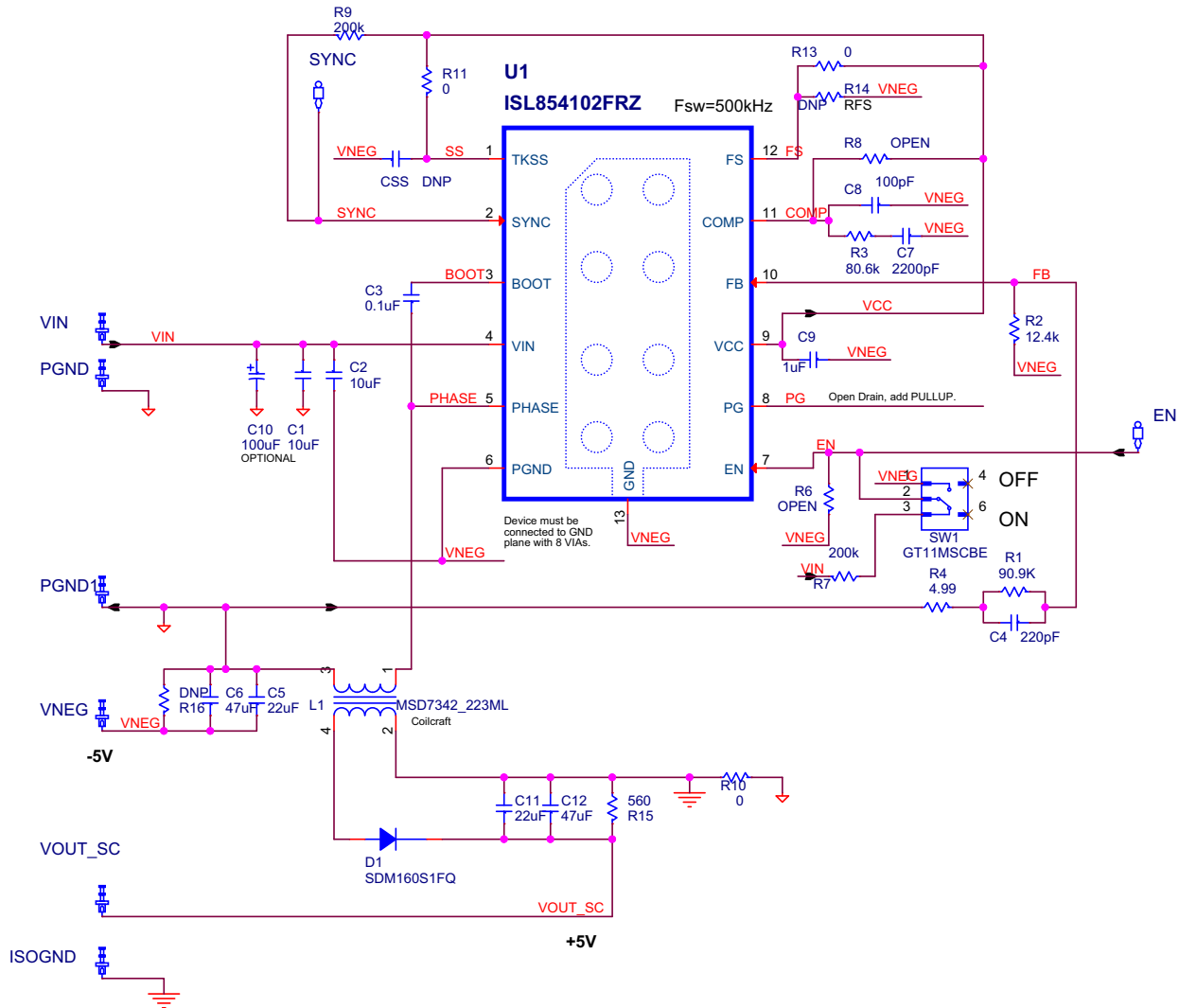
Figure 4. Schematic
