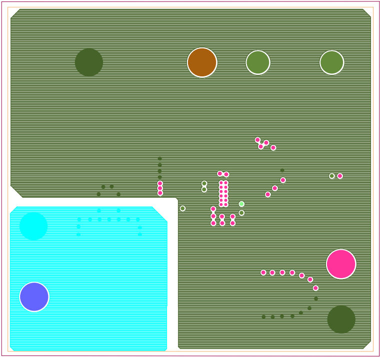
Figure 8. Layer 3
