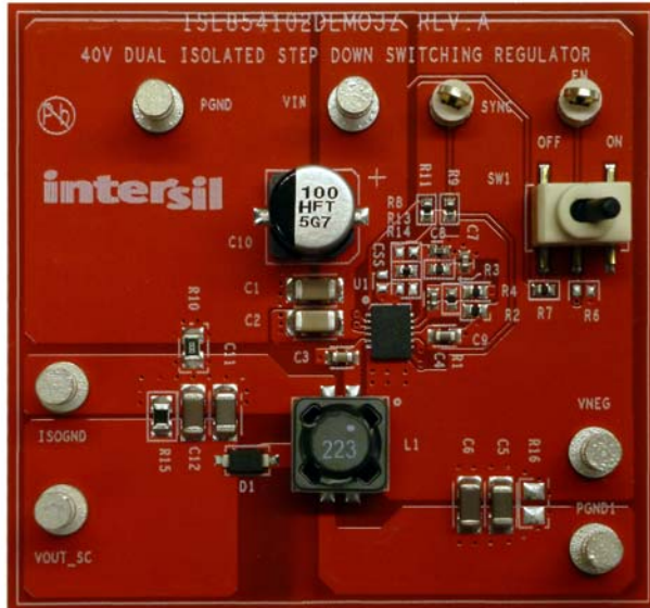
Figure 2. ISL854102DEMO3Z Top
