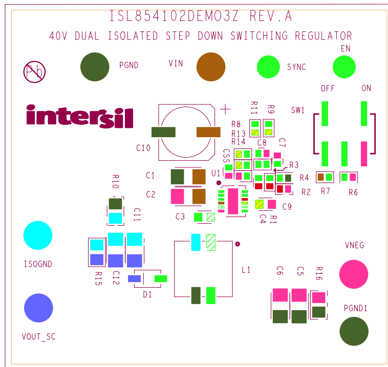
Figure 5. Silkscreen Top
