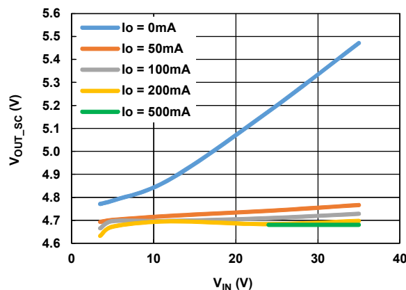
Figure 14. V_{OUT\_SC} Regulation vs V_{IN} ( V_{OUT} = 5V )
