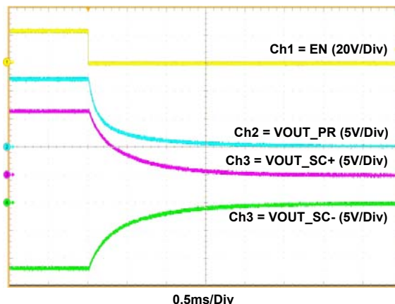
Figure 16. Shutdown by Enable ( V_{IN} = 24V , V_{OUT\_PR} = +12V , V_{OUT\_SC\pm} = \pm 12V , I_{OUT\_PR} = 0.8A , I_{OUT\_SC\pm} = 150mA , FCCM)
