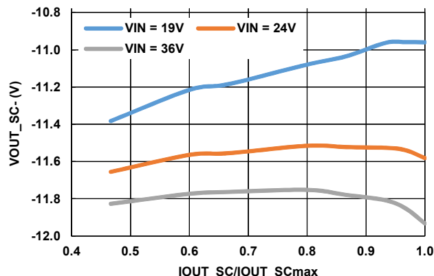
Figure 12. VOUT_SC- Regulation vs IOUT_SC/IOUT_SCmax ( V_{OUT} = \pm 12V )
