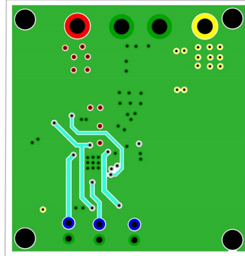
FIGURE 19. LAYER 3
