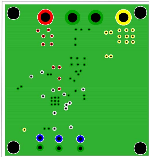
FIGURE 18. LAYER 2
