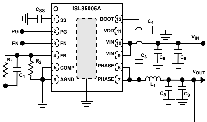
FIGURE 1B. ISL85005AEVAL1Z
