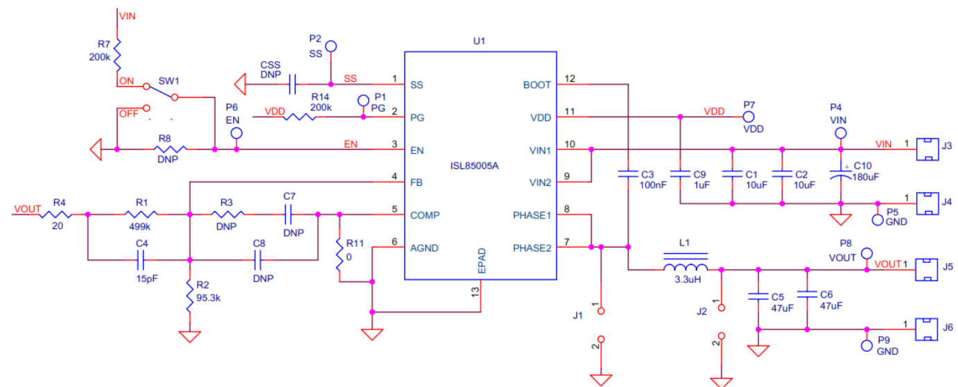
FIGURE 5. ISL85005AEVAL1Z SCHEMATIC
