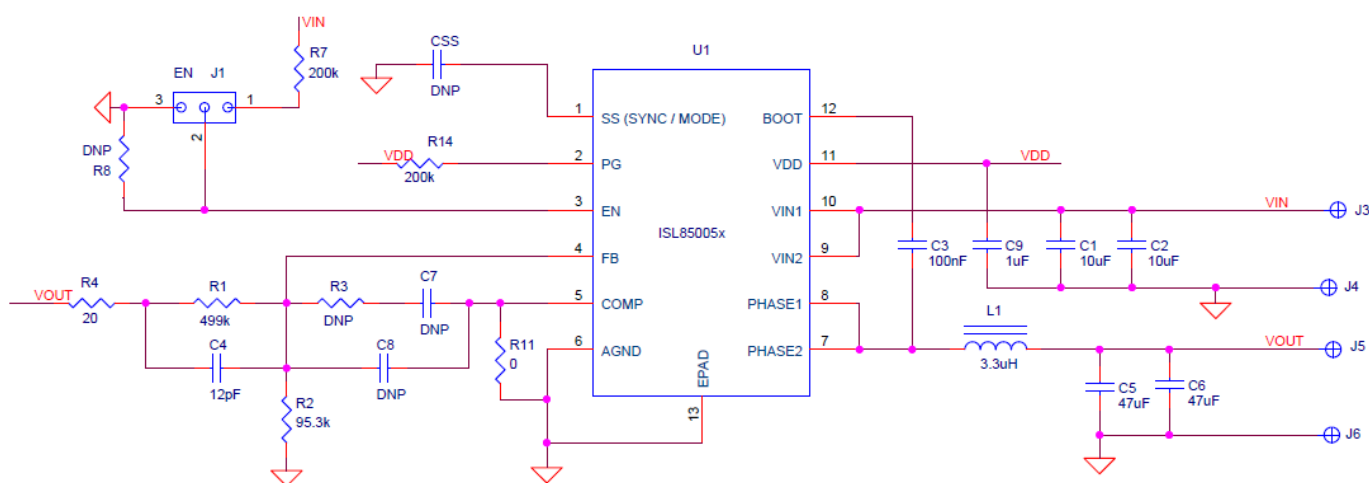
FIGURE 3. ISL85005xDEMO1Z SCHEMATIC
