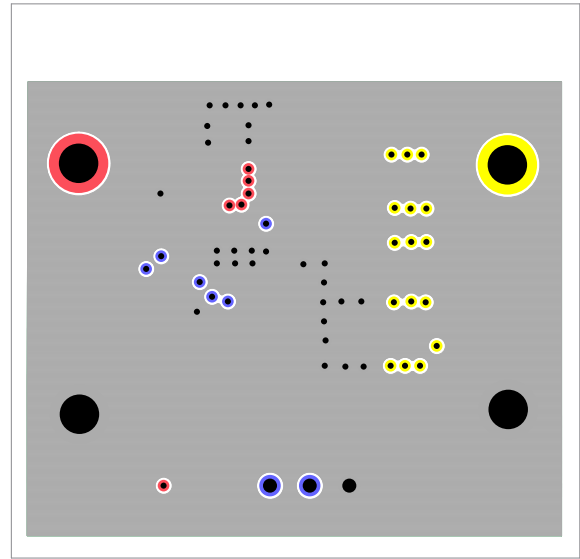
FIGURE 5. LAYER 2
