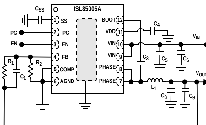
FIGURE 1B. ISL85005ADEMO1Z
